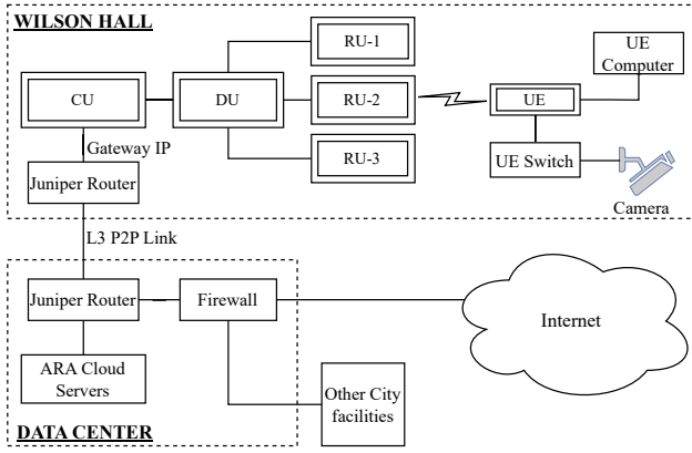
Figure 4: Skylark Deployment Architecture
