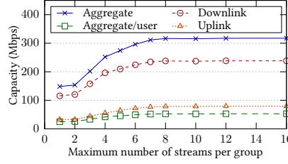
Figure 13: Impact of Maximum Number of Streams on System Capacity
