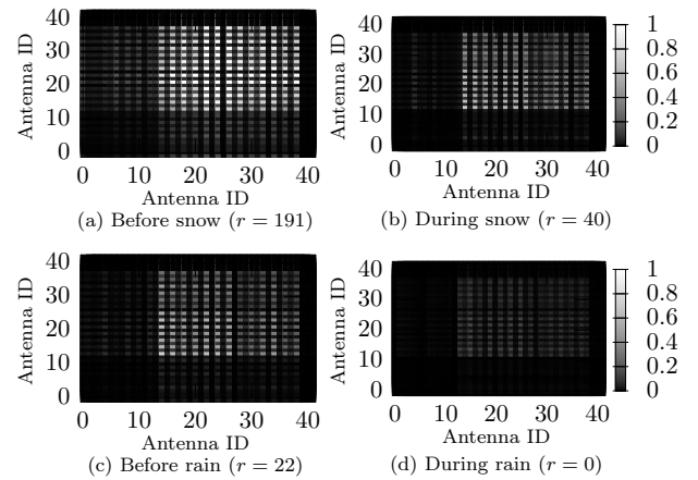
Figure 8: Impact of Snow and Rain on Low-UHF mMIMO Channel Correlation
