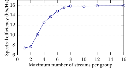
Figure 14: Impact of Increasing Spatial Streams on Spectral Efficiency
