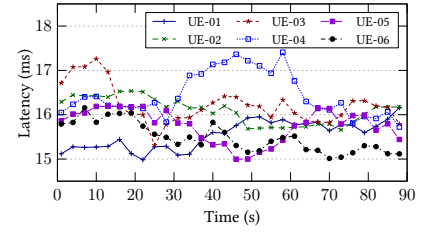
Figure 11: Latency from BS to UEs
