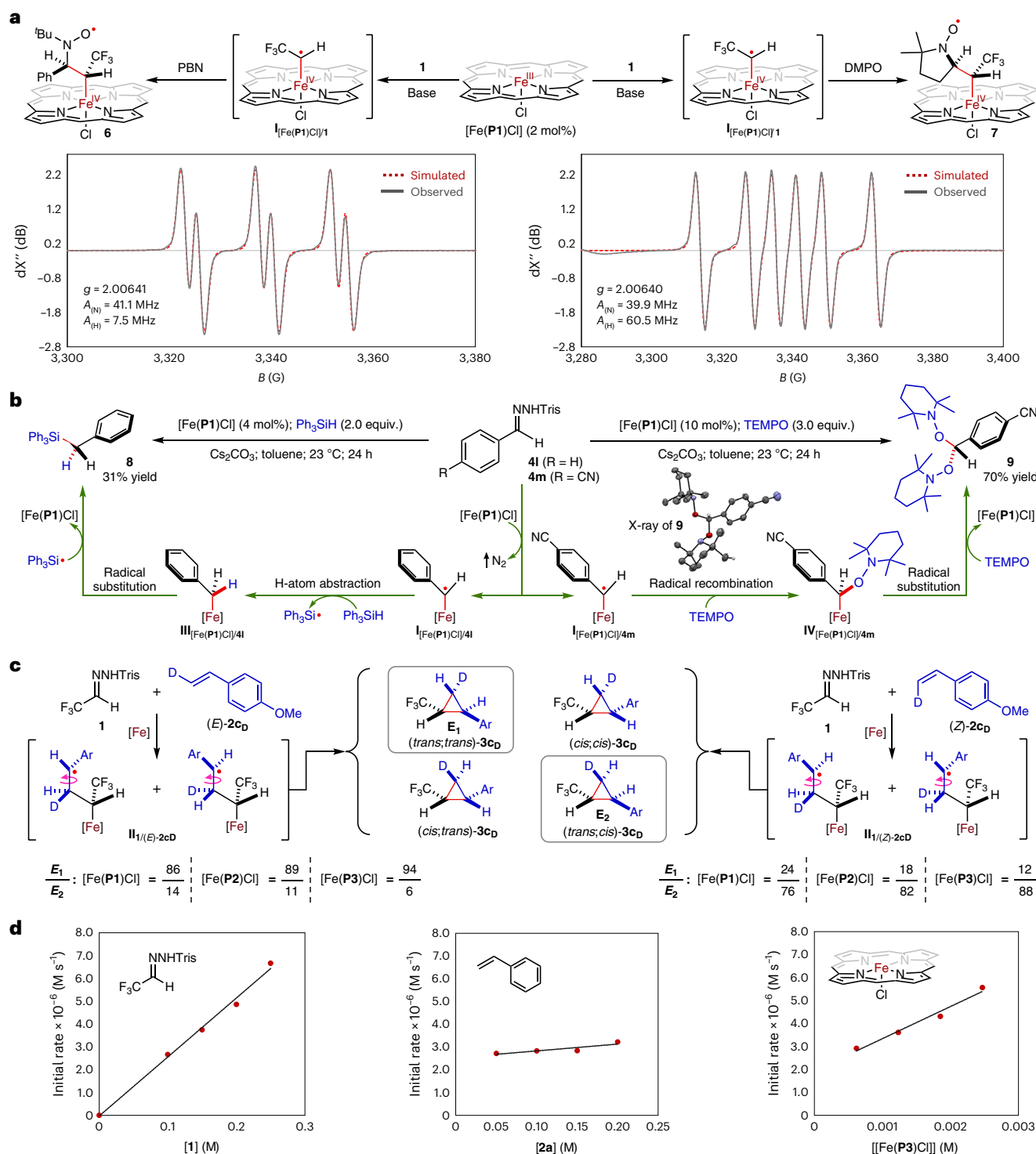
Fig. 5 | Experimental studies on the catalytic mechanism of olefin cyclopropanation by the Fe(III)-based metalloradical system. a , Trapping of the \alpha -Fe(IV)-alkyl radical intermediate by spin traps PBN and DMPO for EPR detection. b , Trapping of \alpha -Fe(IV)-benzyl radicals from metalloradical activation
