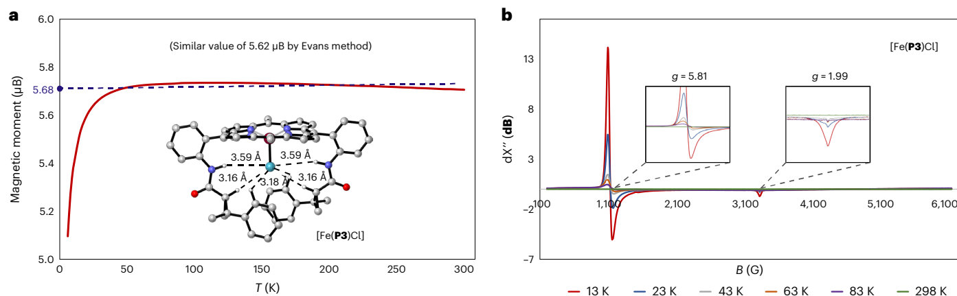
Fig. 4 | Determination of iron spin states in [Fe(P3)Cl]. a , Measurement of the magnetic moment of [Fe(P3)Cl] by variable-temperature SQUID and Evans methods. b , X-band EPR measurement for [Fe(P3)Cl] at different temperatures.
