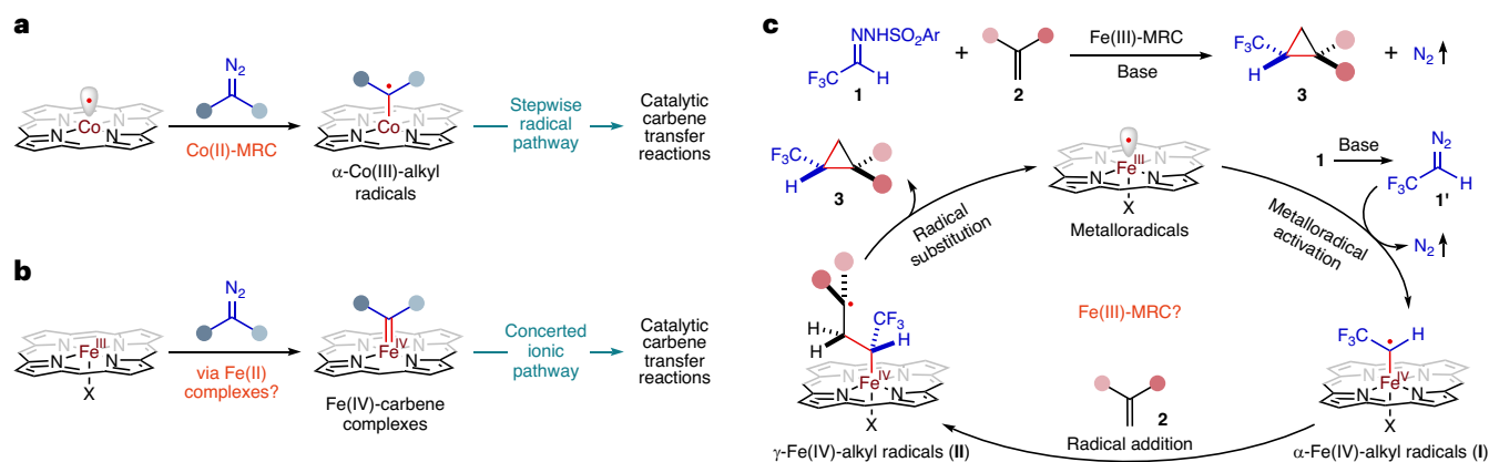
Fig. 1 | Proposed stepwise radical mechanism for cyclopropanation of alkenes with in situ-generated \alpha -trifluoromethyldiazomethane via Fe(III)-based metalloradical catalysis. a , Co(II)-based metalloradical catalysis has emerged as a general catalytic approach for controlling the reactivity and selectivity of homolytic radical reactions. As stable 15e-metalloradicals, cobalt(II) complexes of porphyrins have been demonstrated with the capability of activating diazo compounds to generate \alpha -Co(III)-alkyl radicals that can function as kinetically competent intermediates for catalytic carbene transfer reactions through a stepwise radical pathway. b , Iron(III) complexes of porphyrins have not been unambiguously established as genuine catalysts for catalytic transformations. They have been commonly assumed to be in situ-reduced to Fe(II) complexes as
