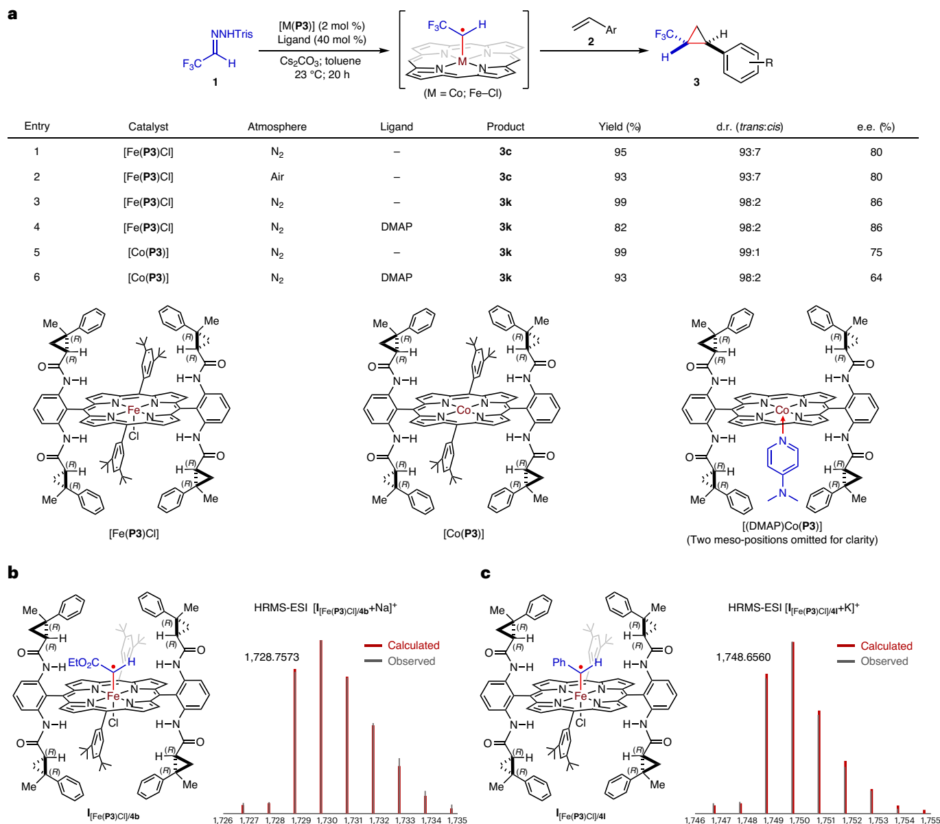
Fig. 2 | Comparative studies on catalytic cyclopropanation and detection of intermediates by HRMS to probe the oxidation state of iron porphyrin catalysts. a , To probe the oxidation state of the active iron catalyst, comparative studies on catalytic cyclopropanation of alkenes 2 with in situ-generated \alpha -trifluoromethyldiazomethane ( 1' ) by [Fe(P3)Cl] were performed under a nitrogen atmosphere and in air, as well as in the absence and presence of DMAP.
