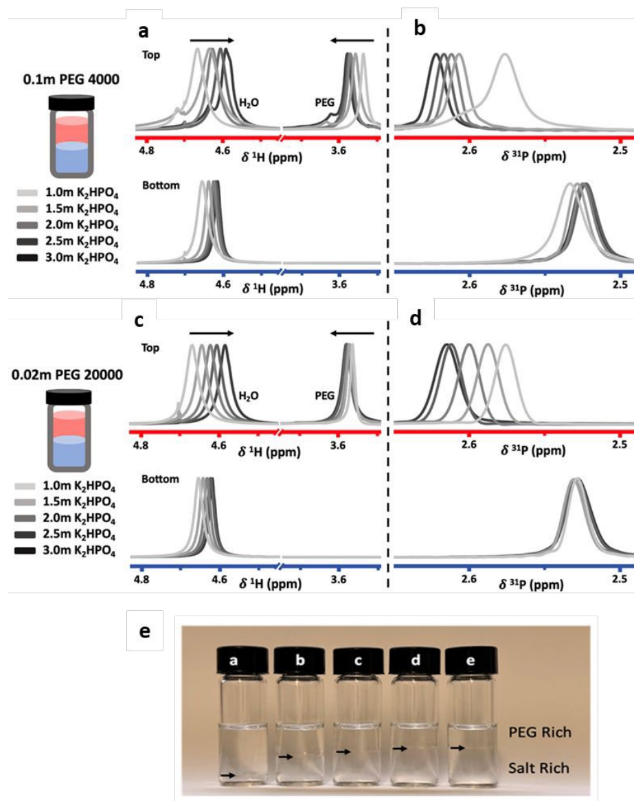
Figure 2. Normalized proton (a, c) and phosphorus (b, d) liquid-state NMR spectroscopy on bulk top (red) and bottom (blue) phases of PEG/K 2 HPO 4 systems with varying salt concentration. In proton spectra, the peak at ≈ 4.7ppm is characteristic of H 2 O while the peak at ≈ 3.6ppm is characteristic of PEG. The only peak in the phosphorus spectra arises from the K 2 HPO 4 . (e) photos of the biphasic systems using PEG20000 at different concentrations of K 2 HPO 4 (a: 1.0m, b: 1.5m, c: 2.0m, d: 2.5m and e: 3.0m) showing the variation of the volumes of the top and bottom phases as function of salt concentration. Black arrows indicate the interface between the two phases.
