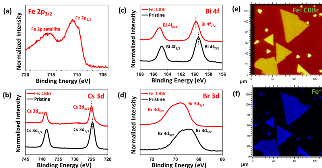
Figure 2. XPS scans of (a) Fe 2p 3 of the Fe:CBBr perovskite and (b) Cs 3d, (c) Bi 4f, and (d) Br 3d of Fe:CBBr (red) and pristine Cs 3 BiBr 6 (black) perovskites. (e) Total ion and (f) Fe + images of the Fe:CBBr perovskites obtained using ToF-SIMS.
