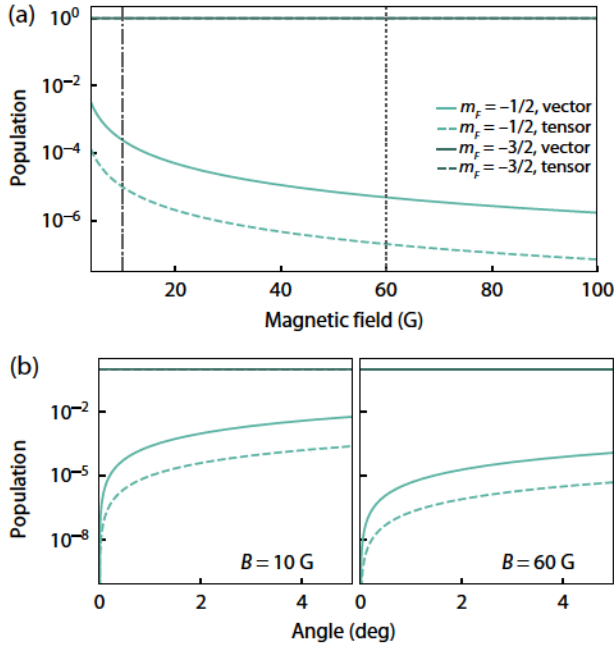
FIG. 13. State mixing of the ^3P_1, F = 3/2, m_F = -3/2 imaging state due to the vector and tensor light shifts. (a) The probabilities in the m_F = -3/2 (dark green) and m_F = -1/2 (light green) states due to the vector ( \gamma = 1^\circ and \theta = 0^\circ ; solid) and tensor ( \theta = 1^\circ and \gamma = 0^\circ ; dashed) light shifts as the magnitude of the applied magnetic field is varied. The gray vertical lines at 10 G (dash-dot) and 60 G (dotted) show field values chosen for the angle studies shown in (b). (b) We study the dependence on the angles \theta and \gamma , which describes the misalignment of the tweezer from the axis of quantization and the degree of ellipticity of the tweezer polarization, respectively. There is a sharp rise at angles close to 0^\circ due to the sudden appearance of the off-diagonal matrix elements.
