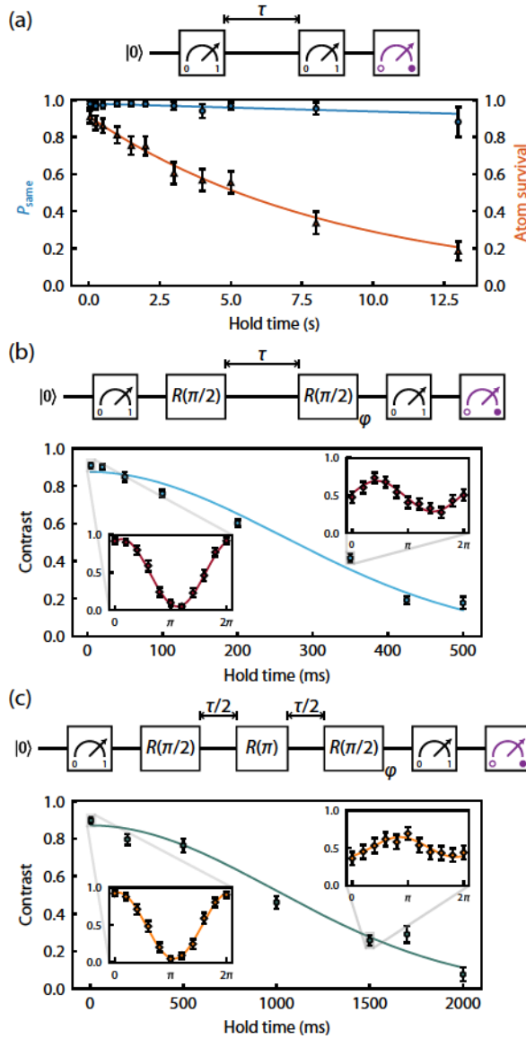
FIG. 17. Measurement of array averaged T_1 , T_2^* , and T_2^{\text{echo}} . (a) The circuit used to measure dark-state survival and the qubit depolarization time, T_1 . This circuit is identical to that shown in Fig. 3 except for the addition of a holding time \tau between the first two readouts. The qubit is also initialized in |0\rangle here in order to measure both P_{\text{same}} (blue circles) and the atom survival fraction (orange triangles), which are plotted below as a function of \tau . The atom survival lifetime is measured to be 8.8(3) s. The qubit depolarization time T_1 is estimated to be 230(50) s, but our data extend only to 13 s. (b) The circuit used to measure the qubit dephasing time, T_2^* . Here, the qubit is rotated to the equator for a time \tau before a \pi/2 pulse with phase \phi relative to the first is applied and the qubit state is measured. The resulting fringes in P_{\text{same}} are plotted as a function of \phi in the insets, and the contrast of the fringes is plotted as a function of the hold time \tau in the main plot. The decay of the contrast follows a Gaussian profile, the 1/e time of which we measure as T_2^* = 0.37(1) s. (c) The same circuit except with a \pi pulse in the middle of the precession time. This spin-echo sequence gives T_2^{\text{echo}} = 1.40(5) s.
