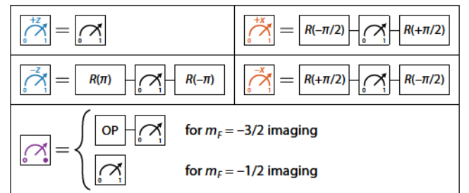
FIG. 2. Circuit legend. Simplified equivalent circuit elements. The number 0 or 1 and the open or filled circle distinguishes “qubit readout” from “atom readout”, respectively.
