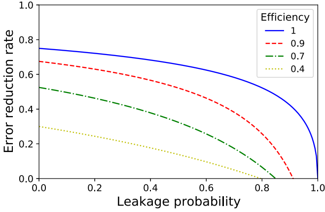
FIG. 3. Error reduction rate as a function of leakage probability for different detection efficiencies.
