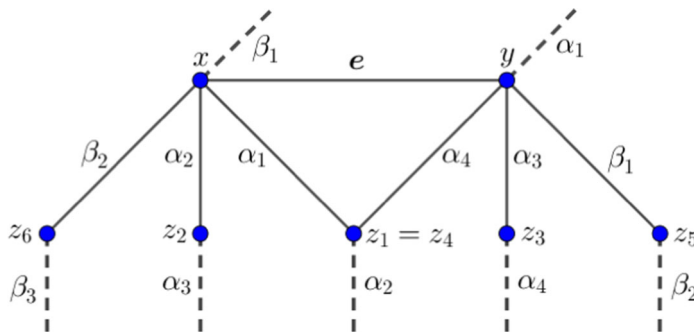
FIGURE 1 An e-fan F^e = (x, e, y, e_1, z_1, \dots, e_6, z_6)
