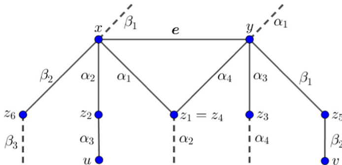
FIGURE 2 A C - e -fan F^{ce} = (x, e, y, e_1, z_1, \dots, e_6, z_6)
