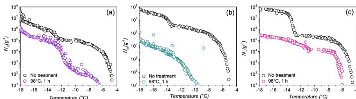
Figure 4. Effects of high-temperature treatment on the ice nucleation activity and corresponding IN population distribution of selected lichens. Shown are the cumulative number of INs ( N_m ) per gram of lichen sample of (a) P. britannica , (b) S. globosus , and (c) P. herrei .
