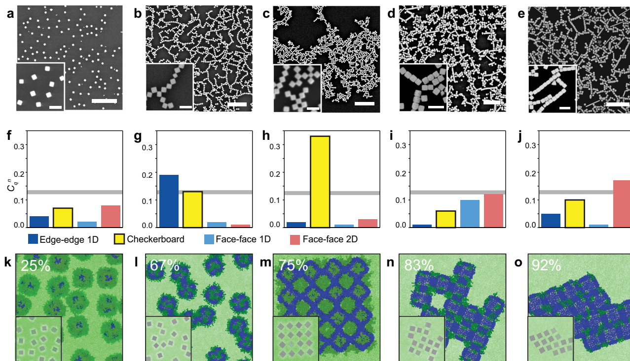
Fig. 3 | Experimental validation of the Ag NC mesophase diagram. a–e SEM images of the assembly results using Ag NCs post-synthetically modified with the following feedstock concentrations: a 0 \mu\text{M} , b 3 \mu\text{M} , c 6 \mu\text{M} , d 9 \mu\text{M} , and e 15 \mu\text{M} C_{16} and 50 \mu\text{M} PEG20K. Scale bar = 1 \mu\text{m} , inset = 200 nm. f–j Histogram of the Fourier coefficients C_q^n (unitless) of phases obtained from ACC analysis of each SEM image ( a–e ), with the threshold value for determining the
