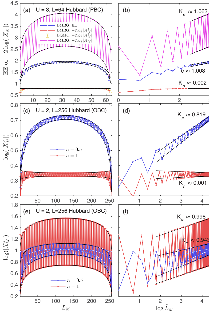
Figure 4: (a) Rényi entropy S_2 and disorder operators, -2\log|X_M^\rho(\frac{\pi}{2})| and -2\log|X_M^\sigma(\pi)| , for a half-filled Hubbard chain with PBC at U = 3 and system size L = 64 . The data points are obtained via DMRG and DQMC, and the horizontal axis L_M is the size of the region M . Figure (b) shows the same data vs the log of the conformal distance \log \tilde{L}_M = \log(\frac{L}{\pi} \sin \frac{\pi L_M}{L}) , which should be fitted to a linear function at large \log \tilde{L}_M , and we find that c \simeq 1.009 , K_\rho \simeq 0.004 and K_\rho \simeq 1.063 . (c,d) Charge disorder operator -\log|X_M^\rho(\frac{\pi}{2})| in a Hubbard chain with OBC at half- or quarter- fillings. Here we utilize DMRG to compute the disorder operator and set U = 2 and L = 256 . Fitting in Fig. (d) gives K_\rho \simeq 0.001 (half filling) and K_\rho \simeq 0.819 (quarter filling), consistent with the Bethe ansatz results K_\rho = 0 (half filling) and K_\rho \simeq 0.82 (quarter filling) [64]. (e,f) Spin disorder operator -\log|X_M^\sigma(\pi)| for the same model. The fitting gives K_\sigma \simeq 0.998 for half filling and K_\sigma \simeq 0.943 for quarter filling, consistent with the expected value K_\sigma = 1 .
