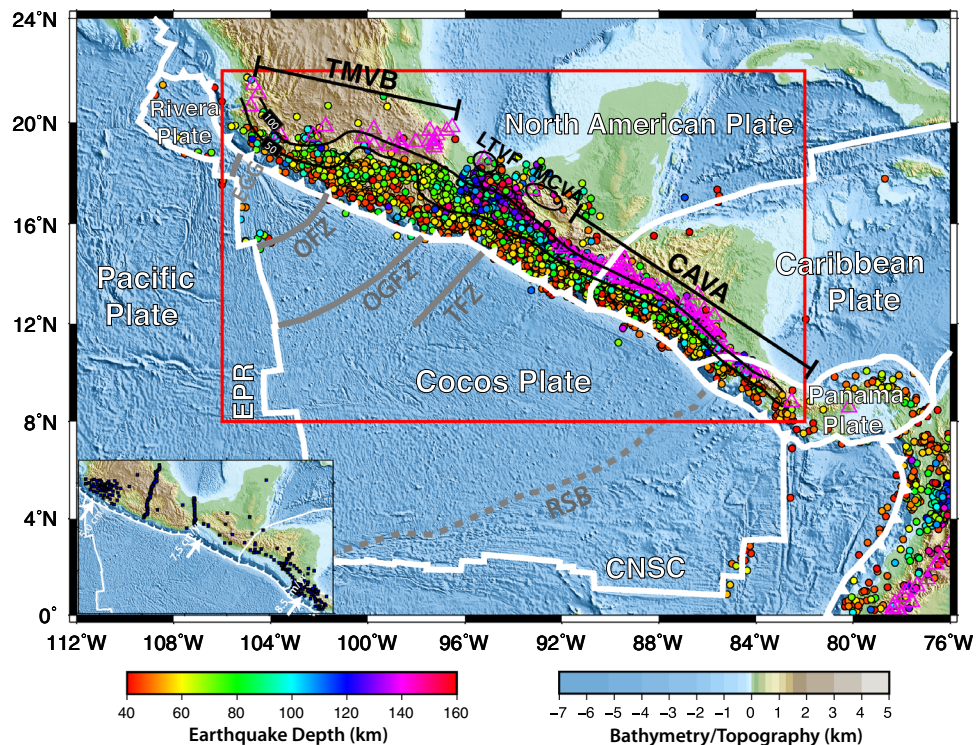
Figure 1. Tectonic setting of the Middle American subduction system. The thick white lines mark the major plate boundaries. The color-coded dots denote the earthquakes with magnitudes \geq 3.0 between 1997 and 2018 ( https://earthquake.usgs.gov/data/comcat ). The magenta triangles denote the Quaternary volcanoes. The black contours represent the plate interfaces at the depths of 50 km and 100 km extracted from Slab2.0 11 . The gray dashed line represents the rough-smooth boundary (RSB) 6 . The red box shows the imaging area in Figs. 2, 3, 4. The inset map shows the seismic stations (blue squares) used in this study and the convergence rates of the Cocos plate along the trench 4 . ERP the East Pacific Rise, CNSC the Cocos-Nazca spreading center, EGG the El Gordo Graben, OFZ the Orozco fracture zone, OGFZ the O’Gorman fracture zone, TFZ the Tehuantepec fracture zone, TMVB the Trans-Mexican volcanic belt, LTVF the Los Tuxtlas Volcanic Field, MCVA the Modern Chiapanecan volcanic arc, CAVA the Central American volcanic arc. The maps are generated using the Generic Mapping Tools (GMT) version 5.3.1 ( https://www.generic-mapping-tools.org ).
