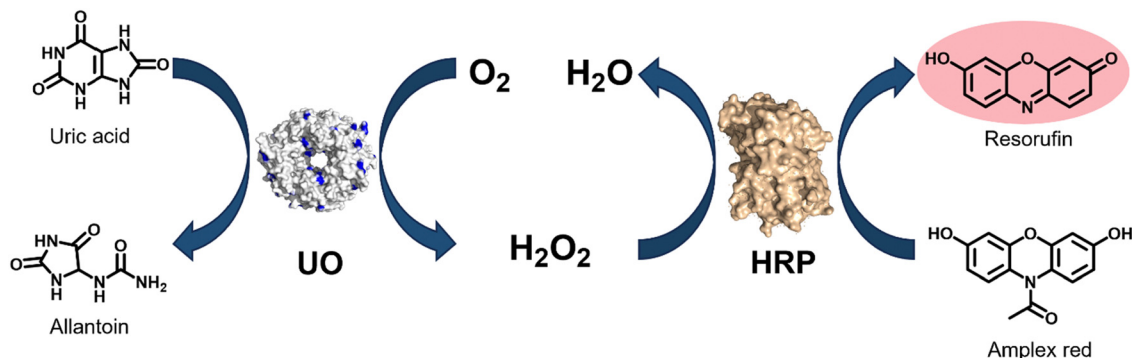
Fig. 2 Schematic illustration of uric acid/uricase activity assay using amplex red reagent.
