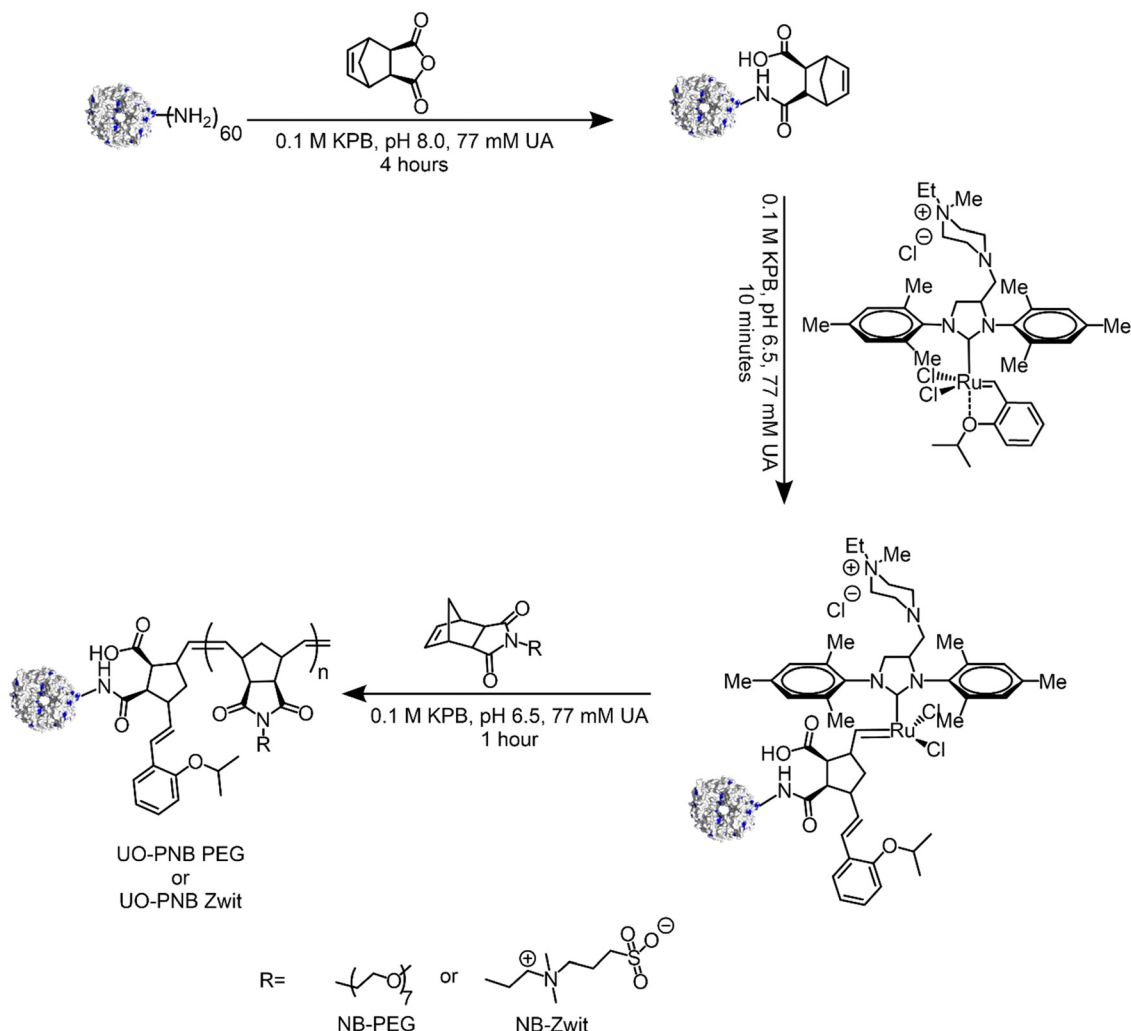
Scheme 1 Synthesis of UO conjugates by aqueous grafting-from ROMP technique.
