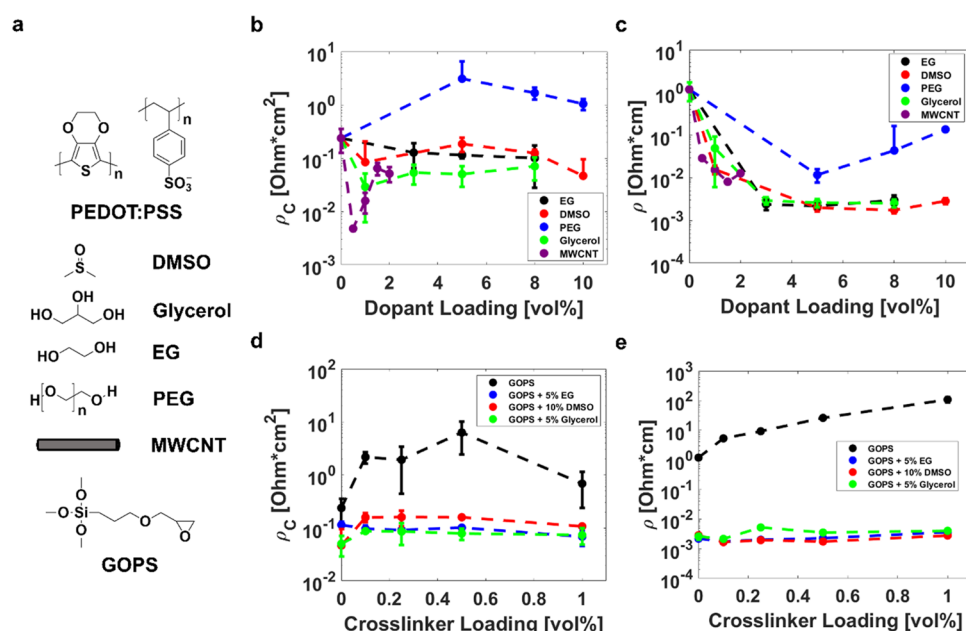
Figure 2. Contact and bulk electronic properties of PEDOT:PSS. (a) Chemical structures of dopants (dimethyl sulfoxide (DMSO), glycerol, ethylene glycol (EG), and poly(ethylene glycol) (PEG)) and of the crosslinker (3-glycidyloxypropyl)trimethoxysilane (GOPS). (b) Contact resistivity and (c) bulk resistivity relative to additive loading determined from TLM. The effect of crosslinker loading, as well as crosslinker incorporated with EG, DMSO, and glycerol as secondary dopants, on the (d) contact resistivity and (e) bulk resistivity of PEDOT:PSS determined using TLM.
