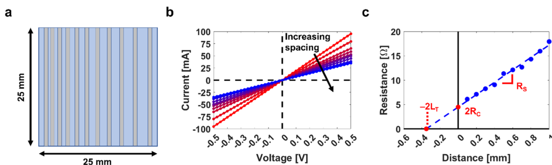
Figure 1. (a) Schematic of evaporated transfer length method (TLM) contacts (silver, 1.6 mm \times 25 mm) on a PEDOT:PSS film. Eleven contacts were evaporated to measure 10 different spacings (0.1–1 mm, in increments of 0.1 mm). (b) Current–voltage ( I – V ) measurements were conducted at each of the 10 different spacings. (c) Resistance was calculated from Ohm’s law and plotted relative to spacing. The data was fit using a linear regression, from which the sheet resistance ( R_S ), contact resistance ( R_C ), and transfer length ( L_T ) could be extracted. Using the geometry of the metal contacts and film thickness, the bulk resistivity ( \rho ) and contact resistivity ( \rho_C ) were calculated.
