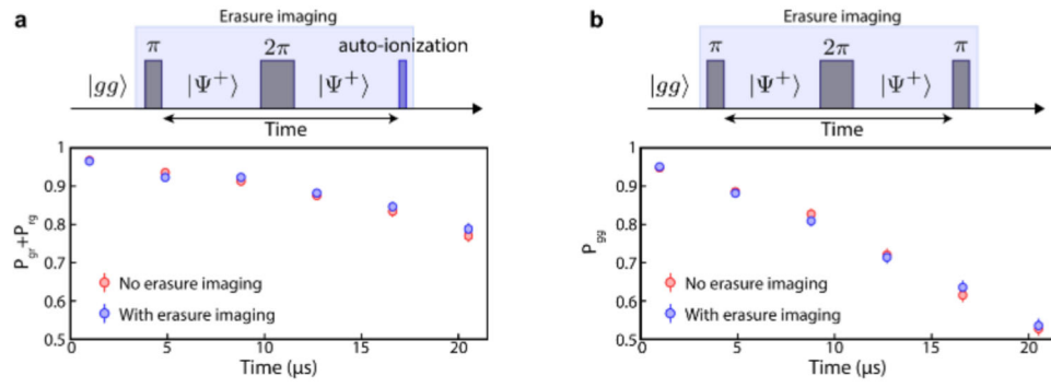
Extended Data Fig. 4 | Coherence preservation during erasure detection.
