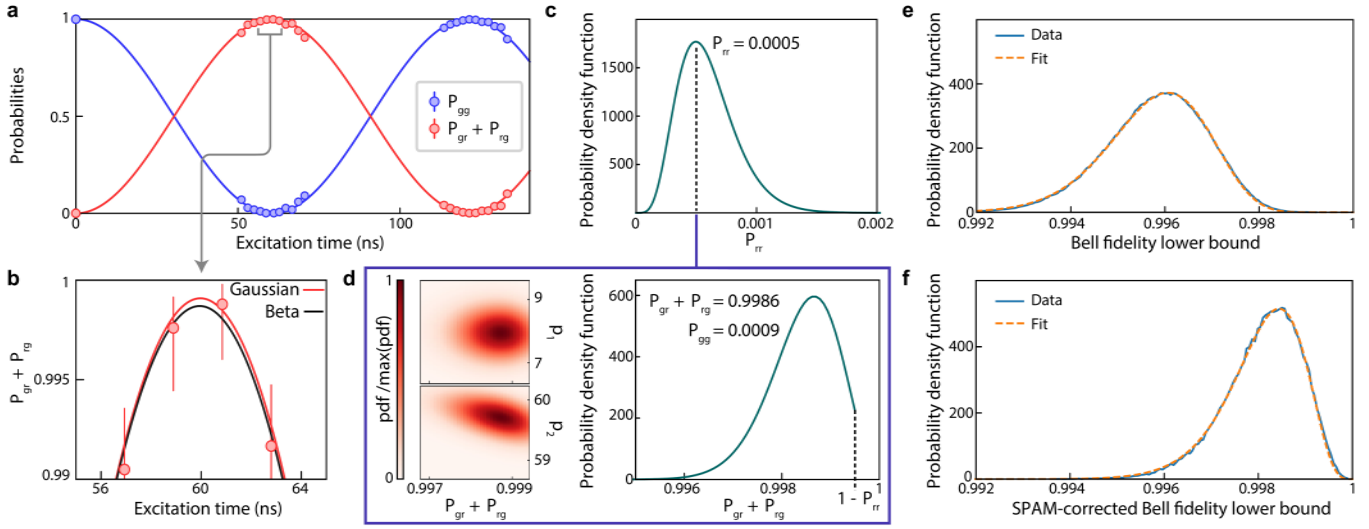
Extended Data Fig. 5 | Bell state fidelity measurement from blockaded Rabi oscillations. a , Probabilities of measuring both atoms in the ground state P_{gg} (blue markers) and a single atom in the ground state P_{gr} + P_{rg} (red markers) in the blockaded regime as a function of excitation time. Solid lines are guides to the eye. b , Zoom over the \pi time, where we prepare the Bell state |\Psi^+\rangle (see main text). We use a quadratic fit function of the form f(x) = p_0 + p_1(x - p_2)^2 to extract the population values at \pi and 2\pi times. We show the fit results (i) assuming the experimental data have a Gaussian uncertainty (red line), and (ii) using their true Beta distribution (black line). c, d , Fitting method used to obtain the probability distributions of P_{rr} , P_{gg} , and P_{gr} + P_{rg} at \pi and 2\pi times. We first experimentally obtain the Beta distribution of the probability P_{rr} to observe both atoms in the Rydberg state. We then perform a joint fit on P_{gr} + P_{rg} and P_{gg} with the same p_1 and p_2 fit coefficients for both. We fix the value of P_{rr} , and condition the joint fit such that the sum of all probabilities is always equals to one. We repeat this process for various values of P_{rr} . The results shown here are
