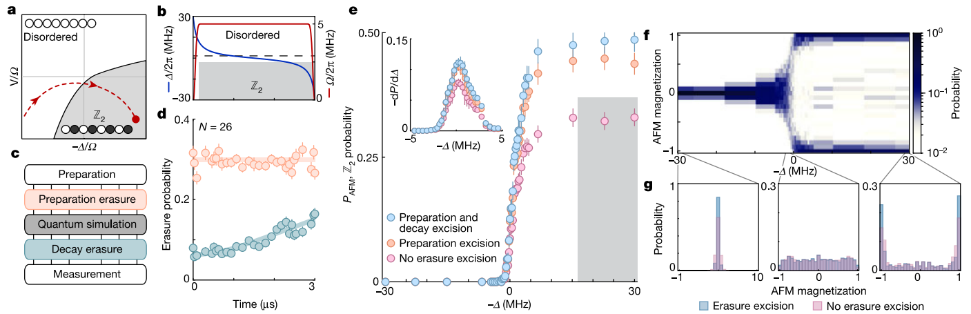
Fig. 3 | Erasure conversion in quantum simulation. a, b. We perform (b) quasi-adiabatic sweeps with N = 26 spins in the effective ground-state manifold of (a) an attractive Rydberg Hamiltonian (Methods), starting from the initially disordered phase and ending in the \mathbb{Z}_2 ordered phase. c. We perform two erasure images, one preceding the quantum simulation (to detect preparation errors) and one following (to partially detect Rydberg decay errors). d. The probability for detecting a preparation error (orange markers) remains constant while the probability for detecting a decay error (green markers) grows in agreement with the Rydberg lifetime and detection infidelities (solid lines; Methods). e. The total probability, P_{\text{AFM}} , for forming either of the
