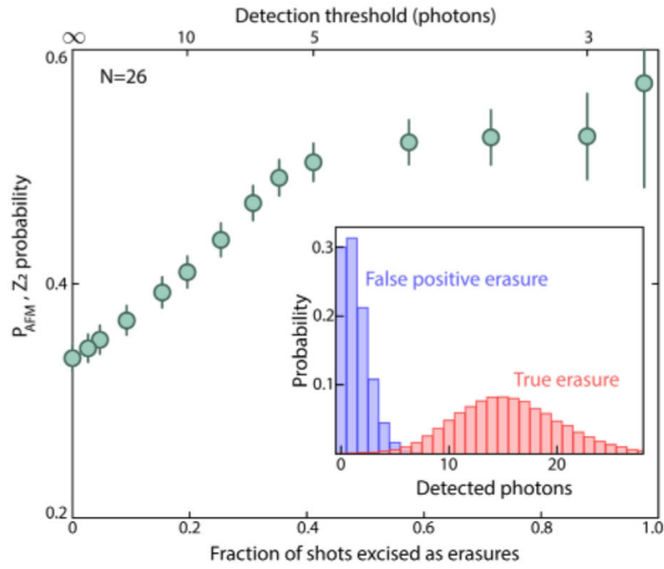
Extended Data Fig. 7 | Controlling fidelity gains from erasure-excision.
