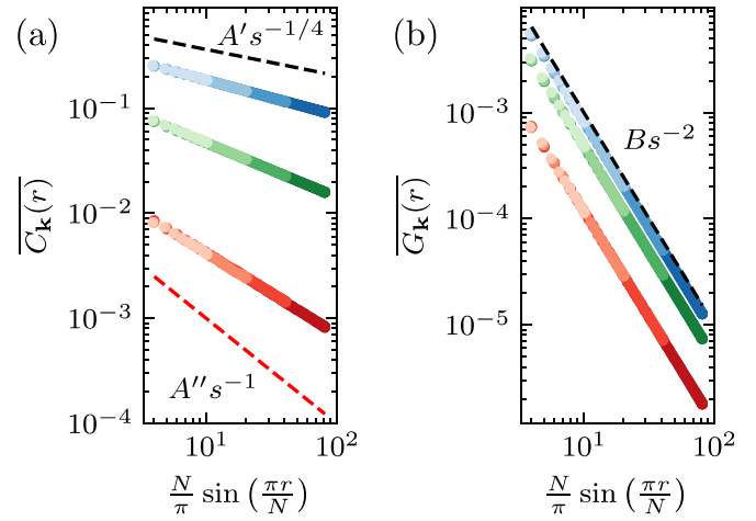
FIG. 4. Ensemble-averaged correlation functions (a) \overline{C_{\mathbf{k}}(r)} and (b) \overline{G_{\mathbf{k}}(r)} in the forced-measurement ensemble, for measurement probabilities p = 0.2 (blue), 0.5 (green), and 0.8 (red), and for system sizes N = 32, 64, 128 , and 256 (light to dark). Data are plotted as a function of s = \frac{N}{\pi} \sin(\frac{\pi r}{N}) to achieve scaling collapse of the various system sizes. Black dotted lines depict the behavior in the unmeasured system, while the red dotted line depicts the asymptotic power law of \overline{C_{\mathbf{k}}(r)} as p \rightarrow 1 . While \overline{G_{\mathbf{k}}(r)} \sim s^{-2} as in the unmeasured system, \overline{C_{\mathbf{k}}(r)} \sim s^{-2\Delta(p)} exhibits power-law scaling with a continuously varying exponent \Delta(p) . For the measurement probabilities shown, we have \Delta(0.2) \simeq 0.167 , \Delta(0.5) \simeq 0.252 , and \Delta(0.8) \simeq 0.367 .
