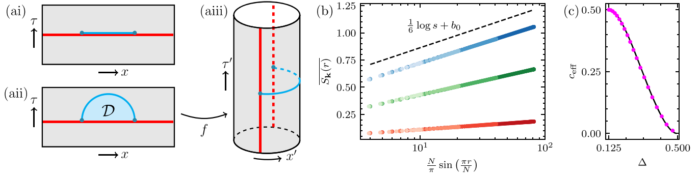
FIG. 5. (a) Spacetime diagrams depicting the relation between the average entanglement entropy \overline{S_k(r)} of the TFIM following forced projective measurements and the entanglement entropy S_d(N/2) of a dual impurity problem. (ai) One sheet of the Riemann surface used to compute the partition function \mathcal{Z}_n in Eq. (31). The red line denotes the measurement defect along the \tau = 0 line, while the blue line denotes the entanglement branch cut. (aii) By redefining the replica fields \psi^{(\alpha)}(\tau, x) in region \mathcal{D} as in Eq. (33), the branch cut is continuously deformed from the real axis onto the semicircle. (aiii) Using the conformal mapping of Eq. (34), the infinite plane is mapped to a cylinder of circumference L . The spacelike measurement defect is mapped to two timelike impurities at x' = 0 and x' = L/2 , while the deformed entanglement cut is mapped to a spacelike cut along the \tau' = 0 axis. (b) Ensemble-averaged entanglement entropy \overline{S_k(r)} of a contiguous subregion of r sites in the forced-measurement ensemble, for measurement probabilities p = 0.2 (blue), 0.5 (green), and 0.8 (red), and for system sizes N = 32, 64, 128 , and 256 (light to dark). Data are plotted as a function of s = \frac{N}{\pi} \sin(\frac{\pi r}{N}) to achieve scaling collapse of the various system sizes. The dotted line depicts the behavior in the unmeasured system. We observe \overline{S_k(r)} \sim \frac{c_{\text{eff}}(p)}{6} \log s + b_0 exhibits logarithmic scaling at all measurement probabilities with a continuously decreasing effective central charge c_{\text{eff}}(p) . For the measurement probabilities shown, c_{\text{eff}}(0.2) \simeq 0.478 , c_{\text{eff}}(0.5) \simeq 0.339 , and c_{\text{eff}}(0.8) \simeq 0.105 . (c) Numerical comparison between the effective central charge c_{\text{eff}}(p) in the average entanglement entropy \overline{S_k(r)} in the forced-measurement ensemble, and the effective central charge c_{\text{eff},d}(g_d) of the half-system entanglement entropy S_d(N/2) of a dual TFIM with defects described by the Hamiltonian (36). Purple dots: effective central charge c_{\text{eff}}(p) for several measurement probabilities p between 0 and 0.95 in increments of 0.05, as a function of the effective scaling dimension \Delta(p) governing the decay of \overline{C_k(r)} . Black curve: effective central charge c_{\text{eff},d}(g_d) as a function of the scaling dimension \Delta_d(g_d) governing the decay of order parameter correlations \langle \psi_d | Z_1 Z_{N/2} | \psi_d \rangle between the two impurities.
