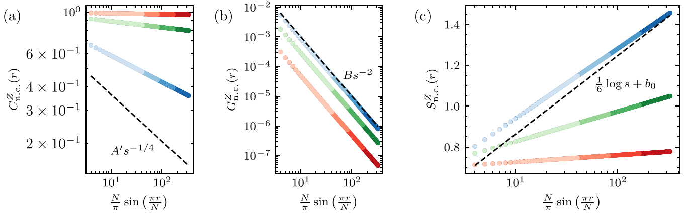
FIG. 9. [(a),(b)] No-click correlation functions C_{n.c.}^Z(r) and G_{n.c.}^Z(r) and (c) entanglement entropy S_{n.c.}^Z(r) , for measurement strengths 1 - \cos \alpha = 0.1 (blue), 0.3 (green), and 0.5 (red), and for system sizes N = 128, 256, 512 , and 1024 (light to dark). Data are plotted as a function of s = \frac{N}{\pi} \sin(\frac{\pi r}{N}) to achieve scaling collapse of the various system sizes. Dotted lines depict the behavior of the unmeasured system. Similar to the case of forced projective Z_j Z_{j+1} measurements, G_{n.c.}^Z(r) \sim s^{-2} exhibits the same power-law scaling as the unmeasured system, while C_{n.c.}^Z(r) \sim s^{-2\Delta_{n.c.}^Z(\alpha)} exhibits a continuously varying power-law exponent and S_{n.c.}^Z(r) \sim \frac{c_{n.c.}^Z}{3} \log s + b_{n.c.}^Z(\alpha) exhibits a continuously varying effective central charge.
