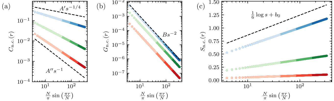
FIG. 8. [(a),(b)] No-click correlation functions C_{n.c.}(r) and G_{n.c.}(r) and (c) entanglement entropy S_{n.c.}(r) , for measurement strengths 1 - \cos \alpha = 0.1 (blue), 0.3 (green), and 0.5 (red), and for system sizes N = 128, 256, 512 , and 1024 (light to dark). Data are plotted as a function of s = \frac{N}{\pi} \sin(\frac{\pi r}{N}) to achieve scaling collapse of the various system sizes. Dotted lines depict the behavior in the unmeasured system. Similar to the case of forced projective measurements, G_{n.c.}(r) \sim s^{-2} exhibits the same power-law scaling as in the unmeasured system, while C_{n.c.}(r) \sim s^{-2\Delta_{n.c.}(\alpha)} exhibits a continuously varying power-law exponent and S_{n.c.}(r) \sim \frac{c_{\text{eff},n.c.}(\alpha)}{3} \log s + b_{n.c.}(\alpha) exhibits a continuously varying effective central charge.
