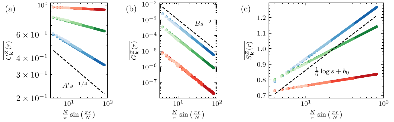
FIG. 7. [(a),(b)] Ensemble-averaged correlation functions \overline{C_k^Z(r)} and \overline{G_k^Z(r)} and (c) entanglement entropy \overline{S_k^Z(r)} in the forced-measurement ensemble, for measurement probabilities p = 0.2 (blue), 0.5 (green), and 0.8 (red), and for system sizes N = 32, 64, 128 , and 256 (light to dark). Data are plotted as a function of s = \frac{N}{\pi} \sin(\frac{\pi r}{N}) to achieve scaling collapse of the various system sizes. Dotted lines depict the behavior of the unmeasured system. While \overline{G_k^Z(r)} \sim s^{-2} exhibits the same scaling as the unmeasured system, \overline{C_k^Z(r)} \sim s^{-2\Delta^Z(p)} exhibits a continuously varying exponent \Delta^Z(p) ; unlike in the forced X_j measurement scheme, where \overline{C_k(r)} \sim r^{-2\Delta(p)} featured a monotonically increasing scaling dimension \Delta(p) , here the scaling dimension \Delta^Z(p) continuously decreases to zero with increasing measurement probability. The entanglement entropy \overline{S_k^Z(r)} \sim \frac{c_{\text{eff}}^Z(p)}{3} \log r + b_5(p) again features a continuously decreasing effective central charge c_{\text{eff}}^Z(p) , but with a nonmonotonic contribution b_5(p) .
