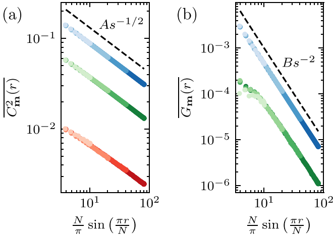
FIG. 2. Ensemble-averaged correlation functions (a) \overline{C_m^2(r)} and (b) \overline{G_m(r)} as defined in Eq. (7), for measurement probabilities p = 0.2 (blue), 0.5 (green), and 0.8 (red), and for system sizes N = 32, 64, 128 , and 256 (light to dark). Data are plotted as a function of s = \frac{N}{\pi} \sin(\frac{\pi r}{N}) to achieve scaling collapse of the various system sizes. Dotted lines depict the behavior in the unmeasured system. Both correlation functions exhibit excellent scaling collapses with the power-law exponents of the unmeasured system at sufficiently large distances.
