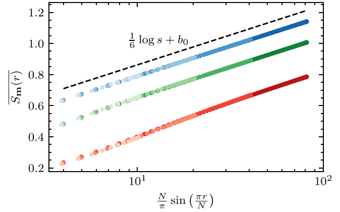
FIG. 3. Ensemble-averaged entanglement entropy \overline{S_m(r)} for a contiguous subregion [0 : r] of r sites, for measurement probabilities p = 0.2 (blue), 0.5 (green), and 0.8 (red), and for system sizes N = 32, 64, 128 , and 256 (light to dark). Data are plotted as a function of s = \frac{N}{\pi} \sin(\frac{\pi r}{N}) to achieve scaling collapse of the various system sizes. The dotted line depicts the behavior of the unmeasured system. For each measurement probability, the entanglement entropy exhibits an excellent scaling collapse with logarithmic scaling corresponding to the central charge c = 1/2 of the unmeasured system at sufficiently large distances.
