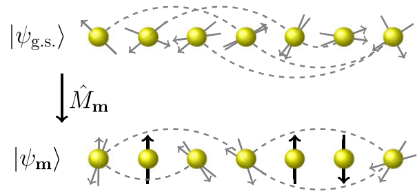
FIG. 1. Schematic depiction of the measurement protocol considered in this work. The ground state |\psi_{g.s.}\rangle of the critical transverse-field Ising model (1) is measured using the measurement operator \hat{M}_m , which is a product of an extensively large set of local projectors. The remaining state |\psi_m\rangle \propto \hat{M}_m |\psi_{g.s.}\rangle retains nontrivial long-range correlations and entanglement scaling.
