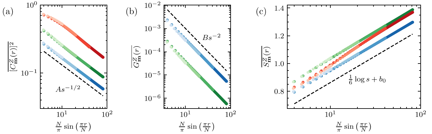
FIG. 6. [(a),(b)] Ensemble-averaged correlation functions \overline{[C_m^Z(r)]^2} and \overline{G_m^Z(r)} and (c) entanglement entropy \overline{S_m^Z(r)} following Z_j Z_{j+1} measurements with outcomes sampled according to the Born rule, for measurement probabilities p = 0.2 (blue), 0.5 (green), and 0.8 (red), and for system sizes N = 32, 64, 128 , and 256 (light to dark). Data is plotted as a function of s = \frac{N}{\pi} \sin(\frac{\pi r}{N}) to achieve scaling collapse of the various system sizes. Similar to the ensemble with X_j measurements (see Sec. III), both correlation functions retain their power-law scaling with exponents of the unmeasured system at sufficiently long distances, while the entanglement entropy retains its logarithmic scaling with central charge c = 1/2 of the unmeasured system.
