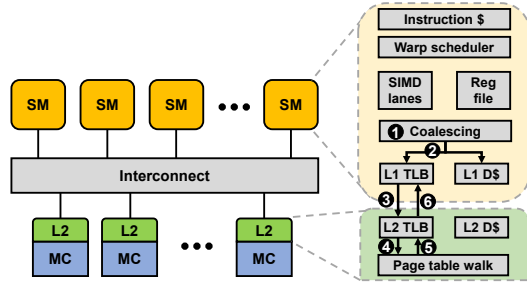
Fig. 1. Baseline GPU Architecture.
