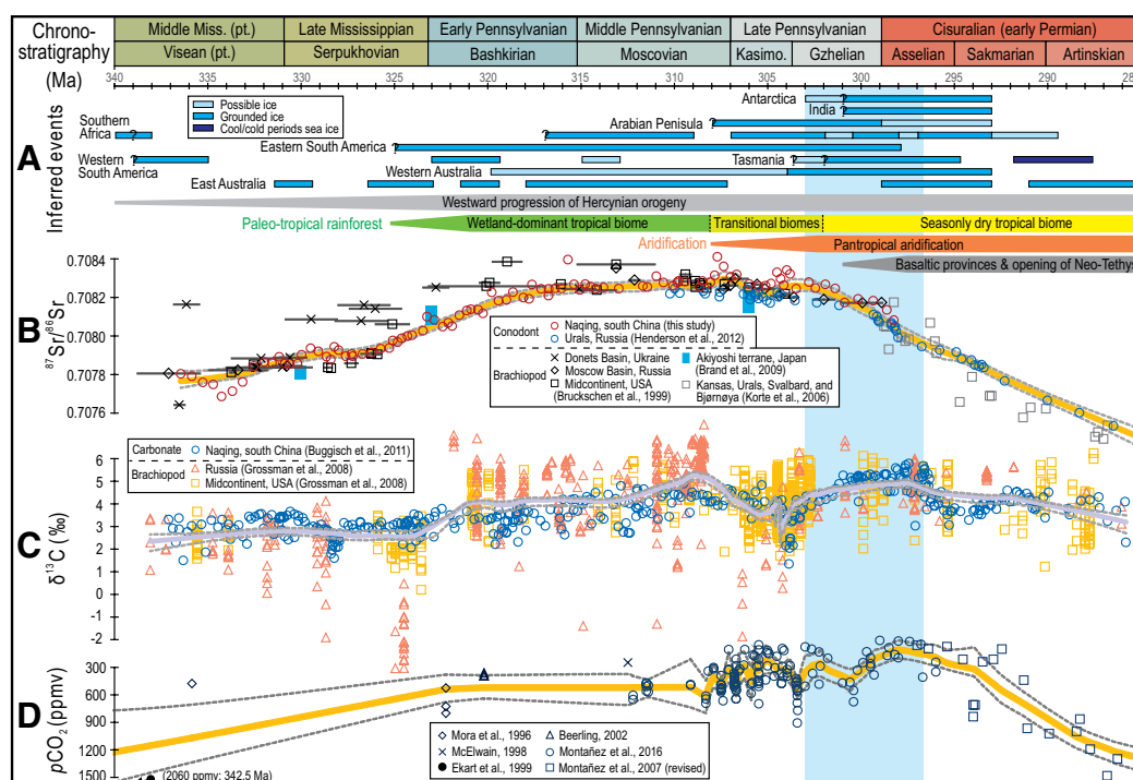
Figure 2. Inferred geologic events and proxy records for the late Paleozoic ice age (LPIA). A: Inferred geologic events (see text for explanation and references). (Glaciation history after Montañez and Poulsen [2013]; vegetation record modified from Montañez [2016]). B: Conodont-based ^{87}\text{Sr}/^{86}\text{Sr} record from Naoqing, south China (this study) and the Urals, Russia (Henderson et al. 2012); previously published brachiopod (“good” data only) ^{87}\text{Sr}/^{86}\text{Sr} values renormalized to 0.710249 (strontium carbonate isotopic standard SRM 987). Locally weighted scatterplot smoothing (LOESS) trend lines for B (conodont-based ^{87}\text{Sr}/^{86}\text{Sr} values), C, and D are as in Figure 1. C: Age-re-calibrated carbonate \delta^{13}\text{C} record from Naoqing and previously published brachiopod \delta^{13}\text{C} records. D: Published atmospheric p\text{CO}_2 estimates (see the Data Repository [see footnote 1] for details). Vertical shading highlights interval of p\text{CO}_2 and ^{87}\text{Sr}/^{86}\text{Sr} decoupling.
