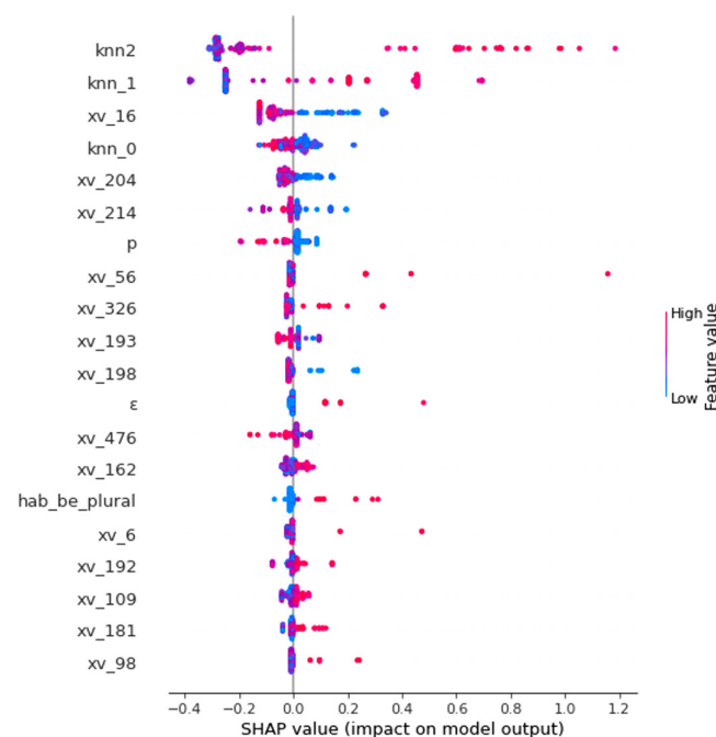
FIG. 3. (Color online) Bee swarm plot depicting the relative impact of features in the ensemble classifier for the child speech from the GSU Kids’ speech database.
