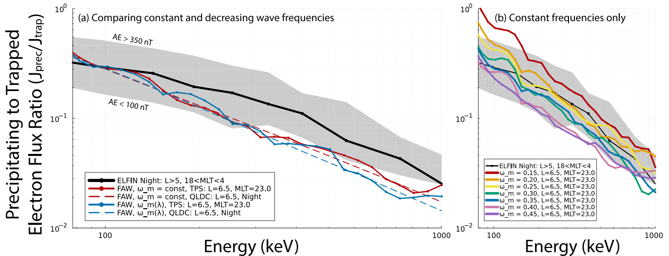
Figure 4. To compare the effects of two frequency models, precipitating-to-trapped electron flux ratio j_{prec}/j_{trap} plotted for ELFIN statistics on the nightside (black) is shown in comparison with j_{prec}/j_{trap} ratios obtained from test particle simulations (TPS, solid lines) and quasi-linear diffusion code (QLDC, dashed lines). In (a), Frequency Model 2 (frequency decreasing toward higher latitudes, blue) produces slightly higher precipitation rates at 100 keV relative to 1 MeV as compared to a constant \omega_m = 0.35 (red). Plot (b) shows results from a variety of normalized wave frequency values that do not vary as a function of magnetic latitude, demonstrating that absolute frequency has little effect on the slope of the precipitation energy spectra.
