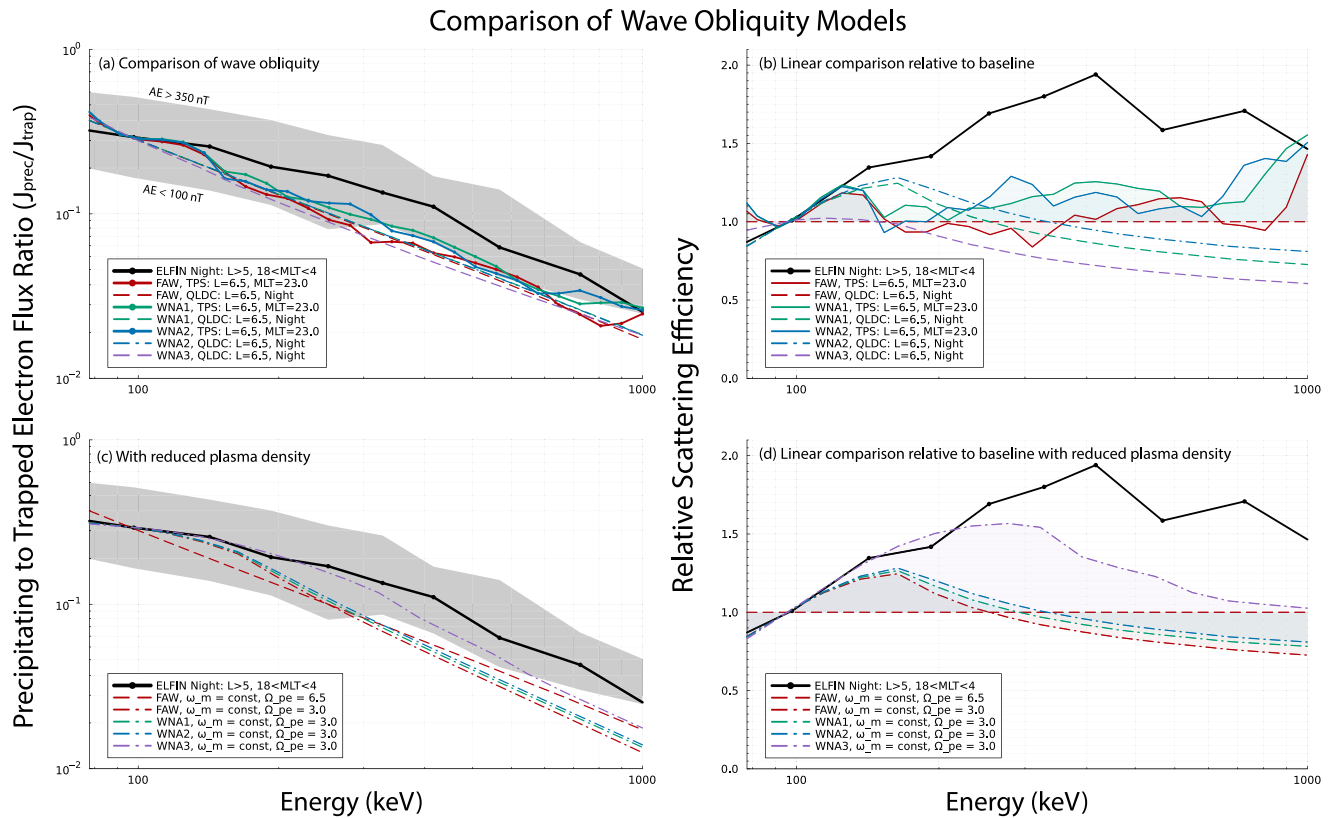
Figure 5. ELFIN-observed j_{prec}/j_{trap} flux ratio at L > 5 on the nightside (18 – 4 MLT) as a function of electron energy (black). The corresponding ratios j_{prec}/j_{trap} obtained from test particle simulations (TPS, solid curves) and from the quasi-linear diffusion code (QLDC, dashed curves) are displayed for lower-band chorus waves in (a), using frequency Model 1 of constant frequency, and parameterized by four wave normal angle models: FAW (red), WNA1 (green), WNA2 (blue), and WNA3 (purple), with a normalization to observations at 97 keV, adopting a typical \Omega_{pe} = 6.5 at L = 6.5 and 23 MLT. (c) Shows QLDC results for the same four wave normal angle models but for a reduced plasma density of \Omega_{pe} = 3.0 . (b, d) Show relative comparisons for each corresponding plot to the same reference baseline curve (red dashed line).
