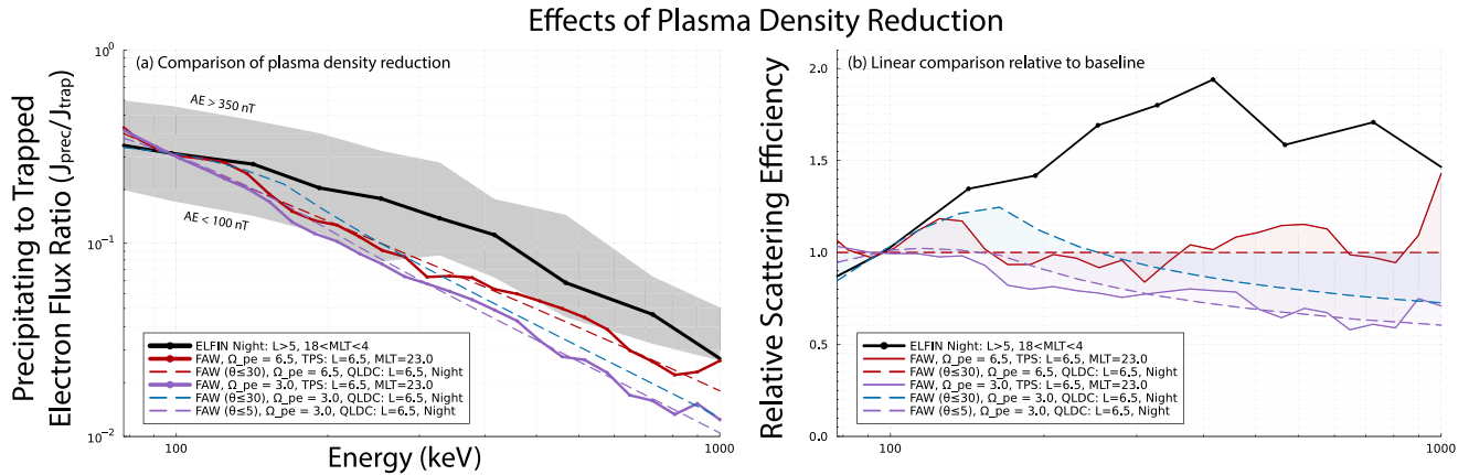
Figure 3. (a) Shows ELFIN-measured precipitating-to-trapped electron flux ratio at L > 5 on the nightside (18 – 4 MLT) as a function of energy (black curve). The corresponding j_{prec}/j_{trap} flux ratio obtained from test particle simulations is shown for parallel (FAW model, \theta = 0^\circ ) lower-band chorus waves, using frequency Model 1 ( \omega_m = \text{constant} ) and a typical \Omega_{pe} = 6.5 at L = 6.5 and 23 MLT (solid red). Results from the quasi-linear diffusion code using the same parameters are shown in dashed red. Similarly, the cases of reduced density \Omega_{pe} = 3 modeled with test particle simulation (solid purple), quasi-linear diffusion code using narrow-band field aligned waves ( \delta\theta = 5^\circ , dashed purple), and quasi-parallel waves ( \delta\theta = 30^\circ , dashed blue), are shown. All simulation results are normalized to observations at 97 keV. (b) Shows j_{prec}/j_{trap} flux ratios relative to the baseline case (red dashed line) on a linear scale.
