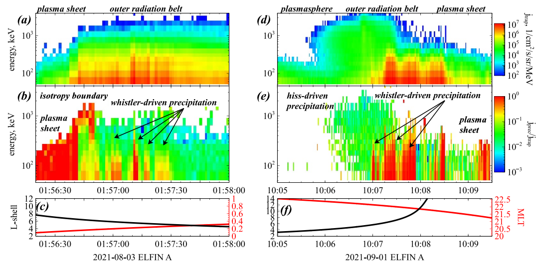
Figure 1. Two examples of ELFIN observations with strong precipitation of energetic electrons in the nightside MLT sector showing locally trapped electron fluxes (a, d), precipitating-to-trapped flux ratio (b, e), and ELFIN's MLT, L -shell coordinates from Tsyganenko (1989) model (c, f).
