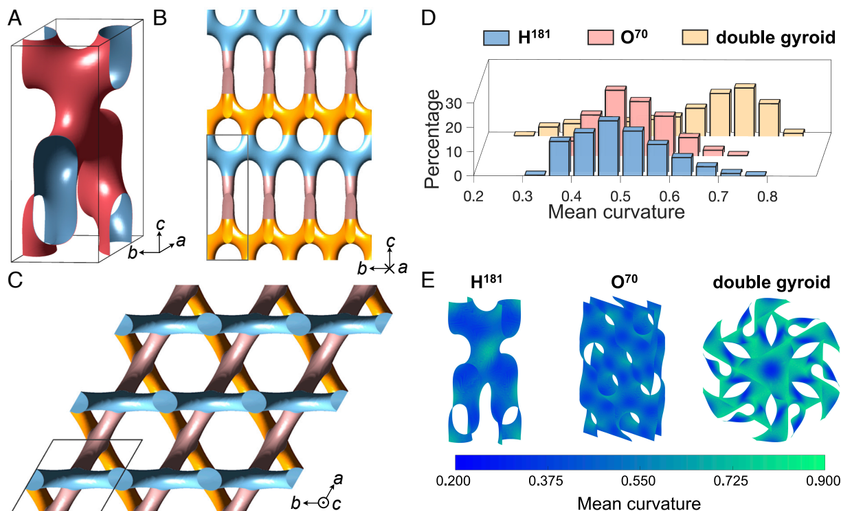
Fig. 5. Structure of H^{181} . (A) Interface corresponding to \phi_A = 0.5 . (B) Projection along the [100] direction. (C) Projection along the [001] direction. For (B) and (C), the skeletons indicate regions where the minority block density satisfies \phi_A = 0.90 , and the boxes are the unit cell. The coloring in the projections in (B) and (C) indicates the threefold connectors with different orientations within the 3D unit cell of Fig. 4B. (D) Histograms and (E) color maps of the mean curvature of A/B interface of H^{181} , O^{70} , and double gyroid. H^{181} and O^{70} have similar average mean curvature (0.498 and 0.506) and curvature distributions in the histogram, while double gyroid has a higher interfacial curvature of 0.621.
