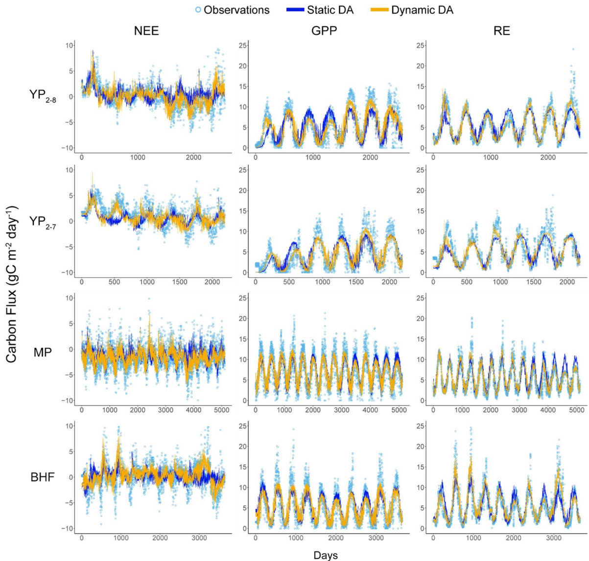
Fig. 2 Data-model fusion of eddy-covariance carbon flux data and the TECO ecosystem model. Simulations were constrained statically using multi-year data (dark blue lines) and dynami-
