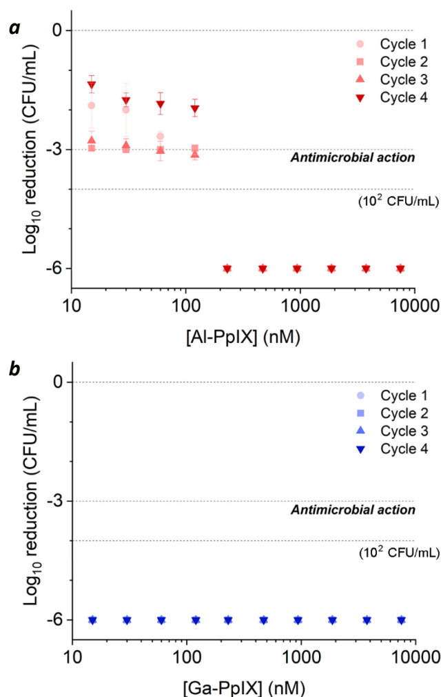
Figure 6. aPDI of S. aureus challenged by 1 mM H 2 O 2 after the log-growth phase, repeated over 4 cycles. (a) Al-PpIX; (b) Ga-PpIX. Studies were conducted with 30-s exposure to 405-nm light (4.2 J/cm 2 ) using an initial population of 10 6 CFU/mL.
