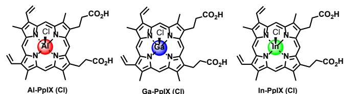
Figure 1. Chloride salts of non-iron heme analogs (M-PpIX) with Group 13 elements Al, Ga, and In.
