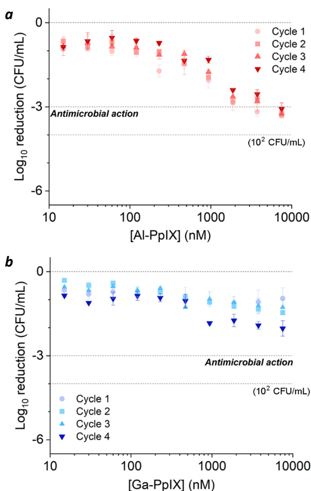
Figure 5. aPDI of S. aureus challenged by 1 mM H 2 O 2 during the log-growth phase, repeated over 4 cycles. (a) Al-PpIX; (b) Ga-PpIX. Studies were conducted with 30-s exposure to 405-nm light (4.2 J/cm 2 ) using an initial population of 10 6 CFU/mL.
