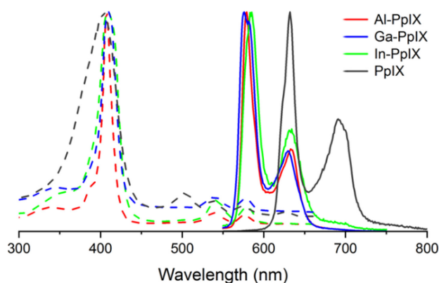
Figure 2. Normalized absorption (dashed curves) and luminescence spectra (solid curves) of M-PpIX(Cl) (M = Al, Ga, and In) and PpIX in 8 \mu M in DMSO.
