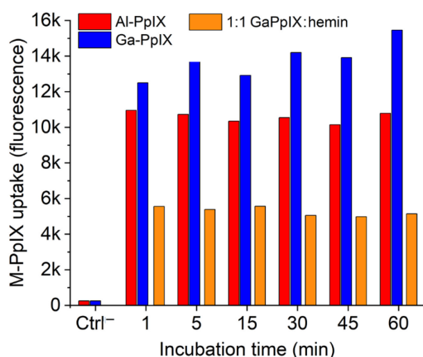
Figure 3. Histogram of flow cytometry (FC) data for S. aureus (PCI 1203) cultured in Fe-deficient media, following treatment with 10 \mu M M-PpIX, where M = Al (red) or Ga (blue). Specificity for M-PpIX uptake by S. aureus established by competition assay using a 1:1 Ga-PpIX:hemin mixture (orange). All bacteria were fixed after M-PpIX treatment and before FC injection; see ESI for original FC data.
