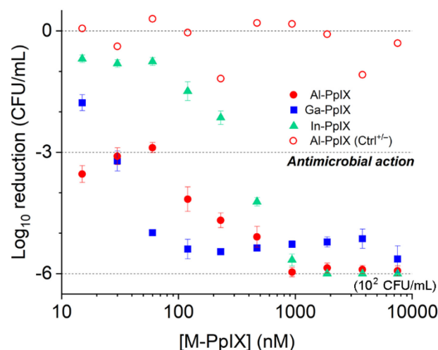
Figure 4. Antimicrobial photodynamic inactivation (aPDI) of S. aureus (PC 1203) by M-PpIX, with 30-s exposure to 405-nm light (4.2 J/cm 2 ). Data for antimicrobial activity of Al-PpIX without light (Ctrl +/− ) included for comparison.
