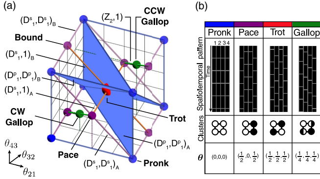
FIG. 3. (a) The eight categories of invariant manifolds for a network of four nodes with square symmetry predicted by the H/K theorem presented in the state space of phase differences is a periodic three-dimensional (3D) cube, \theta_{ij} \in (0, 2\pi] . There are four categories of phase-locked periodic states (points), three categories of lines, and one category of planes; each are colored according to their category in Table II. All linear and planar invariant are periodic; blue lines correspond to the edges of the planes. (b) The four point manifolds predicted by theory, Pronk, Pace/Bound, Trot, and Gallop, are represented (first row) as space-time plots, (second row) as networks with synchronized clusters indicated by color, and (third row) as a triplet of phase differences, \theta , with units of fraction of a period.
