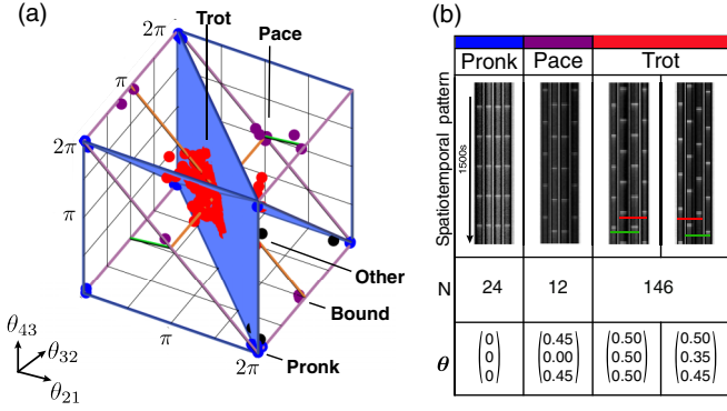
FIG. 4. (a) Experimental phase-locked states plotted within state space. There are three characteristic distributions, associated with the Pronk, Pace/Bound, and Trot states. They are colored to reflect which H/K state they are affiliated with as in Fig. 3, using a state-specific cutoff determined by simulations detailed later in Appendix G. (b) First row: Example space-time plots of steady states in (a). Due to the wide dispersion of the Trot distribution, different states within the Trot distribution can appear qualitatively different; the last column shows one such example. Second row: The number of times a state is observed. Third row: Measured phase difference. Videos of experiments shown in Movies S1–S4 of the Supplemental Material [33].
