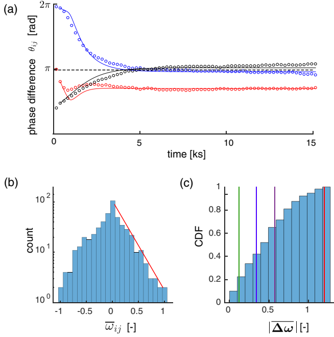
FIG. 7. (a) Example experimental trajectory converging to steady state (circles), and best-fit phase model (solid line). The fit model required heterogeneity \Delta\omega_{ij} \neq 0 to fit data. For comparison, the steady-state phase difference \theta^* = (\pi, \pi, \pi) of the homogeneous phase model is shown (dashed horizontal line). (b) Distribution of best-fit dimensionless intrinsic frequency differences \bar{\Delta\omega} = \Delta\omega/kH_{\max} , nondimensionalized by the coupling rate k and amplitude of the interaction function H_{\max} (Fig. 2). The distribution is approximately Laplacian with scale factor b = 0.2441 . (c) Cumulative probability distribution of |\Delta\omega| from (a). Lines denote the average heterogeneity \langle |\Delta\omega^*| \rangle at which the bifurcation analysis predicts the attractors: Gallop (green), Pronk (blue), Pace/Bound (purple), and Trot (red) will lose stability (Table III). This predicts the fraction of experiments that can support a given attractor given the inherent heterogeneity.
