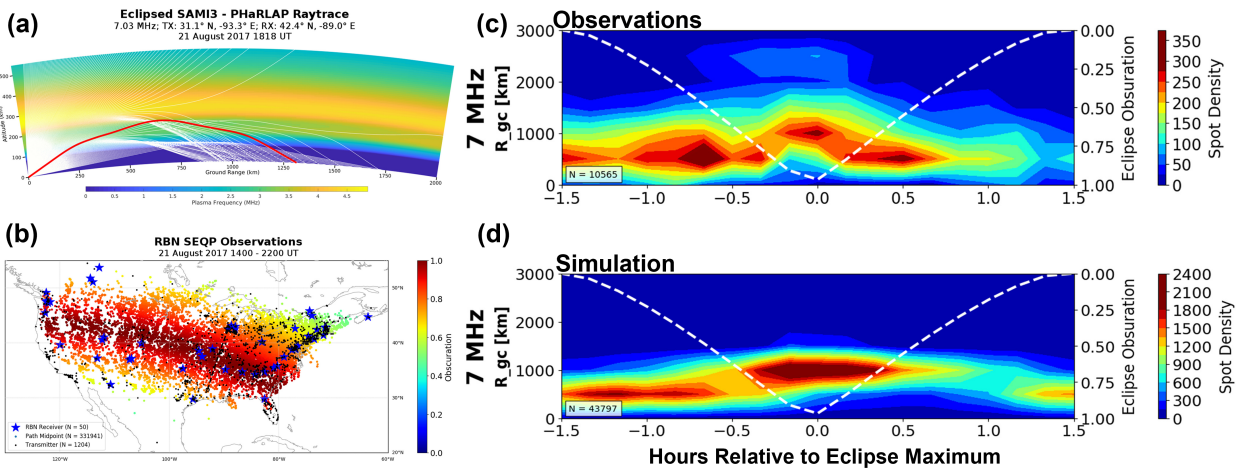
Figure 2: Solar Eclipse QSO Party Results from Frissell et al. [16]. (a) 7 MHz ray trace through eclipsed SAMI3 ionosphere along the dashed line path from south to north shown in (b). (b) Map of ham radio HF observation locations; black dots are transmitters (TX), blue stars are RBN receivers (RX), and TX-RX midpoints are dots color coded by maximum eclipse obscuration at that location. (c) Observations of the 7 MHz amateur radio band as a function of time relative to eclipse maximum, showing that the communication distance extends as ionospheric electron densities decrease during the eclipse. (d) Simulation of (c) using the PHaRLAP ionospheric raytracing library [3] and an eclipsed version of the first-principles SAMI3 ionospheric model [29]. Data-model comparisons such as this are a powerful method for linking amateur radio observations to physical understanding.
