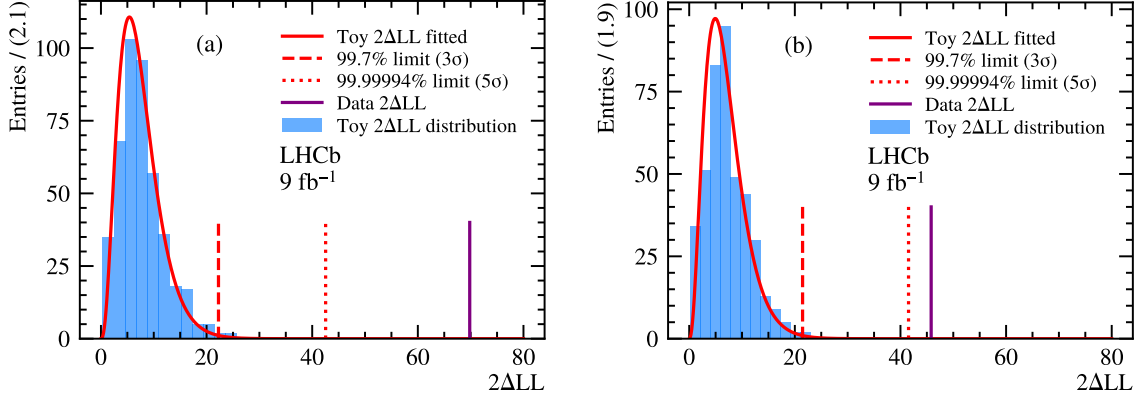
Figure 10: Significance tests for the new D_s \pi states in the (a) B^0 \rightarrow \bar{D}^0 D_s^+ \pi^- and (b) B^+ \rightarrow D^- D_s^+ \pi^+ samples. The blue histogram is the distribution of 2\Delta LL and the red solid curve shows the fitted \chi^2 PDF. The red dashed and dotted lines are the 2\Delta LL values corresponding to 3\sigma and 5\sigma , and the purple solid line is the 2\Delta LL measured in the data.
