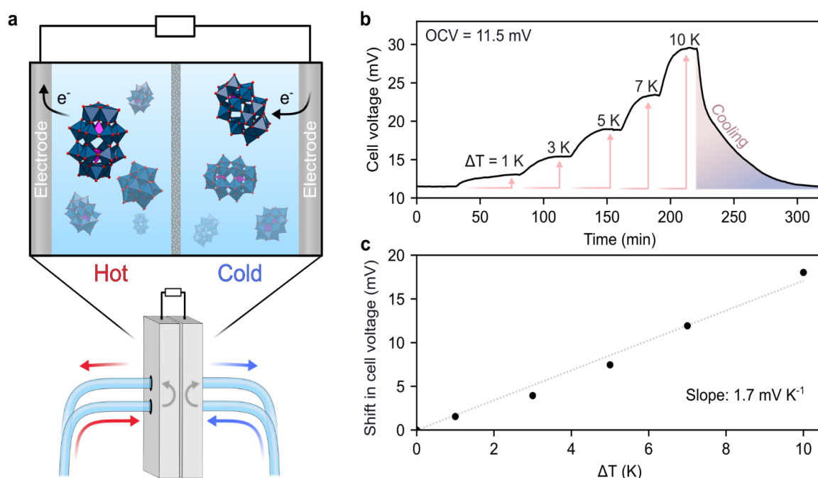
Figure 4. (a) Schematic of a flow cell where the hot and cold sides are separated by a Nafion membrane (for a detailed schematic, see Supporting Information). (b) Measured cell voltage of the flow cell, showing a difference in cell voltage of ~17 mV with a temperature difference of 10 K between the hot and cold solutions (1 mM WD solution made from 0.1 M sodium acetate buffer, pH = 5.5), also showing that the voltage reversibly disappears upon removal of the temperature gradient. The open-circuit voltage (OCV) of the flow cell was 11.5 mV after the equilibration period. (c) Observed shift in cell voltage as a function of temperature difference ( \Delta T ) for the flow cell, showing a linear relationship.
