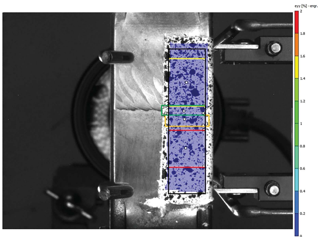
Fig. 2 — Etched F22/625 CWTT sample with applied DIC pattern. Also shown are the physical extensometer; the global DIC extensometer (black rectangle); and the BM, HAZ, FB, and WM local extensometers (red, orange, green, and yellow rectangles, respectively).
