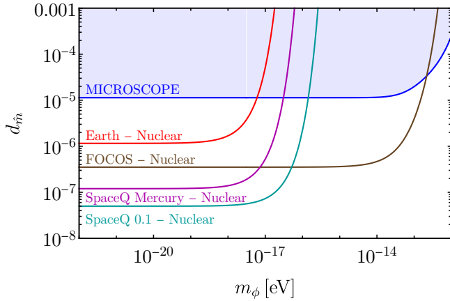
FIG. 9: In the d_m vs. m_\phi plane, we show how the projected limits from future clock based experiments compare against the current bounds from direct fifth force searches. The blue region shows the parameter space excluded by the MICROSCOPE experiment [31, 67]. The red line gives the sensitivity of an Earth based two-clock experiment involving a nuclear clock, the dark brown line depicts the reach of the space based FOCOS experiment equipped with a nuclear clock while the dark magenta and dark cyan lines project the sensitivities of the space based SpaceQ experiment assuming that the satellite reaches r = 0.39\text{AU} and r = 0.1\text{AU} respectively and is equipped with a nuclear clock. We assume \Delta K_q = 10^5 and \Delta \tilde{f}/\tilde{f} = 10^{-18} for all clock pairs except for the FOCOS experiment where we assume \beta = 10^{-9} .
