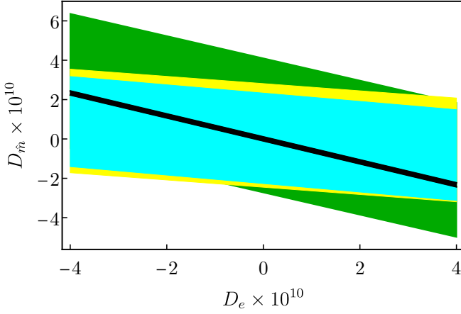
FIG. 1: Current bounds on D_e vs. D_m set by fifth force experiments [27, 30, 31, 67]. The black band represents the bound set by MICROSCOPE [31, 67], the blue and yellow bands are the constraints set by the EotWash group with Be-Ti and Be-Al masses [30], and the green band is the Moscow group's result obtained with Al-Pt masses [27].
