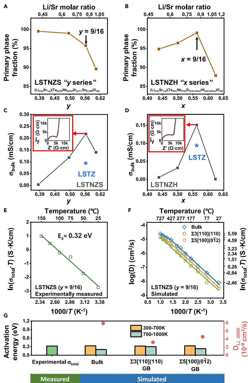
Figure 3. Plots of primary phase fraction and bulk ionic conductivity for the LSTNZS y series [(\text{Li}_{2/3y}\text{Sr}_{1-y})(\text{Ta}_{0.33x}\text{Nb}_{0.347}\text{Zr}_{0.211}\text{Sn}_{0.108})\text{O}_{3-\delta}] and the LSTNZH x series [(\text{Li}_{2/3x}\text{Sr}_{1-x})(\text{Ta}_{2/3x}\text{Nb}_{2/3x}\text{Zr}_{0.5(1-4/3x)}\text{Hf}_{0.5(1-4/3x)})\text{O}_{3-\delta}] , experimentally measured Arrhenius plot vs. simulated Li-ion diffusivities for LSTNZS ( y = 9/16 )
