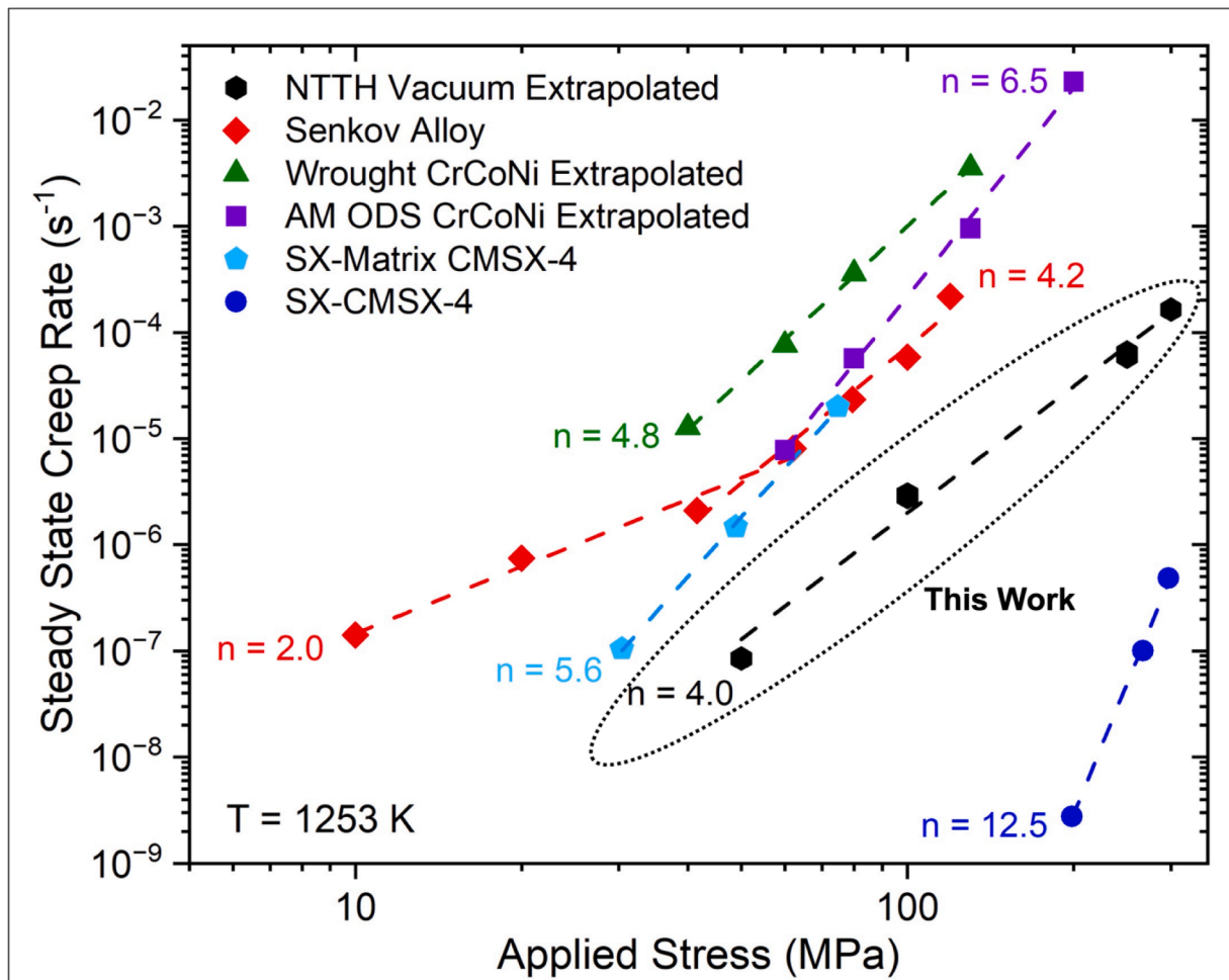
Fig. 3. Comparison of steady-state creep rates among several different types of HEAs: BCC Nb 45 Ta 25 Ti 15 Hf 15 (or NTTH investigated in this study), TaNbHfZrTi (or the Senkov alloy [13,14]), wrought FCC CrCoNi [30], additively manufactured (AM) oxide dispersion strengthened (ODS) CrCoNi [31], a commercial single crystal FCC/L1 2 two-phase Ni-based superalloy CMSX-4, as well as the FCC matrix of CMSX-4 (also a concentrated solid solution) [40]. The creep data were either reported at 1253 K or extrapolated to 1253 K using known activation energies for creep.
