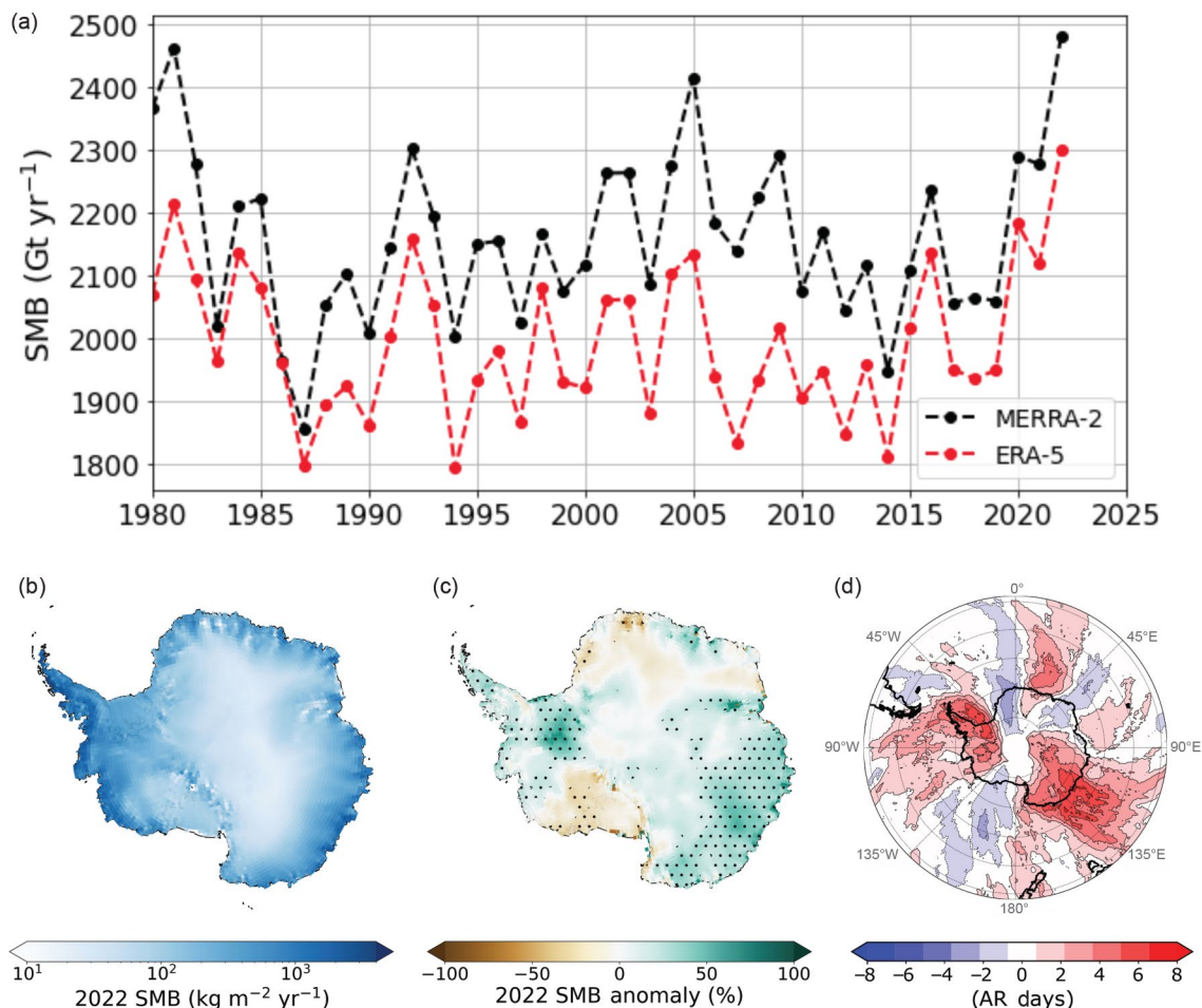
Fig. 6.5. (a) Time series of annual surface mass balance (SMB) in Gt ( 10^{12} kg) \text{yr}^{-1} . (b) MERRA-2 2022 SMB ( \text{kg m}^{-2} \text{yr}^{-1} ). (c) MERRA-2 2022 SMB anomaly relative to the 1991–2020 mean (%). The 2022 SMB anomaly is higher than the 1991–2020 standard deviation in the stippled areas. (d) 2022 atmospheric river occurrence anomaly (days) relative to the 1991–2020 mean from MERRA-2.
