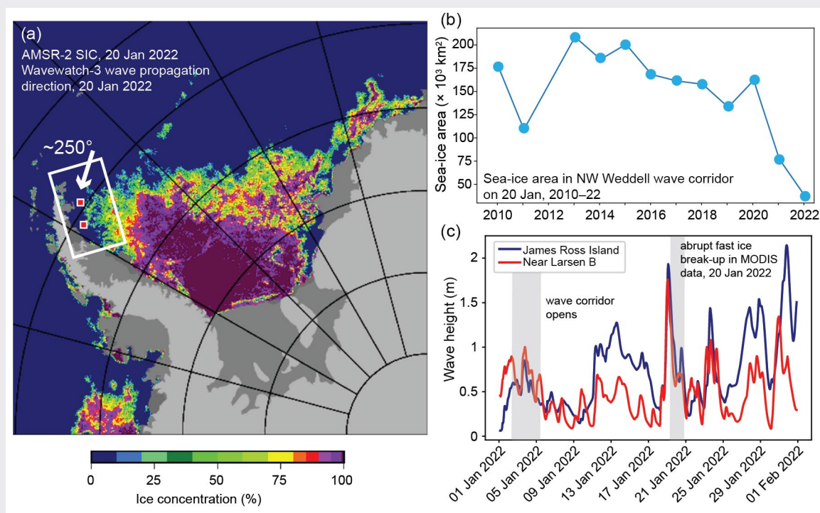
Fig. SB6.5. (a) Sea-ice conditions on 20 Jan 2022, showing ice concentration (%) and distribution from AMSR-2 data (Spreen et al. 2008; https://seaice.uni-bremen.de/sea-ice-concentration/amsr-amsr2 ). Wave propagation direction on 20 Jan from Wavewatch-3 data is shown by the white arrow (~250° true); white outline shows the region assessed for sea-ice area in (b); red squares show the location of the Wavewatch-3 wave height grid cells shown in (c); (b) sea ice area (10 3 km 2 ) from AMSR and AMSR-2 data in the corridor region of the northwest (NW) Weddell Sea for 2010–22; (c) wave height data (m) for Jan (starting at 0000 UTC on 1 January 2022) from ERA5 Wavewatch-3 gridded wave timeseries for the grid cell areas in (a).
