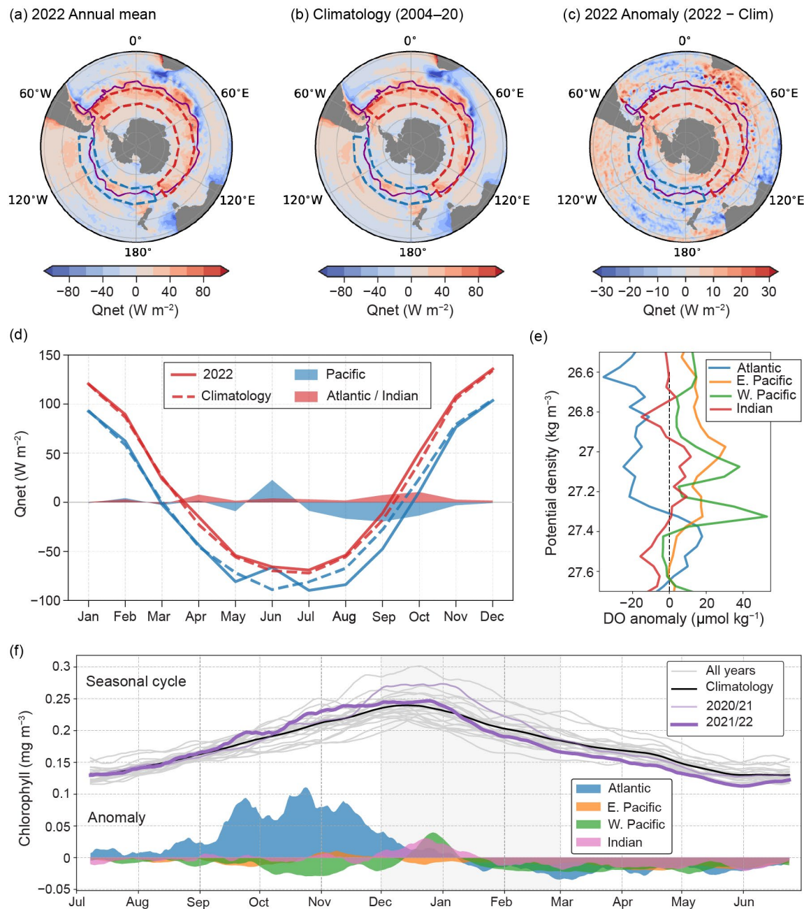
Fig. 6.14. ERA5 net heat flux, Q_{\text{net}} ( \text{W m}^{-2} ): (a) 2022 annual mean, (b) 2004–20 climatology, and (c) 2022 anomaly. The purple line denotes the location of the Subantarctic Front as in Fig. 6.13. The blue and red boxes indicate the Pacific ( 50^{\circ}\text{S} – 60^{\circ}\text{S} , 160^{\circ}\text{E} – 80^{\circ}\text{W} ) and Atlantic/Indian ( 50^{\circ}\text{S} – 60^{\circ}\text{S} , 50^{\circ}\text{W} – 150^{\circ}\text{E} ) sectors, respectively, chosen for further analysis. Positive values indicate the ocean heat gain. (d) Monthly mean net surface heat flux ( \text{W m}^{-2} ) for the Pacific (blue line) and Atlantic/Indian (red line) sectors of the Southern Ocean during 2022 (dashed) and the 2004–20 climatology (solid). Shading shows the 2022 anomaly from the climatology. (e) Jul 2021–Jun 2022 dissolved oxygen anomalies ( \text{kg m}^{-3} ) relative to the 2005–20 Argo climatology. Potential density was calculated from pressure, temperature, and salinity data, and binned into 0.05 \text{ kg m}^{-3} intervals. (f) Seasonal cycle of the area-weighted ( 40^{\circ}\text{S} – 65^{\circ}\text{S} ), daily mean chlorophyll concentration ( \text{mg m}^{-3} ): all historical years (gray lines); the climatological mean for 1997–2022 (black line); the most recent two growing seasons (purple lines); anomalies relative to climatological mean for each basin (colored shading). A 14-day rolling average was applied to all time series. The x-axis is centered on the austral summer months. (Source: data are derived from the multi-satellite merged, cloud-free product; https://doi.org/10.48670/moi-00281 .)
