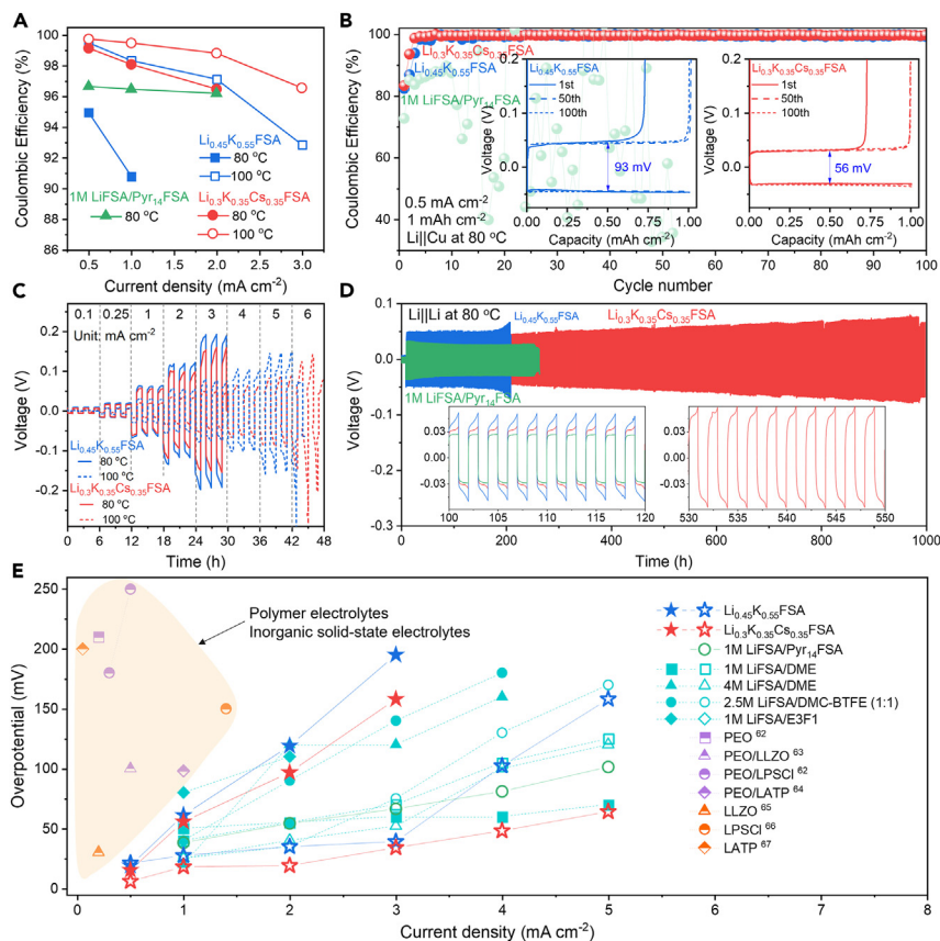
Figure 4. Lithium-metal cycling
