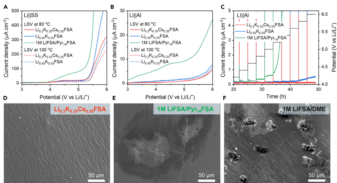
Figure 3. Oxidative stability
