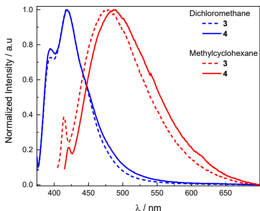
Figure 3. Normalized luminescence spectra in dichloromethane (blue) and methylcyclohexane (red) of 3 (dotted lines) and 4 (solid lines) ( [c] \sim 10^{-5} M) at 298 K.
