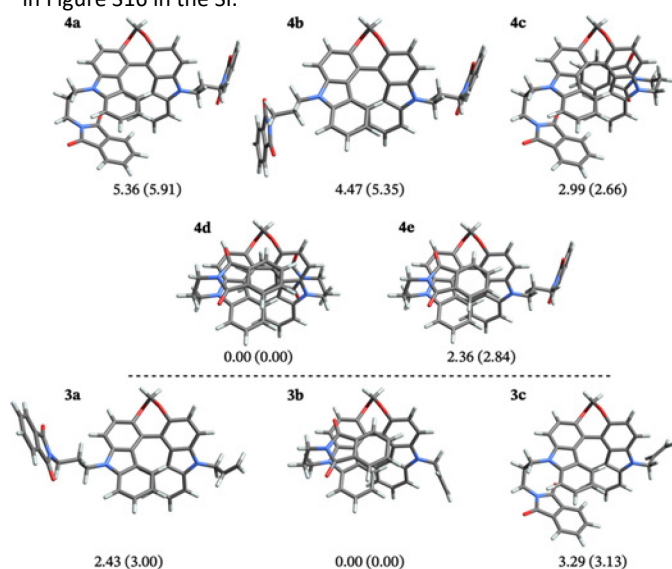
Figure 5 Conformers investigated for the disubstituted bicarbazole unit 4 (top) and the monosubstituted compound 3 . The numbers are relative Gibbs free energies for DCM (MCH) solvent in kcal/mol. The structures shown are from the DCM calculations.
