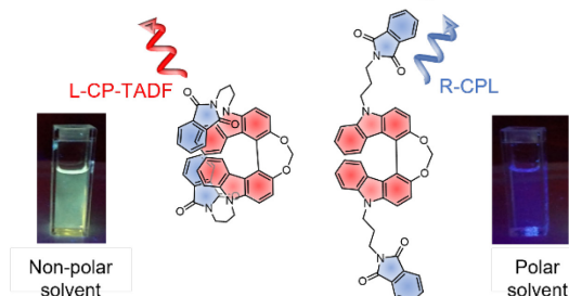
Figure 1. Top: Examples of chiral systems showing CPL sign inversion via excimeric formation (Ref. 17) and positive solvatochromism (Ref. 19). Bottom: Chemical structures of one of the new exciplex emitters, 4 , reported in this study with the schematic illustration of their CPL sign (blue and red for right- and left-CPL, respectively), and the picture of their emission colours in non-polar and polar solvents.
