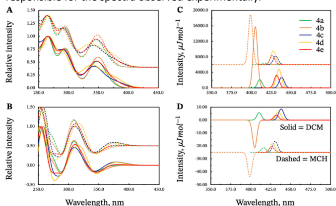
Figure 7 Calculated absorption (panel A), ECD ( P configurations, panel B), emission (panel C), and CPL ( P configurations, panel D) spectra for the five conformers of compound 4 in DCM (solid lines) and in MCH (dashed lines). The calculated energies were shifted as explained in the text.
