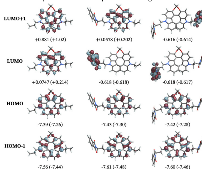
Figure 6 Isosurfaces ( \pm 0.04 au) of the relevant frontier molecular orbitals of (left to right) a dipropyl-substituted biscarbazole, 3a , and 4b . The numbers are orbital energies in eV for DCM (MCH) solvent. The orbitals shown are from the DCM calculations.
