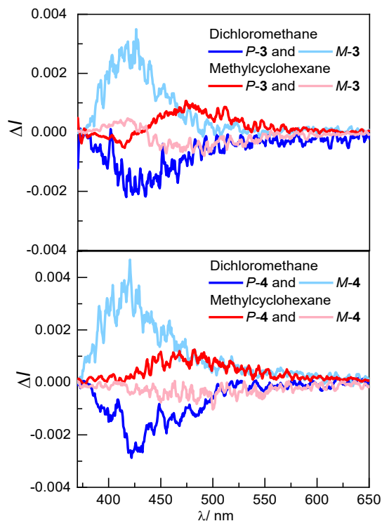
Figure 4. CPL spectra in dichloromethane (blue) and methylcyclohexane (red) of a) P-3 and M-3 and b) P-4 and M-4 ( \sim 10^{-5} M) at 298 K.
