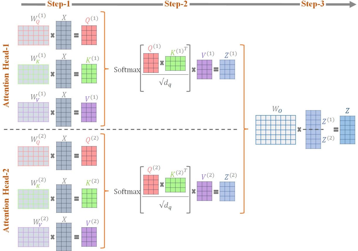
Figure 5: Multi-head attention steps. The example consists of two heads, and the input sequence comprises of three words. The input \{x_i\}_{i=1}^n is mapped to word embedding, and positional encoding vectors are added, resulting in the input matrix X \in \mathbb{R}^{6 \times 3} . Two sets of query, key, and value matrices, Q^{(l)} , K^{(l)} , and V^{(l)} \in \mathbb{R}^{4 \times 3} ( l = 2 ), are constructed corresponding to each attention head. The self-attention operation applied on both sets of query, key, and value matrices produces output matrices Z^{(1)} and Z^{(2)} \in \mathbb{R}^{4 \times 3} . A linear operation, involving a learnable parameter W_O \in \mathbb{R}^{d \times rs} , follows the concatenation of Z^{(1)} and Z^{(2)} to map it to the same dimension as input matrix X . Output matrix Z \in \mathbb{R}^{6 \times 3} accumulates information from all the attention heads.
