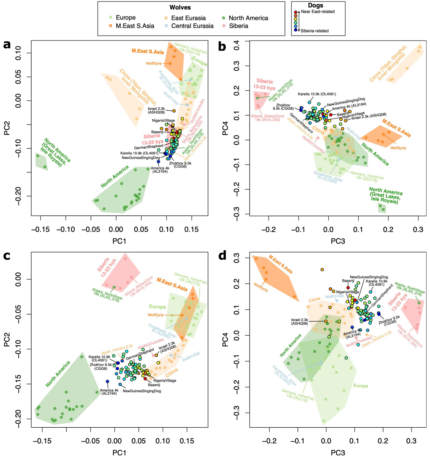
Extended Data Fig. 2 | Placing dogs into wolf diversity in a 'pre-LGM' PCA. PCA on wolves that lived after 25 ka (including present-day), based on profiles of f_4 -statistics only of the form f_4(X, A; B, C) , where A, B, and C are wolves that lived prior to 28 kya. Dogs are projected. Dogs are coloured according to the f_4 -statistic f_4(\text{AndeanFox}, X; \text{Zhokhov dog } 9.5\text{ka}, \text{Tel Hreiz dog } 7.2\text{ka}) , with negative values going towards blue and positive values towards red. A few wolves
