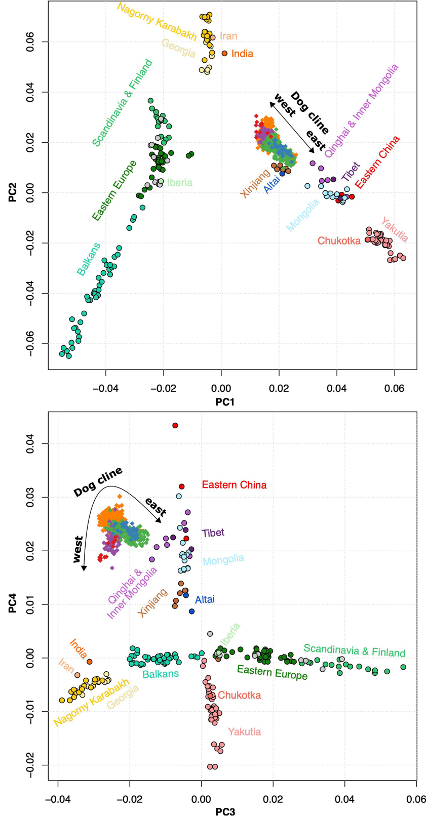
Extended Data Fig. 5 | Projecting dogs onto present-day wolf population structure. Principal components analyses performed only on modern wolves, with modern dogs projected.
