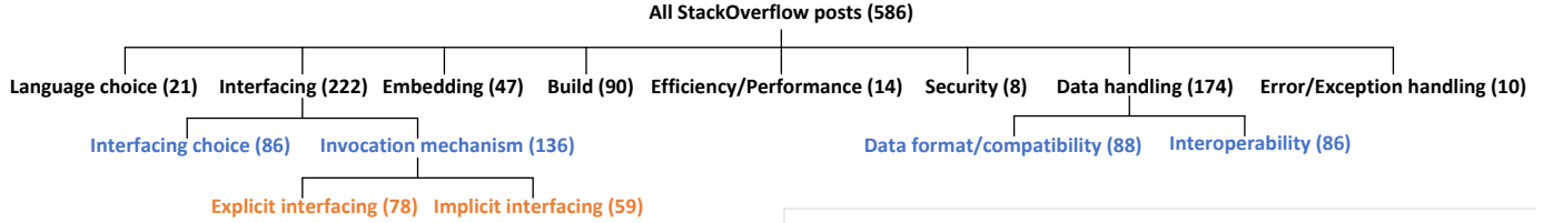
Fig. 4: Our proposed taxonomy of multilingual development
