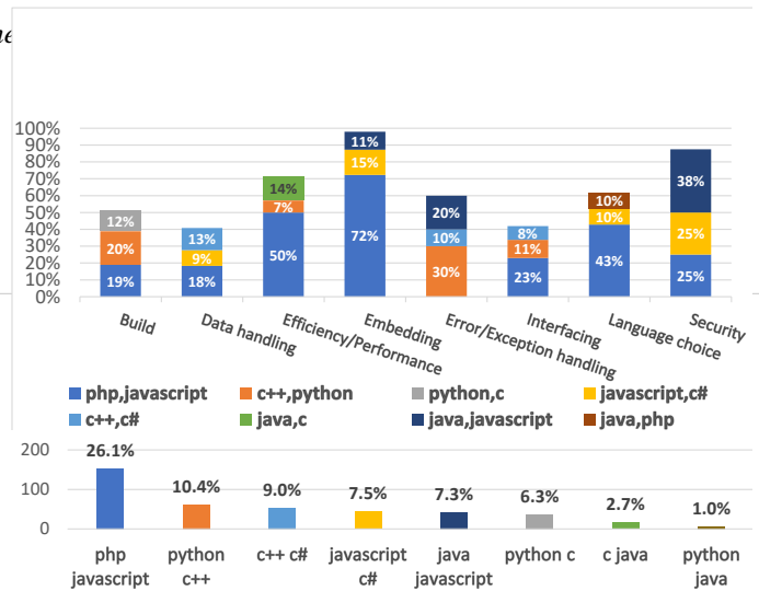
Fig. 5: The percentage distribution of top three language combinations involved in the posts of each issue category (top), and the percentage distribution of all the 586 posts over all such language combinations (bottom). The bottom chart serves as a reference for better understanding the top chart.
