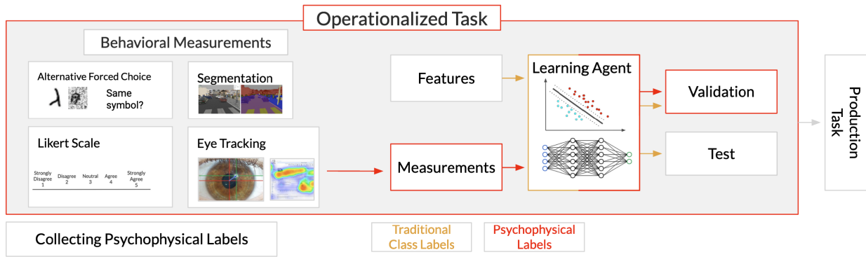
Fig. 1. When performing similar visual tasks, humans and machine agents both solve for some latent representation of features. However, at present, the human capacity for this is superior. The central component of psychophysically informed learning is collecting quantifiable latent information from human experiments on visual recognition tasks and augmenting the training regime of machine learning models with it. A learning agent with a closer representational space to humans for a visual task, which is in part learned from the psychophysical measurements, solves that task in a way that is better than an agent without access to those measurements.
