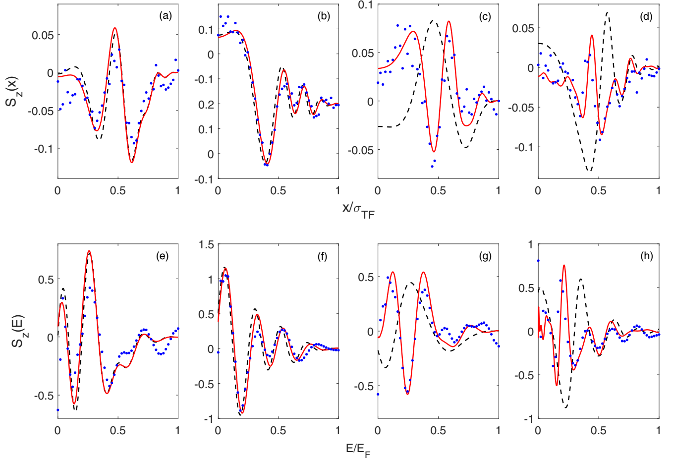
FIG. 4. Single-shot spin-density profiles in space (top) and in energy space (bottom) for perturbed quantum rewinding. For this set of data, \sigma_{\text{TF}} \approx 340 \text{ } \mu\text{m} , (a), (e) measured scattering length a = 5.2a_0 , \phi_x = \pi/2 , \tau = 200 \text{ ms} ; (b), (f) a = 5.2a_0 , \phi_x = \pi , \tau = 200 \text{ ms} ; (c), (g) a = 8.0a_0 , \phi_x = 3\pi/2 , \tau = 200 \text{ ms} ; (d), (h); a = 5.2a_0 , \phi_x = \pi/2 , \tau = 400 \text{ ms} . Blue dots are single-shot data. Red curves: Quasiclassical collective spin vector model using the measured scattering length, with forward and backward evolution phases \varphi_f and \varphi_b as fit parameters. Black dashed curves show the fits using the analysis method of Ref. [20], which requires a_{\text{fit}} = 9.0a_0 for (a), (e) and (b), (f). Black dashed curves in (c), (g) and (d), (h) show typical fit failures for the same method.
