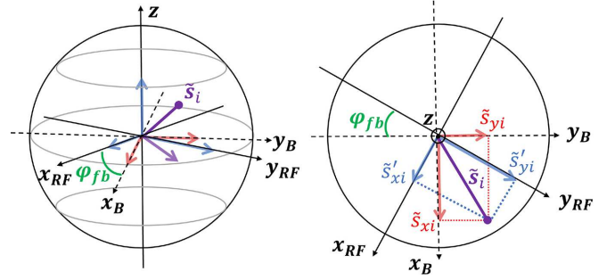
FIG. 3. Relation between the spin vector components in the radio-frequency (rf) and Bloch (B) frames for nonzero \varphi_{fb} .
