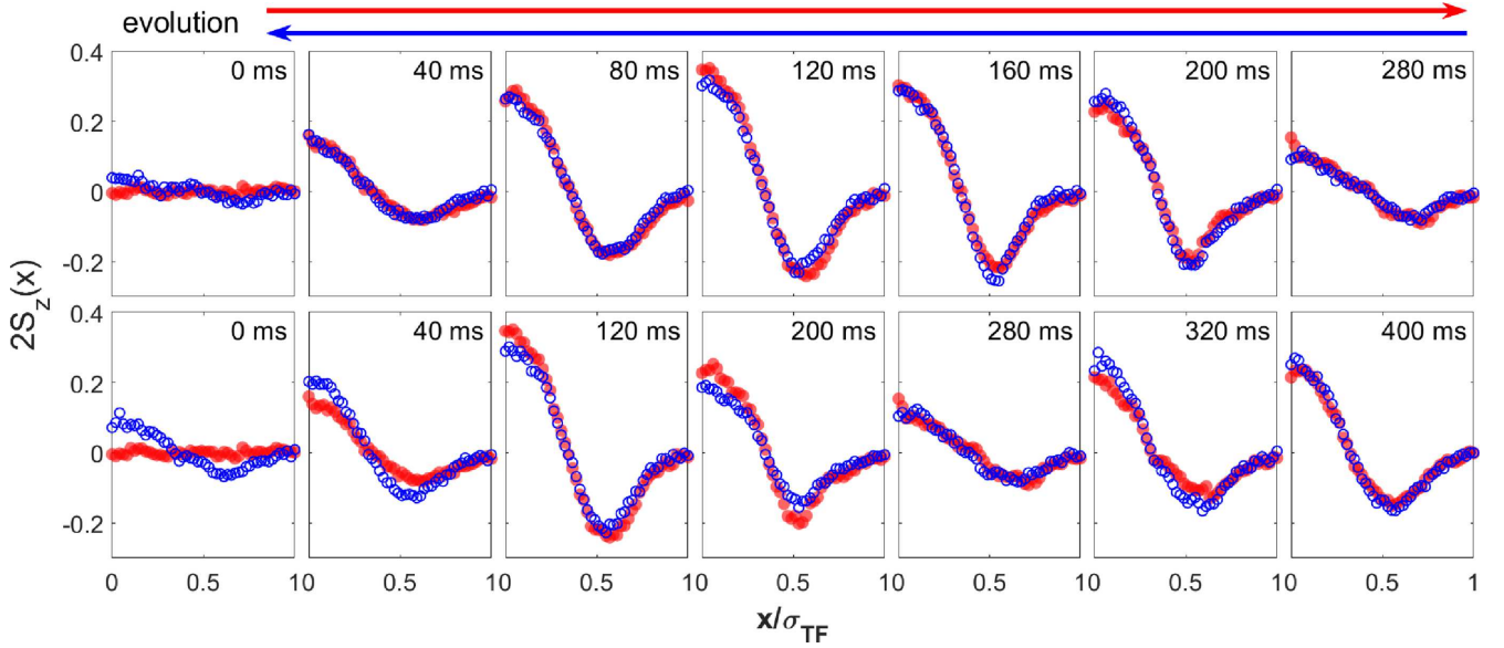
FIG. 1. Observing quantum rewinding by comparing the spin densities for forward evolution (red circles) and backward evolution (blue circles). The scattering length a = 8.0a_0 and \sigma_{\text{TF}} \approx 335 \mu\text{m} . The Hamiltonian is reversed at \tau_f = 280 \text{ ms} (top) and \tau_f = 400 \text{ ms} (bottom). For forward evolution data, the time t_k shown on the top right corner of each tile is the total evolution time t_{\text{bk}} : For the backward evolution data, the total evolution time t_{\text{bk}} = \tau_f + \tau_b , where \tau_f is the time at which reversal occurs, and \tau_b = \tau_f - t_k is the backward evolution time (see Fig. 2). To avoid confusion with the x axis of the rf or Bloch frame, here, we clarify that x in all spatial profiles means the axial direction along the longitudinal axis of the cigar-shaped cloud.
