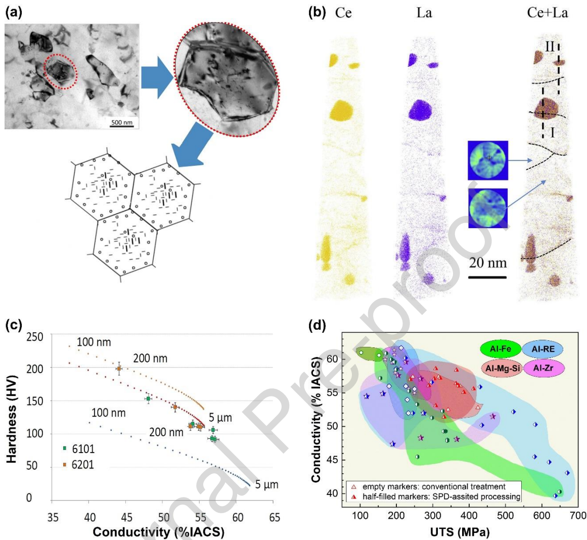
Fig. 69. (a) A strategy to improve the strength-conductivity ratio in age-hardenable aluminum alloys by SPD-controlled nano-precipitation [832]. (b) Grain boundary segregations in SPD-processed immiscible Al-RE (RE: rare earth) alloys [1520]. (c) A theory-based predictive approach to define limits of the hardness-conductivity trade-off in UFG Al-Mg-Si alloys as a function of the grain size and with 0.2 wt% of solutes left in solid solution. Different curves correspond to different contributions considered for the estimations: without precipitates (blue), with precipitates with density corresponding to the conventional T6 (red), with precipitates and maximal measured dislocation density after HPT at room temperature (orange). Green and orange squares correspond to experimental data collected on the 6101 and 6201 alloys, respectively [1516]. (d) A potential of SPD to expand the space of improving the strength and conductivity of conductor aluminum alloys [832]. IACS stands for International Annealed Copper Standard [854].
