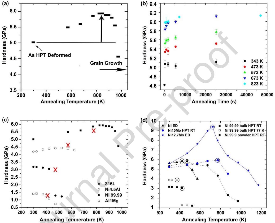
Fig. 32. (a) Hardness after isochronal (30 min) annealing of 316L steel processed by HPT at ambient temperature (grain growth occurs above 823 K) [684]. (b) Isothermal annealing of 316L steel processed by HPT for different times [691]. (c) Hardness of several nanostructured FCC materials after 30 min annealing as a function of annealing temperature (temperatures for the annihilation of lattice dislocations in high-angle grain boundaries are highlighted) [692,693]. (d) Hardness of various nanostructured nickel and Ni-Mo alloys as a function of annealing temperature (annealing time <1 hour), indicating that the temperature leading to the maximum hardness stays almost unaffected, despite large differences in grain size [687].
