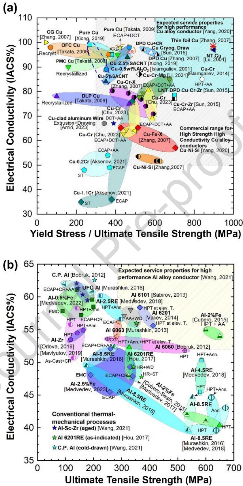
Fig. 40. Electrical conductivity with respect to strength in (a) copper and (b) aluminum alloys [831].
