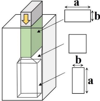
Equal channel forward extrusion (ECFE) [89]
