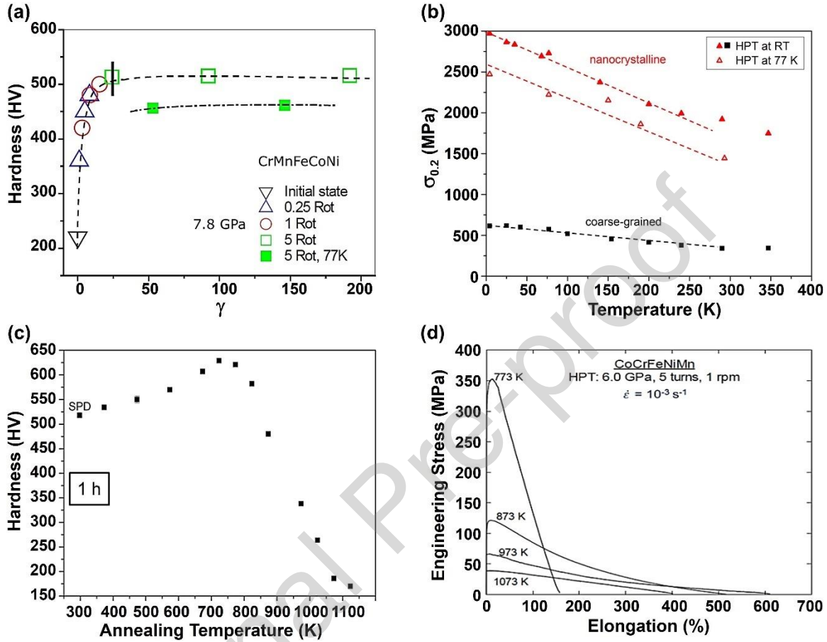
Fig. 76. (a) Room-temperature Vickers hardness as a function of shear strain \gamma after HPT processing at room temperature (open) and 77 K (full symbols) [287]. (b) Temperature dependence of the yield stress \sigma_{0.2} in nanograined Cantor alloy processed by HPT at room temperature and 77 K in comparison with coarse-grained sample [270]. (c) Vickers hardness of isochronally annealed (1 h) Cantor alloy samples after HPT processing at room temperature [500]. (d) Engineering stress-elongation curves at different temperatures for samples processed by HPT at room temperature [1644].
