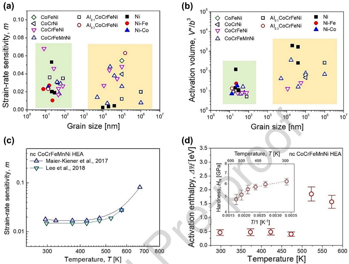
Fig. 80. Variations in (a) strain rate sensitivity and (b) activation volume of various FCC metals and alloys as a function of grain size [1668,1671,1682-1701]. (c,d) Results of high-temperature nanoindentation experiments for HPT-processed nanocrystalline CoCrFeMnNi HEA [502,1687].
