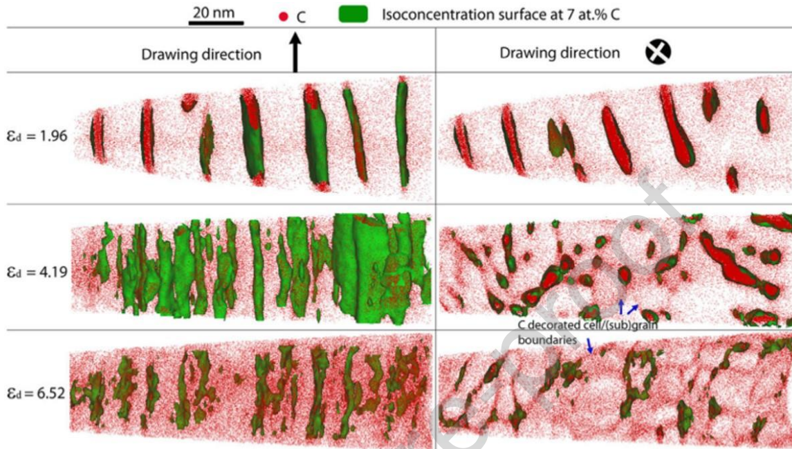
Fig. 72. Evolution from an initially lamellar structure (strain: \varepsilon_d = 1.96 ) to a ferritic subgrain structure with carbon either supersaturated in the matrix or segregated to subgrain boundaries (strain: \varepsilon_d = 6.52 ) by straining [679].
