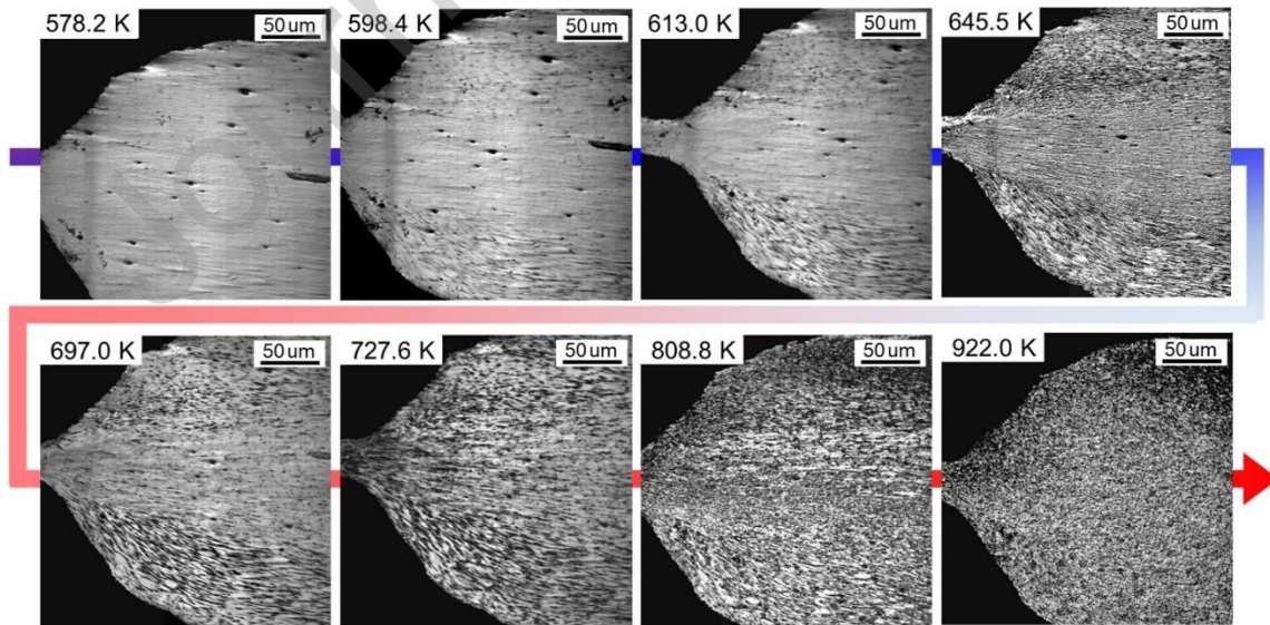
Fig. 24. A heterogeneous phase transformation observed by laser-scanning confocal microscopy (LSCM) at the cross-sections of the HPT-processed CoCrFeNiMn alloy disc edges upon heating [496].
