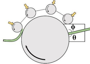
Conshearing [98]
