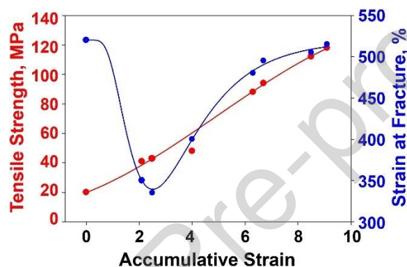
Fig. 89. Influence of the value of accumulated strain on tensile strength and strain at break of high-density polyethylene exposed to ECMAE [1854].
