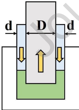
Accumulative back extrusion (ABE) [91]
