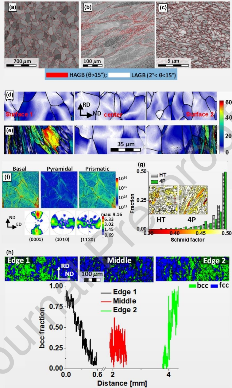
Fig. 21. (a-c) Armco iron processed by (a) zero, (b) one and (c) 16 ECAP passes [449]. (d,e) Grain reference orientation deviation (GROD) maps for interstitial free steel processed by (d) cold symmetric rolling and (e) asymmetric rolling [440]. (f) Geometrically necessary dislocations (GND) and pole figures for commercially pure titanium after two passes of equal-channel angular sheet extrusion (ECASE) [436]. (g) Schmid factor evolution for low-carbon 1020 steel after heat treatment (HT) and four ECAP passes [446]. (h) Phase maps for an austenitic stainless steel processed by one ECASE pass [434].
