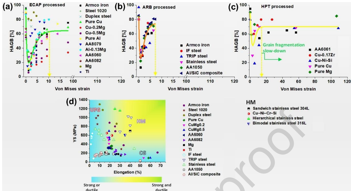
Fig. 22. High-angle grain boundary (HAGB) fractions for different metallic materials processed by (a) ECAP (Armco iron [449], steel 1020 [444], duplex steel [450], pure copper [451], Cu-0.2Mg [452], Cu-0.5Mg [452], pure aluminum [453], AA8079 [454], Al-0.13Mg [454], AA6060 [455], AA6082 [456], Mg-based alloy [457] and commercially pure titanium [458]), (b) ARB (Armco iron [459], interstitial free (IF) steel [460], TRIP (transformation-induced plasticity) steel [461], stainless steel [462], AA1050 [463] and Al/SiC composite [463]) and (c) HPT (AA6061 [464], Cu-0.17Zr [465], Cu-Ni-Si [466], pure copper [467] and pure magnesium [468]). (d) Yield strength and elongation evolution for UFG, coarse-grained and heterostructured materials (sandwich stainless steel [469], Cu-Ni-Cr-Si [470], hierarchical stainless steel [471] and bimodal stainless steel 316L [472]).
