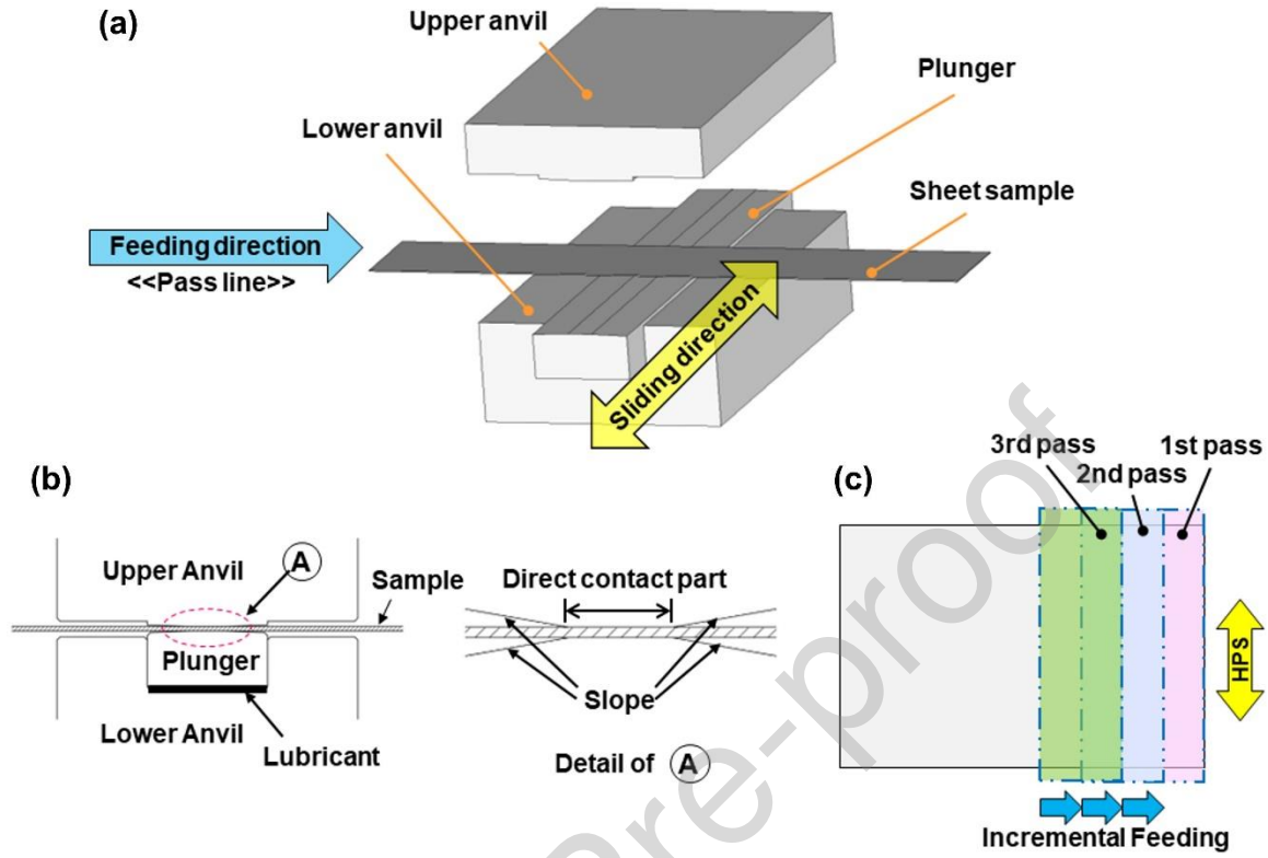
Fig. 10. (a) Schematic illustration, (b) cross-sectional view and (c) incremental feeding pattern for consecutive 1 st , 2 nd and 3 rd passes of incremental-feeding HPS [157].
