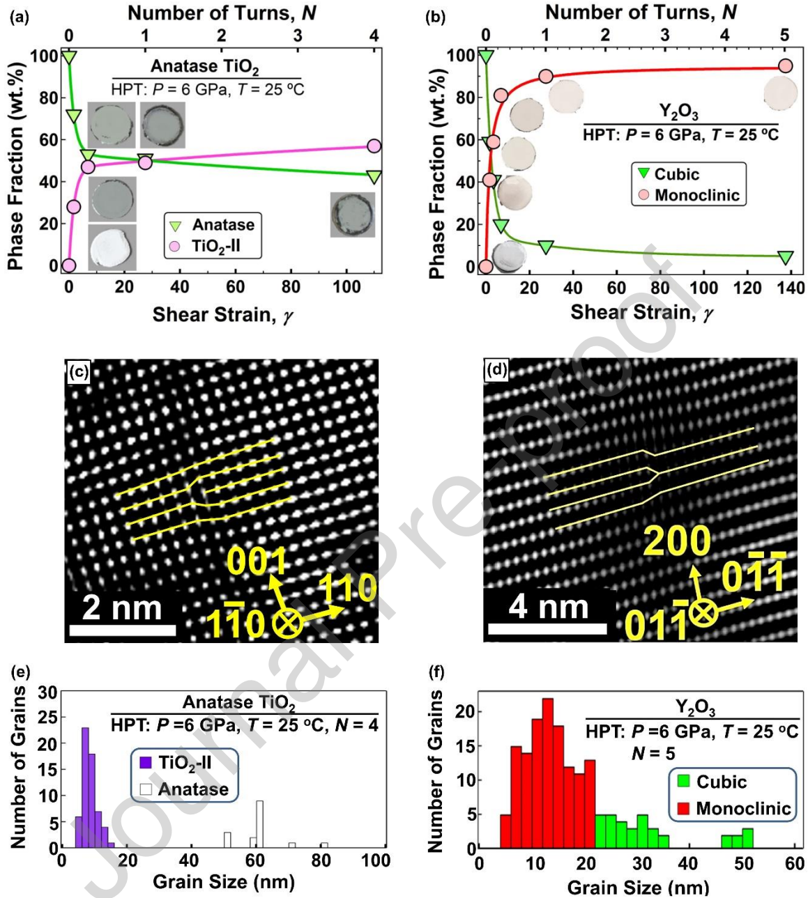
Fig. 27. (a,b) Influence of plastic shear strain on the fraction of high-pressure phases in (a) \text{TiO}_2 [579] and (b) \text{Y}_2\text{O}_3 [580] after HPT processing. (c,d) Formation of dislocations during phase transformations of (c) \text{ZrO}_2 [581] and (d) \text{TiO}_2 [579] after HPT processing. (e,f) Grain size effect on the stability of high-pressure (e) \text{TiO}_2\text{-II} [579] and (f) monoclinic \text{Y}_2\text{O}_3 [580] after HPT processing.
