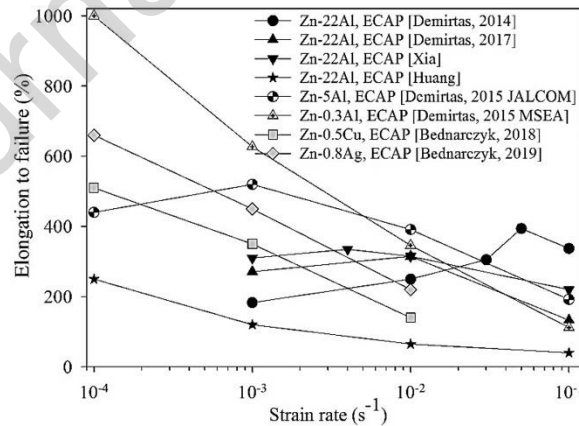
Fig. 39. Room temperature superplastic elongations of some severely deformed alloys [789].
