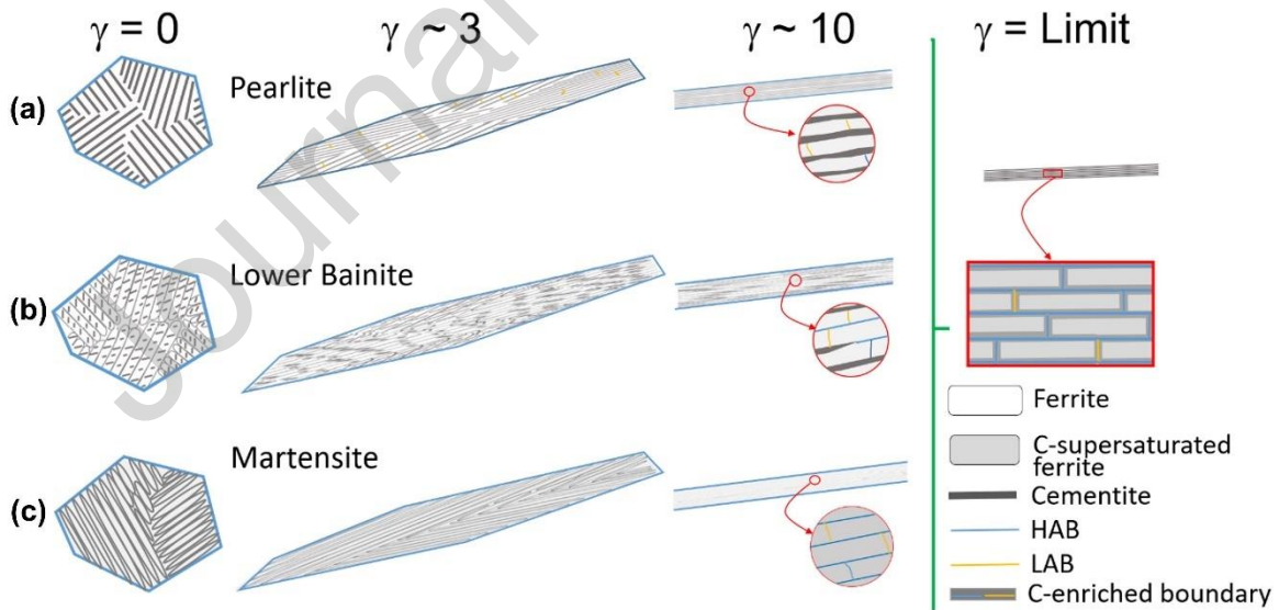
Fig. 73. Schematic illustration of the structural evolution of (a) pearlitic, (b) bainitic and (c) martensitic structures during quasi-constrained HPT deformed up to current technological limits [1580].
