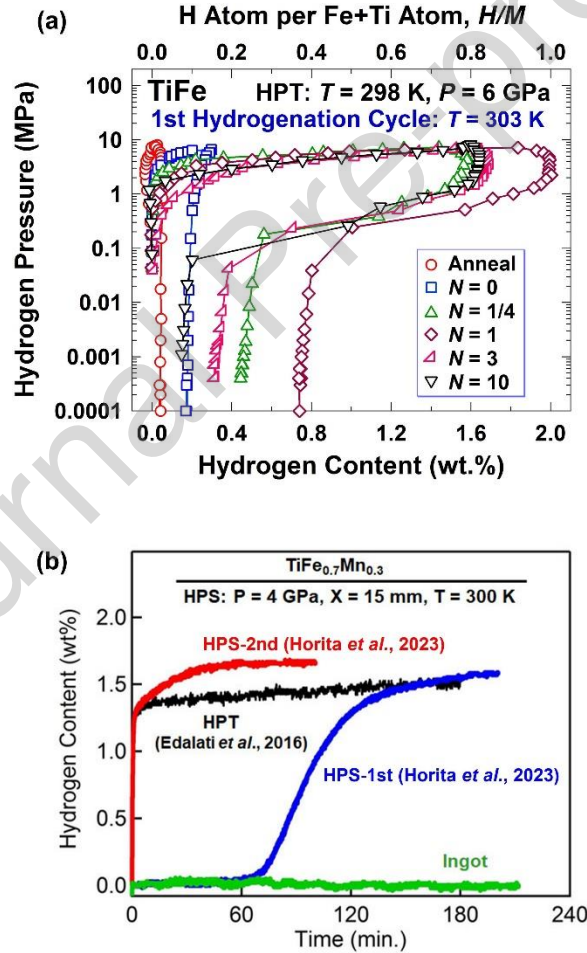
Fig. 55. (a) pressure-composition isotherms of TiFe at 303 K for annealed sample, sample processed by compression under 6 GPa ( N = 0 ) and samples processed by HPT for N = 1/4 -10 turns [1133]. (b) Variation of hydrogen content against hydrogenation time at room temperature after the first and second exposure to hydrogen under a pressure of 2 MPa for Ti-Fe-Mn intermetallic processed by HPS including as-received ingot and HPT-processed disc [1185].
