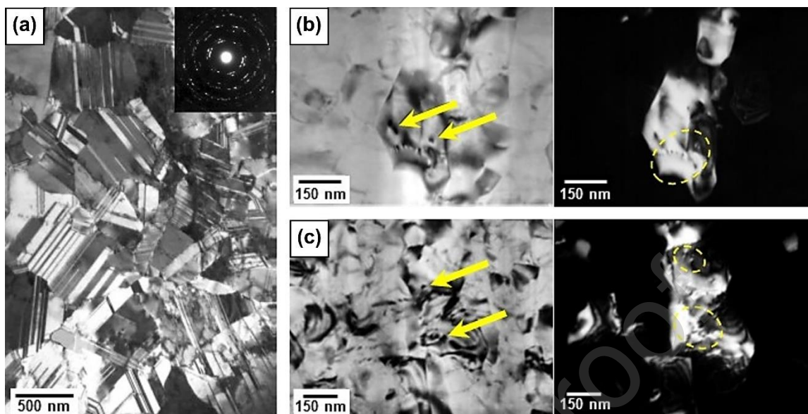
Fig. 41. (a) TEM bright-field image of as-deposited copper with diffraction pattern (as inset) [861]. (b,c) TEM bright/dark-field images of Al-2Fe (wt%) alloy after HPT processing for (b) 20 and (c) 75 revolutions at peak-aged condition [874].
