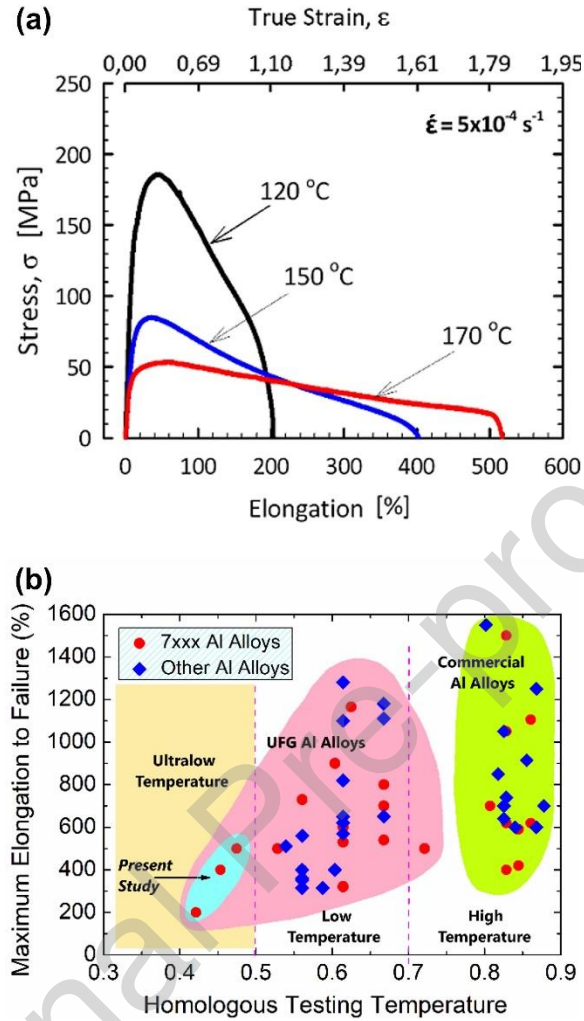
Fig. 68. (a) Deformation curves of an UFG Al-Zn-Mg-Zr (7xxx) alloy, showing a record total elongation higher than 500% at 443 K (homologous temperature: 0.47) [809]. (b) Significance of the UFG structure having grain boundaries segregated by solute atoms, resulting in ultralow-temperature superplasticity in the Al-Zn-Mg-Zr alloy (denoted as Present Study) [809].
