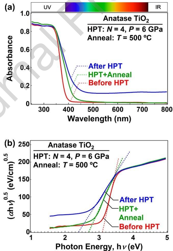
Fig. 44. (a) UV-Vis absorbance spectra and (b) bandgap calculation by the Kubelka-Munk theory for TiO 2 before and after HPT processing and after HPT followed by annealing [636].
