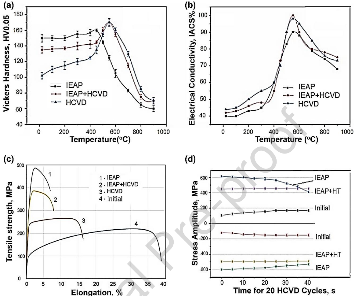
Fig. 13. (a) Variation of Vickers hardness versus aging temperature and (b) electrical conductivity versus aging temperature, (c) tensile strength versus elongation and (d) experimental values of stress amplitudes obtained during HCVD testing for 20 cycles at a frequency of 0.5 Hz and a strain amplitude of \pm 1\% for Cu-0.66Cr-0.03Si-0.02Fe-0.016S (wt%) alloy processed under different conditions (initial coarse-grained sample, SPD by indirect extrusion angular pressing IEAP and SPD followed by heat treatment at 723 K IEAP+HT) [264].
