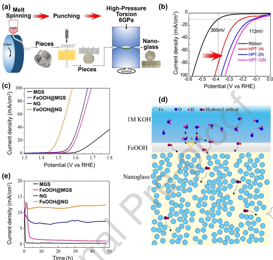
Fig. 49. (a) Schematic illustration for the fabrication of Fe 78 Si 9 B 13 nanoglass alloy [1020]. (b) Linear sweep voltammetry (LSV) curves of the Fe 78 Si 9 B 13 amorphous alloy upon HPT treatment [1020]. (c) LSV curves (iR compensation 90%) of melt-spinning glass (MSG), HPT-processed nanoglass (NG), glass covered by FeOOH (FeOOH@MSG) and nanoglass covered by FeOOH (FeOOH@NG) [1026]. (d) OER catalytic mechanism of the FeOOH@NG [1026]. (e) stability performance obtained from chronoamperometric curves of all samples at the working voltage at 10 mA cm -2 [1026].
