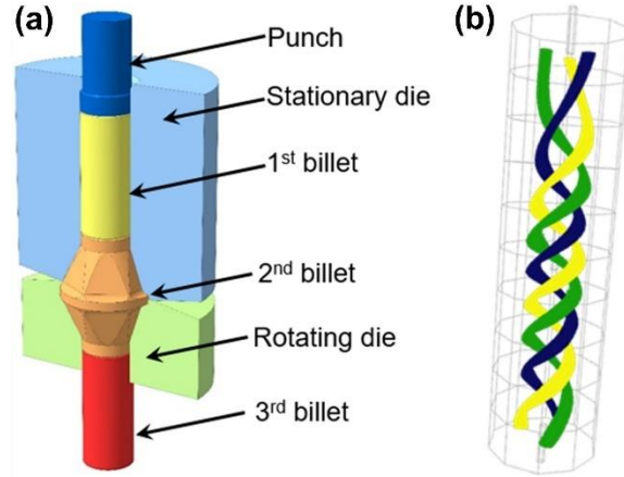
Fig. 6. (a) Schematics of the HPTE process with three billets inside the die [181]. (b) X-ray tomography reconstruction of aluminum wires embedded into the copper billet after HPTE processing with translational velocity v = 6 mm/min and rotational velocity \omega = 1 rpm (aluminum wires are shown in three different colors for better visualization) [182].
