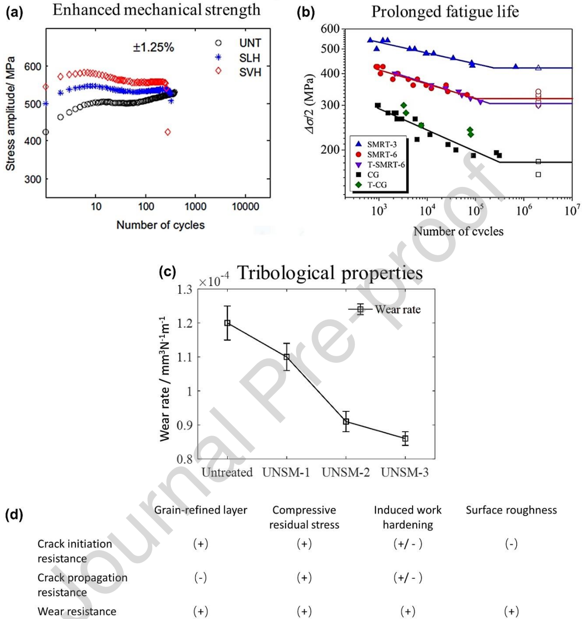
Fig. 97. (a-c) Some typical mechanical properties of gradient-structured materials including (a) low-cycle fatigue of 316L steel in different states [1992], (b) high-cycle fatigue of 316L steel in different states [125] and (c) Tribological properties of an AZ91D magnesium alloy [2009]. (d) Roles played by different parameters on fatigue and wear resistance of gradient-structured materials.
