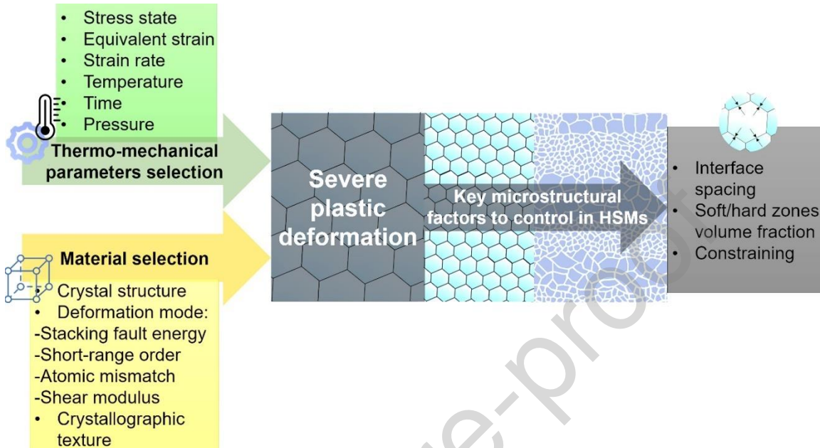
Fig. 92. Main intrinsic and extrinsic parameters to select starting materials and processing routes during the design of heterostructured materials [1883].
