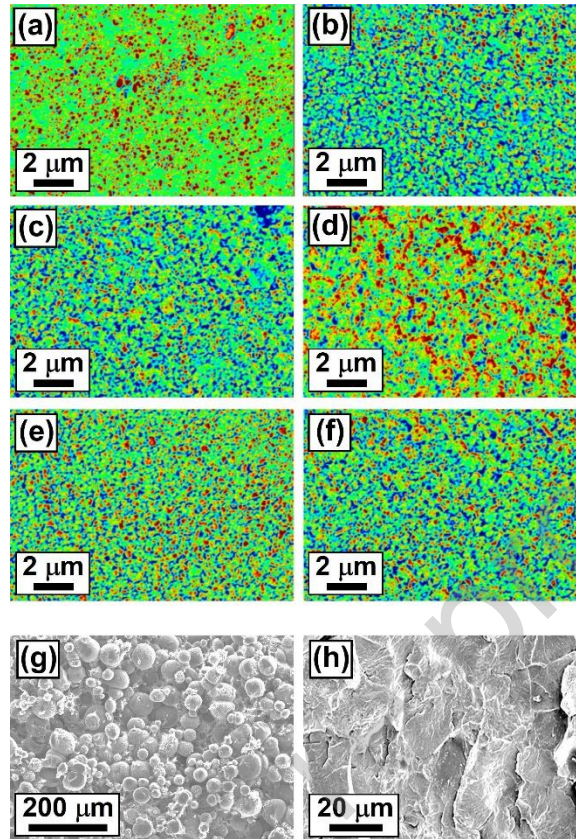
Fig. 90. (a-f): SEM micrographs of nanocomposites of LLDPE polymer with (a-c) 10 wt% of carbon nanotubes and (d-f) 20 wt% of carbon nanotube addition, after true strains of (a,d) e = 0 , (b,e) e = 4.4 , (c,f) e = 8.5 [1861]. (g,h) Morphologies of compacted polypropylene powders after strains of (g) e = 0 and (h) e = 8.5 [1838].
