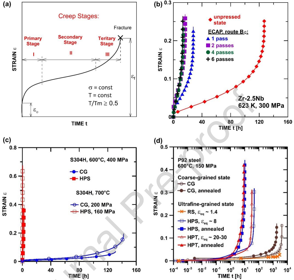
Fig. 34. (a) Schematic representation of a creep curve. (b) Creep curves for Zr-2.5Nb (wt%) cladding alloy [751]. (c) Creep curves for austenitic S304H steel [752]. (d) Creep curves for creep-resistant P92 steel with 9 wt% Cr [753].
