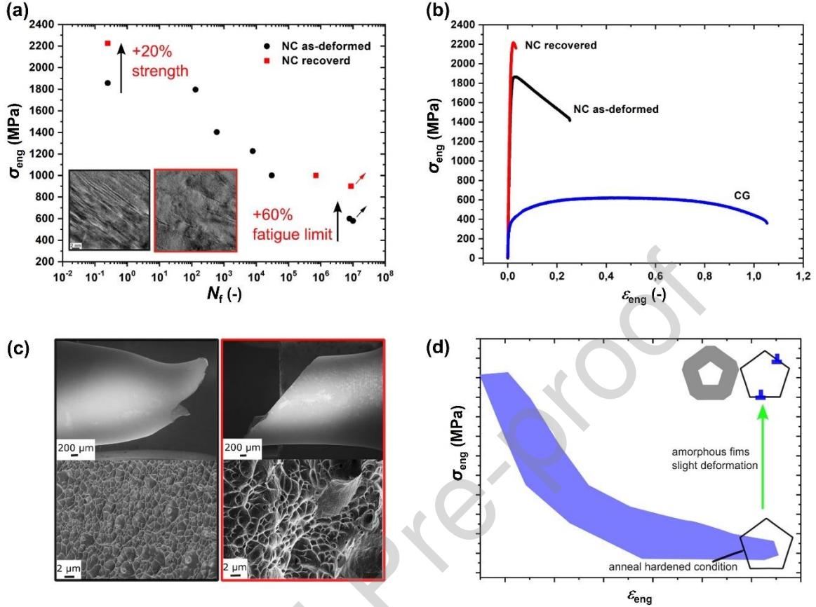
Fig. 33. (a) Fatigue S-N (stress-cycle to failure) curves showing the effect of anneal hardening (recovery) on the quasi-static strength and the fatigue limit of a nanocrystalline 316L austenitic steel prepared by HPT at room temperature [709]. (b) Representative engineering stress-strain curves of a uniaxial tensile test obtained on the same samples as in (a), indicating that anneal hardening drastically shortens the elongation to failure [709]. (c) Representative images of fractured tensile specimens and the corresponding fracture surfaces of a nanocrystalline 316L steel in HPT-processed (black) and anneal-hardened (red) conditions [709]. (d) Schematics showing the general problem of the strength-ductility trade-off applying especially for anneal hardened metals, and potential solutions to this problem [687].
