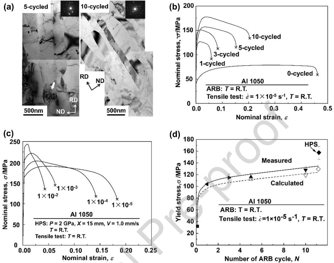
Fig. 31. (a) TEM bright-field images of aluminum after five and 10 ARB cycles. (b) Nominal stress-strain curves at a strain rate of 1 \times 10^{-5} \text{ s}^{-1} for aluminum after 0, 1, 3, 5 and 10 ARB cycles. (c) Nominal stress-strain curves with strain rates ranging from 1 \times 10^{-2} to 1 \times 10^{-5} \text{ s}^{-1} for HPS-processed aluminum. (d) Plots of yield stress against the number of ARB cycle at a strain rate of 1 \times 10^{-5} \text{ s}^{-1} , including value of HPS-processed sample and values calculated by grain boundary and dislocation hardening [672].
