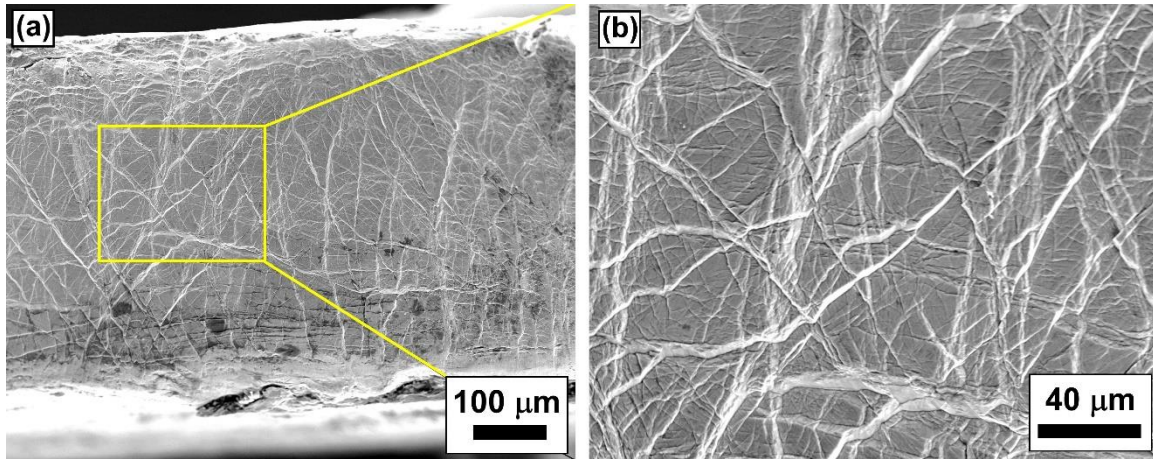
Fig. 86. (a,b) SEM images showing shear bands in a \text{Zr}_{52.5}\text{Cu}_{17.9}\text{Ni}_{14.6}\text{Al}_{10}\text{Ti}_5 metallic glass processed by HPT with 5 rotations, where (b) is a magnified view indicating formation of interacting shear band networks with increasing strain [1783].
