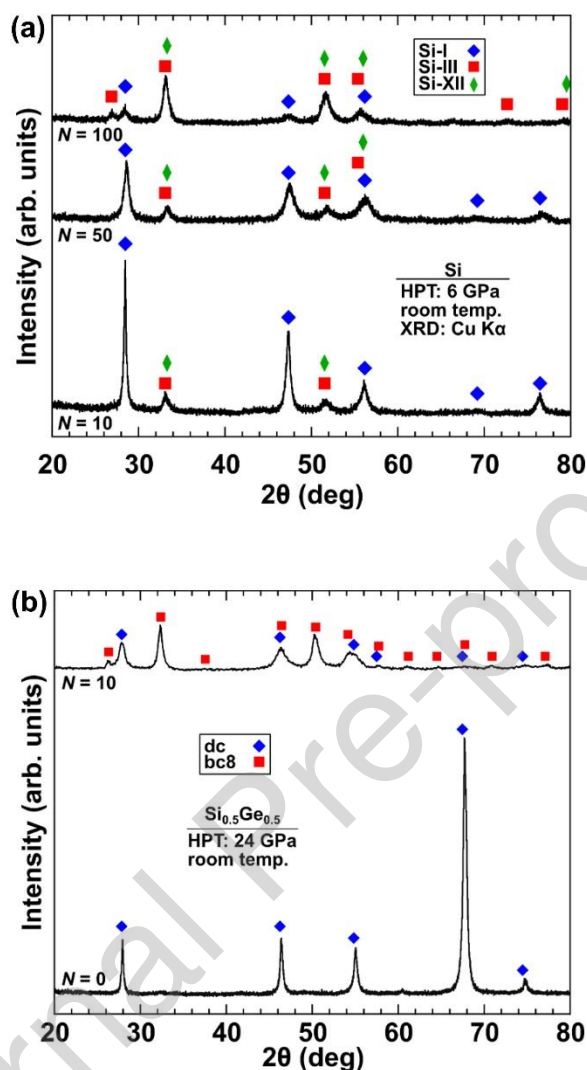
Fig. 87. XRD profiles of (a) silicon processed by HPT for different rotations ( N ) [1807] and (b) \text{Si}_{0.5}\text{Ge}_{0.5} processed by pure compression ( N = 0 ) and N = 10 turns of HPT [1809].
