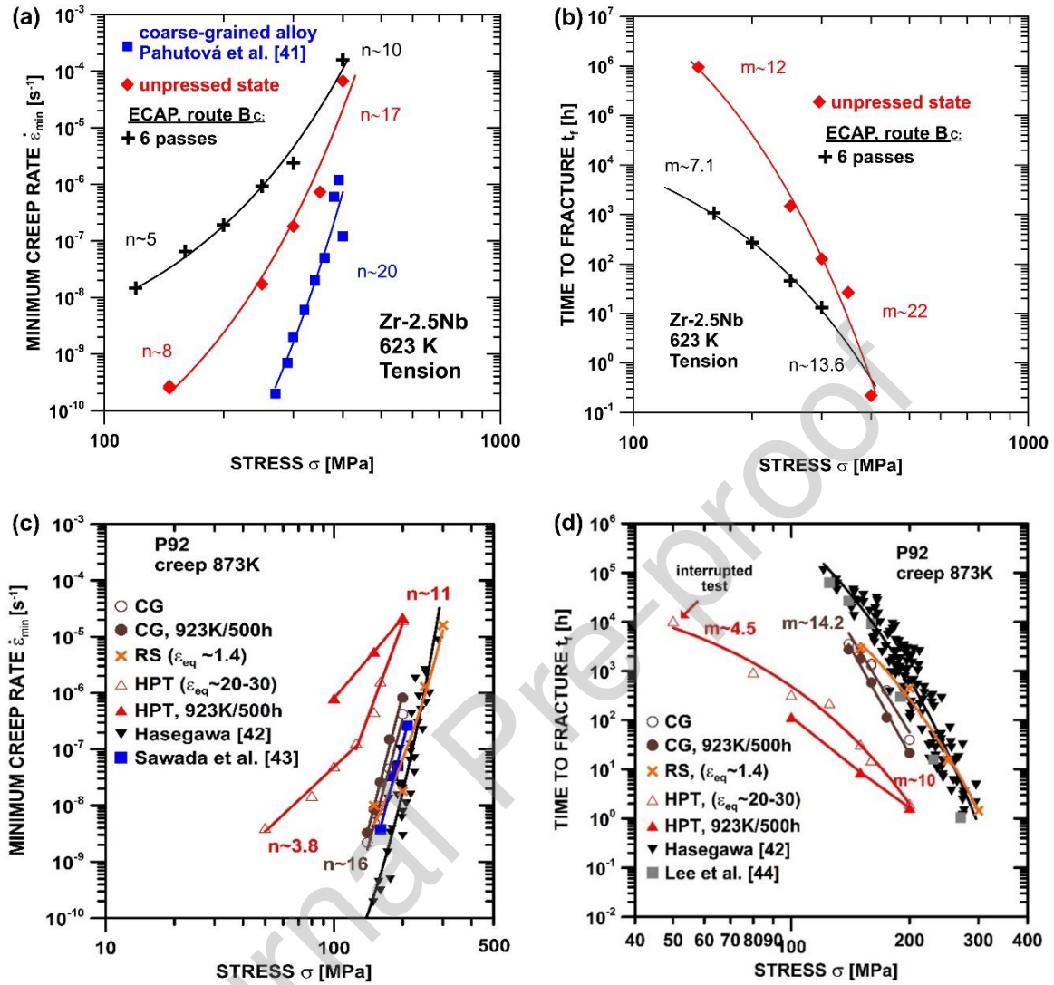
Fig. 35. Stress dependences of (a,c) the minimum creep rate \dot{\epsilon}_{\min} , and (b,d) the time to fracture t_f for (a,b) Zr-2.5Nb (wt%) alloy [751] and (c,d) P92 steel [753]. The creep results for coarse-grained materials published by Pahutova et al. [756], Hasegawa [757], Sawada et al. [758], and Lee et al. [759] are also listed.
