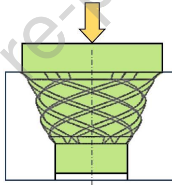
Simple shear extrusion (SSE) [83,84]
