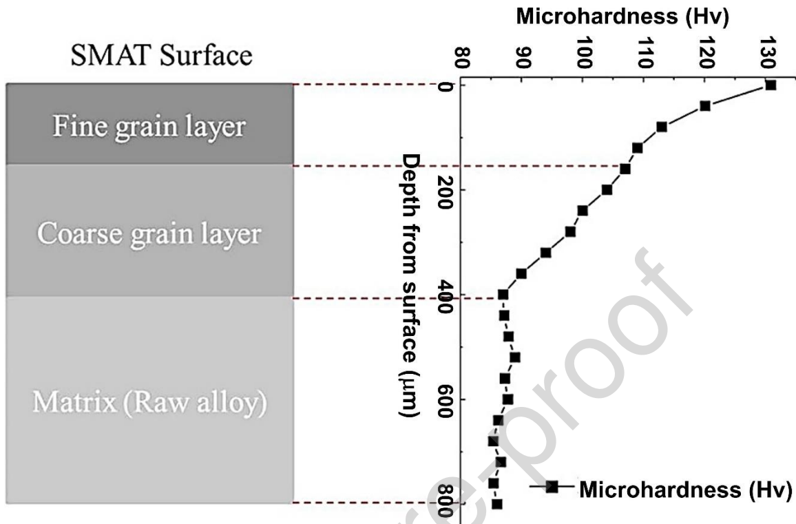
Fig. 94. Schematic diagram of gradient grain structure and corresponding microhardness of metallic samples [1946].
