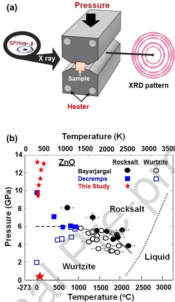
Fig. 28. (a) Schematic illustration of high-pressure application system for in situ XRD analysis at SPring-8, Japan [604]. (b) Temperature-pressure phase diagram of ZnO. Open and closed circles are reproduced from Bayarjargal and Winkler [590] for wurtzite and rocksalt structures, respectively. Open and closed blue squares are from Decremps et al. [591], representing transformation points from rocksalt to wurtzite structure and from wurtzite to rocksalt structure, respectively. Star symbols represent results of HPT-processed ZnO in which rocksalt occupies 100% [604].
