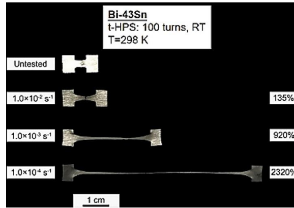
Fig. 37. Appearance of Bi-43Sn (wt%) samples after processing by t-HPS for 100 turns and pulling to failure at 298 K [221]: the elongation of 2320% exceeds the elongation of 1950% reported in early experiments by Pearson [24].
