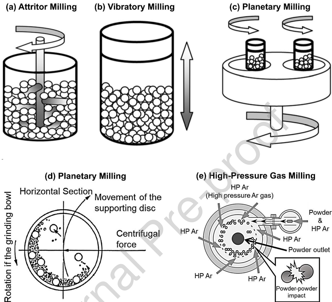
Fig. 4. Various types of high-energy ball milling for powder-SPD: (a) attritor milling, (b) vibratory milling, (c,d) planetary milling and (e) high-pressure gas milling [43,148,150].
