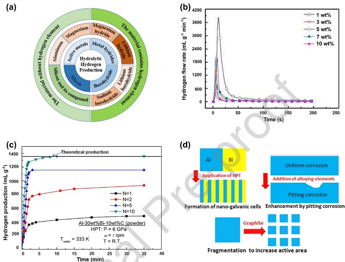
Fig. 50. (a) Materials used for hydrolytic hydrogen production [1035]. (b) Hydrolytic hydrogen flow rate curves of Al - 5 wt% LiH - x wt% Ga 2 O 3 ( x = 1, 3, 5, 7 and 10) at 298 K [1042]. (c) Hydrolytic hydrogen production curves of HPT-processed Al-30Bi-10C (wt%) composite with different HPT turns [1041]. (d) Combination of three strategies to promote aluminum hydrolysis by high-pressure torsion [1041].
