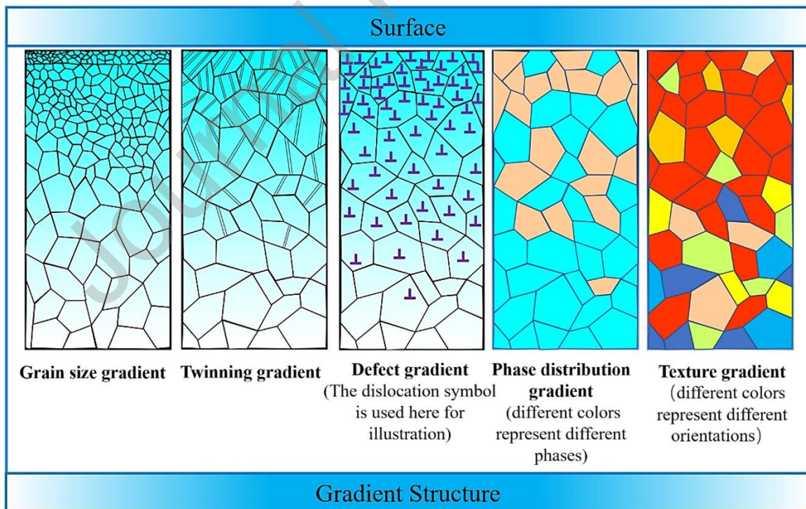
Fig. 95. Micro-schematic diagram of various gradient structures [1952].
