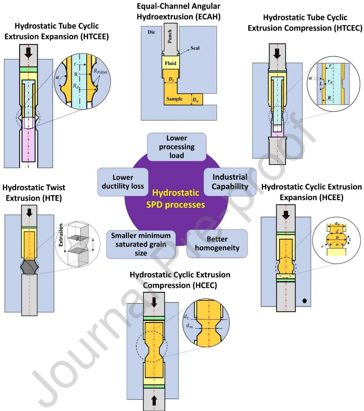
Fig. 5. Schematics of different SPD methods with high hydrostatic pressure [154].
