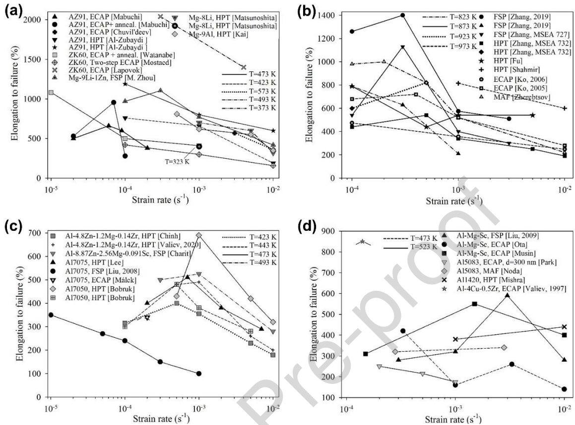
Fig. 38. The variation of superplastic elongation values with strain rate at different temperatures in severely-deformed alloys: (a) Mg-based alloys, (b) Ti-6Al-4V (wt%) alloy, (c) 7xxx series of Al-based alloys and (d) other Al-based alloys [789].
