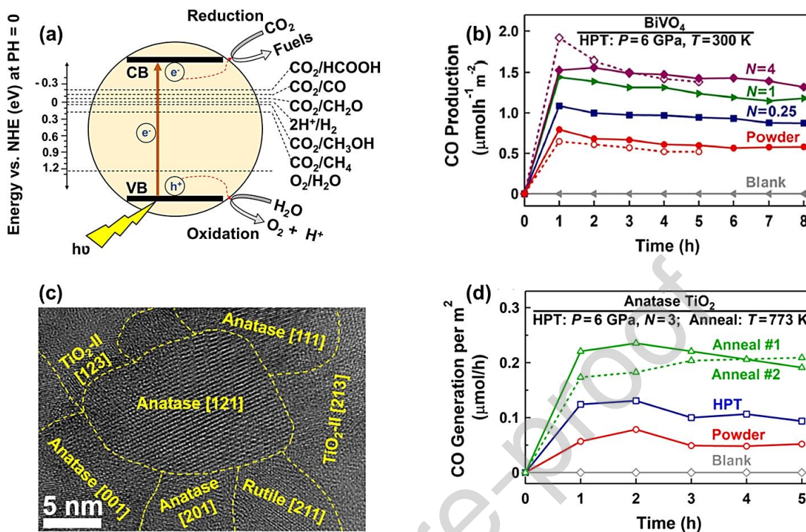
Fig. 46. (a) Schematic of photocatalytic \text{CO}_2 conversion mechanism [978]. (b) Photocatalytic CO production rate of \text{BiVO}_4 versus time for powder and samples processed by HPT with 0.25, 1 and 4 turns [958]. (c) High-resolution TEM image of sample processed by HPT containing \text{TiO}_2 -II high-pressure phase [982]. (d) Rate of CO generation for \text{TiO}_2 samples before HPT, after HPT and after HPT and annealing [982].
