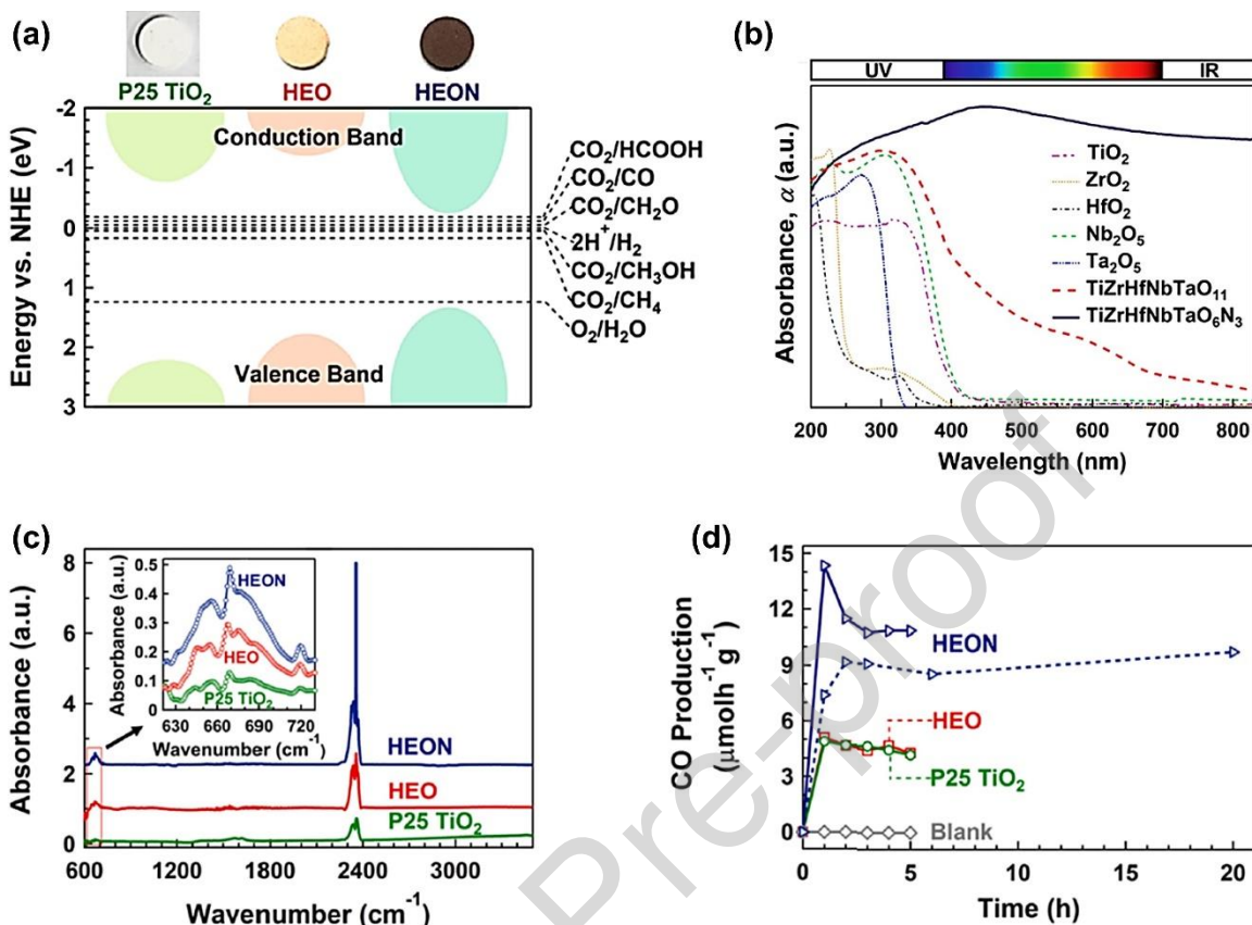
Fig. 47. (a) Electronic band structure of TiZrNbHfTaO 6 N 3 high-entropy oxynitride (HEON), P25 TiO 2 and TiZrNbHfTaO 11 high-entropy oxide (HEO) [323]. (b) UV-vis light absorbance spectra for TiZrNbHfTaO 6 N 3 compared to TiZrNbHfTaO 11 and corresponding binary oxides [322]. (c) Diffuse reflectance infrared Fourier transform spectra for TiZrNbHfTaO 6 N 3 compared to P25 and TiZrNbHfTaO 11 [323]. (d) Rate of CO production for TiZrNbHfTaO 6 N 3 compared to P25 TiO 2 and TiZrNbHfTaO 11 [323].
