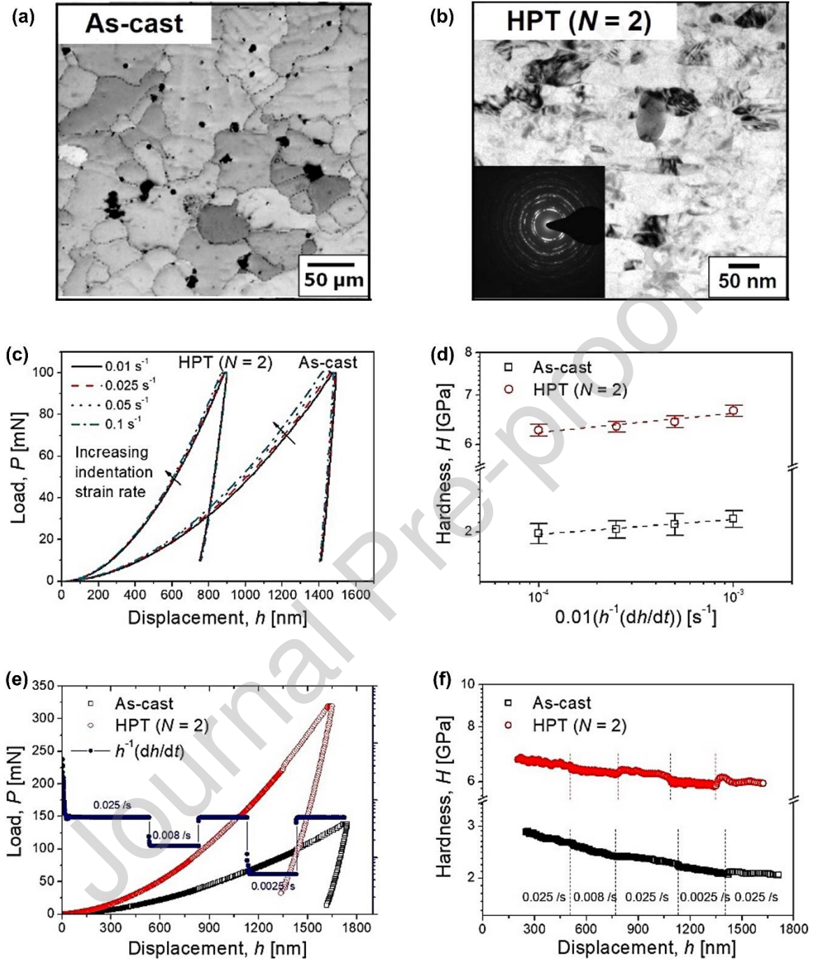
Fig. 79. Microstructures of (a) as-cast and (b) HPT-processed CoCrFeMnNi HEAs [1668] along with corresponding examples of (c,d) constant strain rate (CSR) nanoindentation [1668] and (e,f) strain rate jump (SRJ) nanoindentation [502].
