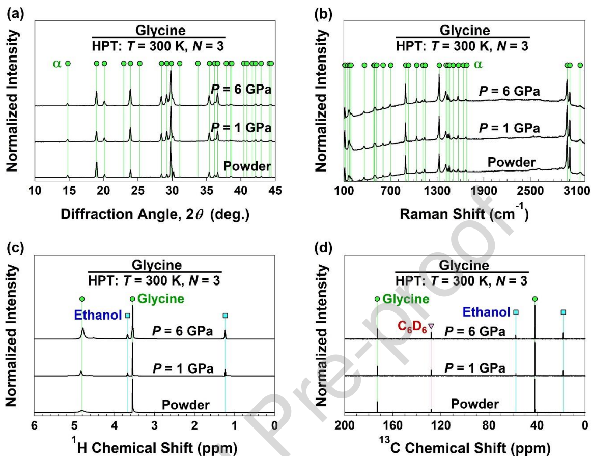
Fig. 101. (a) XRD profiles, (b) Raman spectra and (c,d) nuclear magnetic resonance spectra for glycine amino acid before and after treatment by HPT under 1 and 6 GPa [2058].
