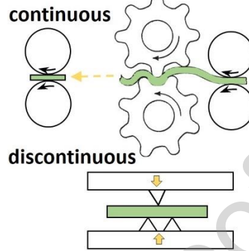
Repetitive corrugation and straightening (RCS) [94]
