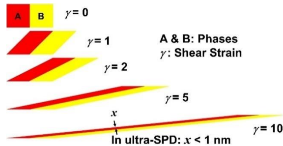
Fig. 16. Schematic illustration of ultra-SPD concept, in which severe shear strains are applied to a material so that the thickness of sheared phases is reduced to the subnanometer level [324].
