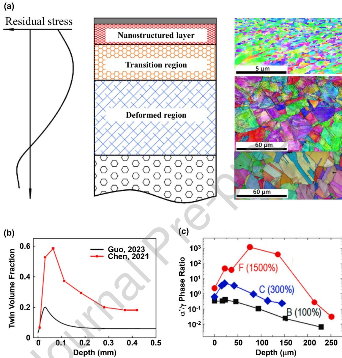
Fig. 96. Generated gradient features including (a) gradient microstructure and residual stress [1968], (b) variation of twin volume fraction [1982] and (c) distribution of phase transformation (B, C and F refer to samples processed by shot peening coverage of 100%, 300% and 1500% respectively) [1983].
