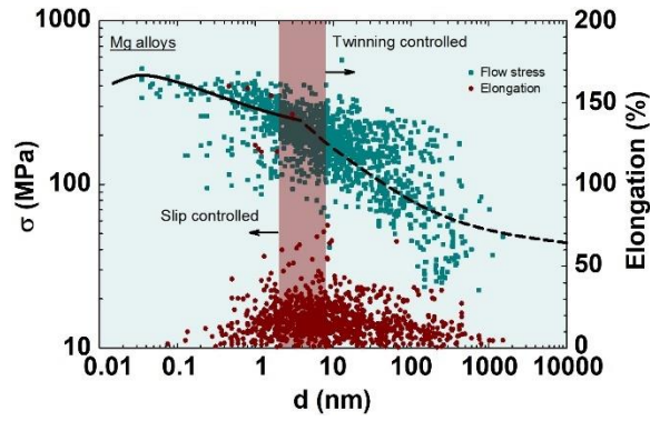
Fig. 65. Flow stress and elongation to failure of magnesium alloys plotted as a function of the grain size [1467].
