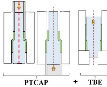
Combined parallel tubular channel angular pressing (Combined PTCAP) [106]
