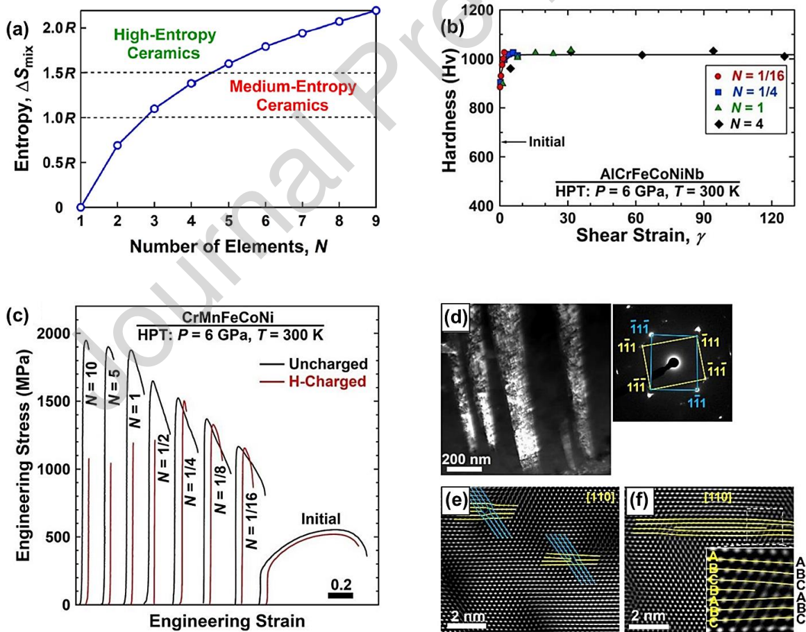
Fig. 83. (a) Entropy of mixing versus number of elements [983]. (b) Hardness of AlCrFeCoNiNb synthesized by HPT for N = 1/16, 1/4, 1 and 4 turns [1651]. (c) Engineering stress versus engineering strain before and after hydrogen exposure for CrMnFeCoNi before and after HPT
