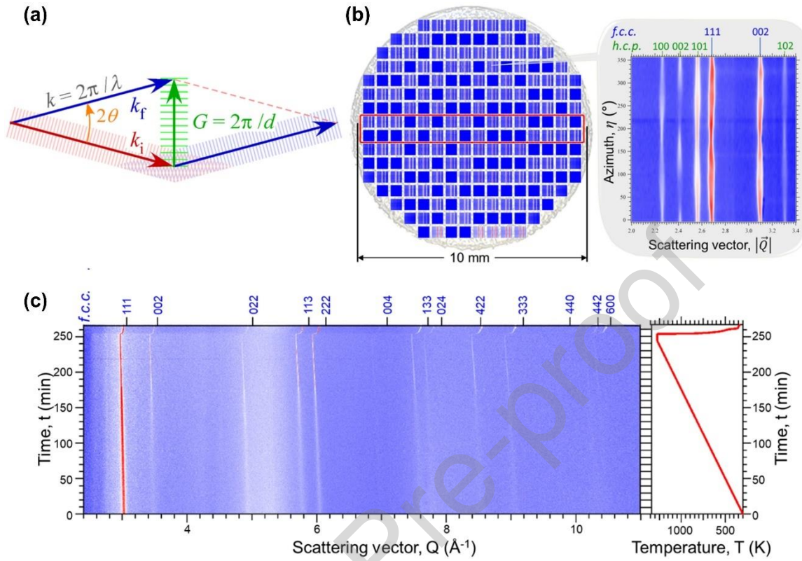
Fig. 23. (a) A portrayal of Laue–Bragg interference [473]. (b) Position-dependent microstructure map constructed by a series of high-energy XRD (HEXRD) patterns with an enlarged representative diffractogram [487]. (c) A contour plot showing neutron diffraction patterns with time and temperature [494].
