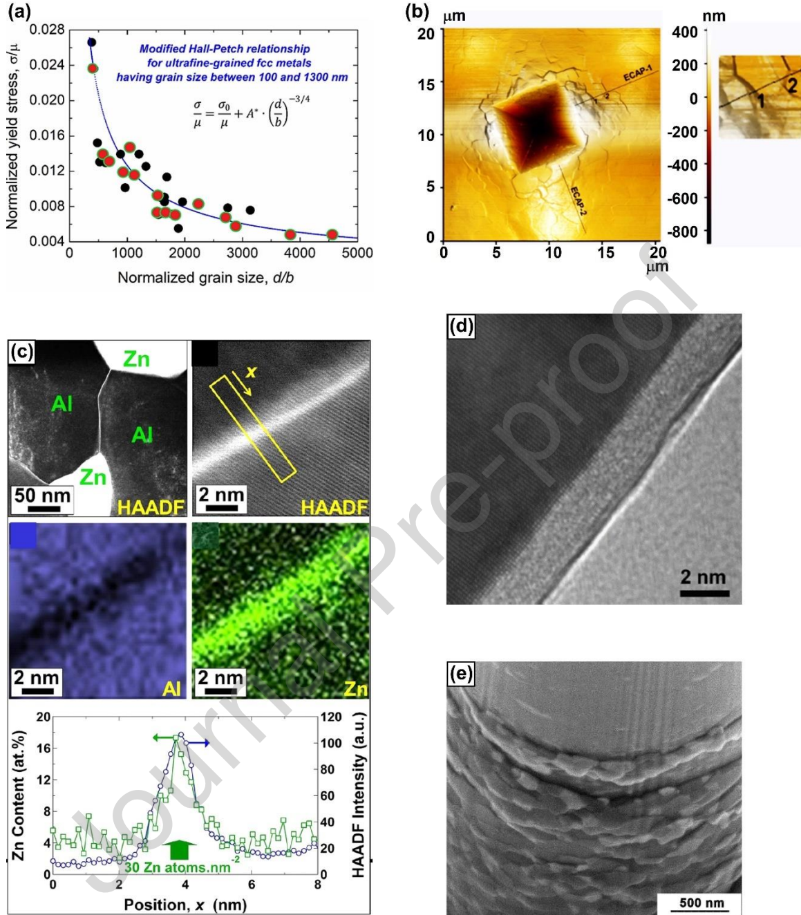
Fig. 67. (a) A possible modification of the Hall-Petch relationship for UFG FCC metals and solid solutions [1494]. (b) Evidence on grain boundary sliding at room temperature in UFG pure Al, shown by three-dimensional atomic force microscopy (AFM) [1498]. (c) The Al/Al boundaries strongly segregated by solute zinc atoms, causing wetted grain boundaries in SPD-processed Al-30Zn (at%) alloys [348]. (d) High-resolution TEM image showing a wetting layer along an Al/Al grain boundary in the HPT-processed Al-30Zn (at%) sample [1504], (e) Surface morphologies of the compressed pillars on the surface of the HPT-processed Al-30Zn (wt%) sample, demonstrating a direct evidence for the occurrence of intensive grain boundary sliding without any deformation localization [1501].
