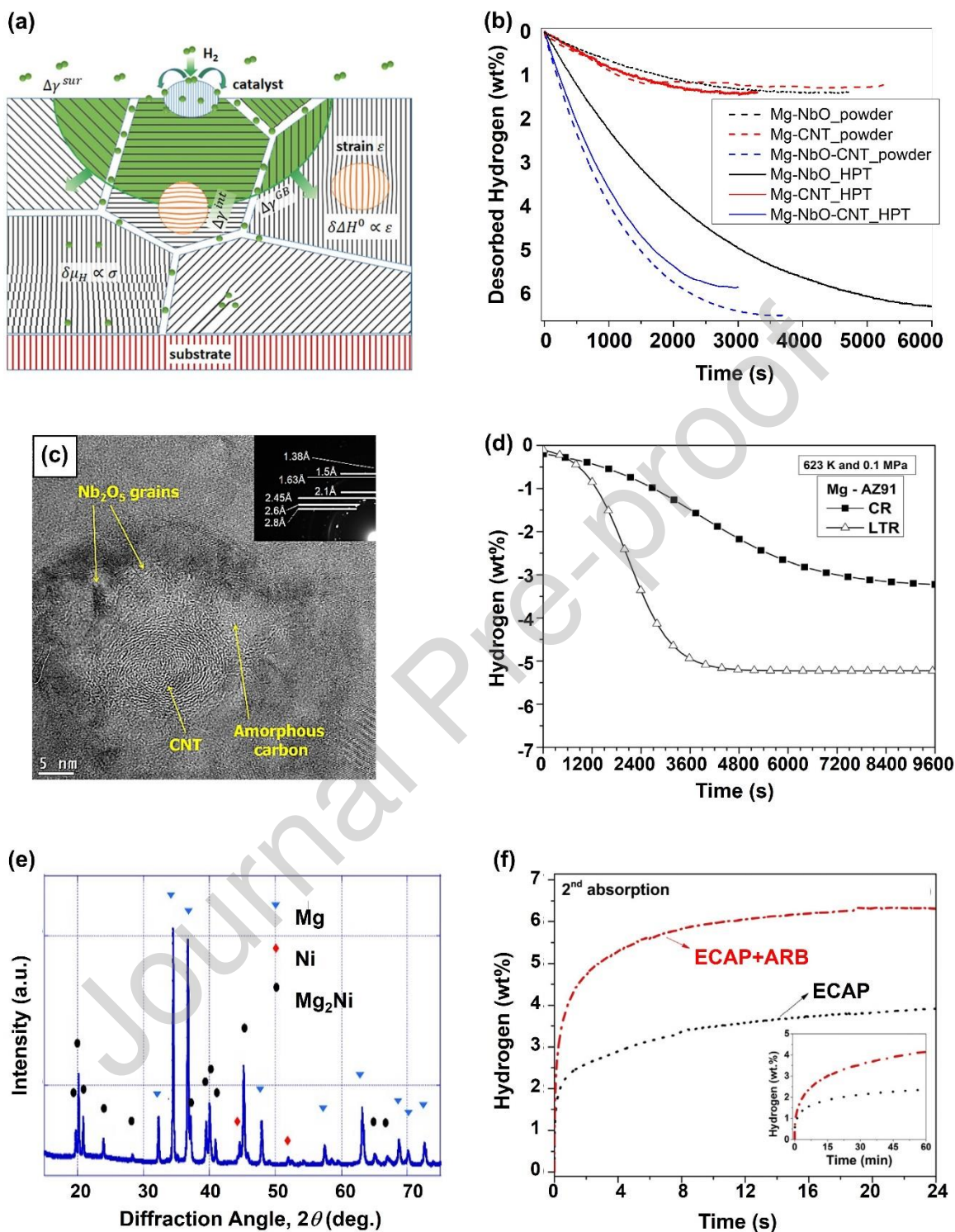
Fig. 51. (a) Structural and geometrical features relevant to hydrogen sorption in nanomaterials [1078]. The growth of the hydride phase, depicted in green, requires H_2 dissociation possibly favored by a catalyst, subsurface penetration and H diffusion, which is accelerated along internal interfaces or line defects (dislocations). (b) Dehydrogenation kinetic measurements obtained at 573 K and 1 kPa for nanocrystalline magnesium powders catalyzed by Nb 2 O 5 and/or carbon nanotube (CNT) and for the corresponding HPT-processed discs [1083]. (c) High-resolution lattice
