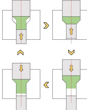
Repetitive upsetting and extrusion (RUE) [92]
