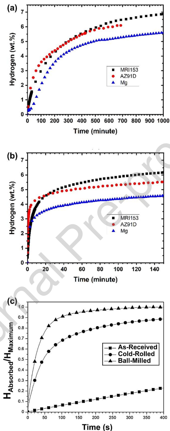
Fig. 54. (a) First and (b) second hydrogenation at 623 K under 2 MPa of hydrogen for cold-rolled pure magnesium, MRI153 and Az91D alloys [1154,1161]. (c) Normalized kinetic absorption at 623K and under 2.0 MPa hydrogen pressure for MgH 2 in as-received, cold rolled (five passes, CR5X) and mechanically milled for 30 minutes (BM 30 m) [1163].
