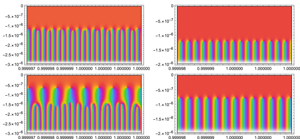
FIGURE 3. (Top) A plot showing the resonances arising in the setting of N = 5 . (Bottom) The cases of N = 6 . In both cases, by varying values of \beta and \ell , we can generate either multiple resonance lines or only one line.
