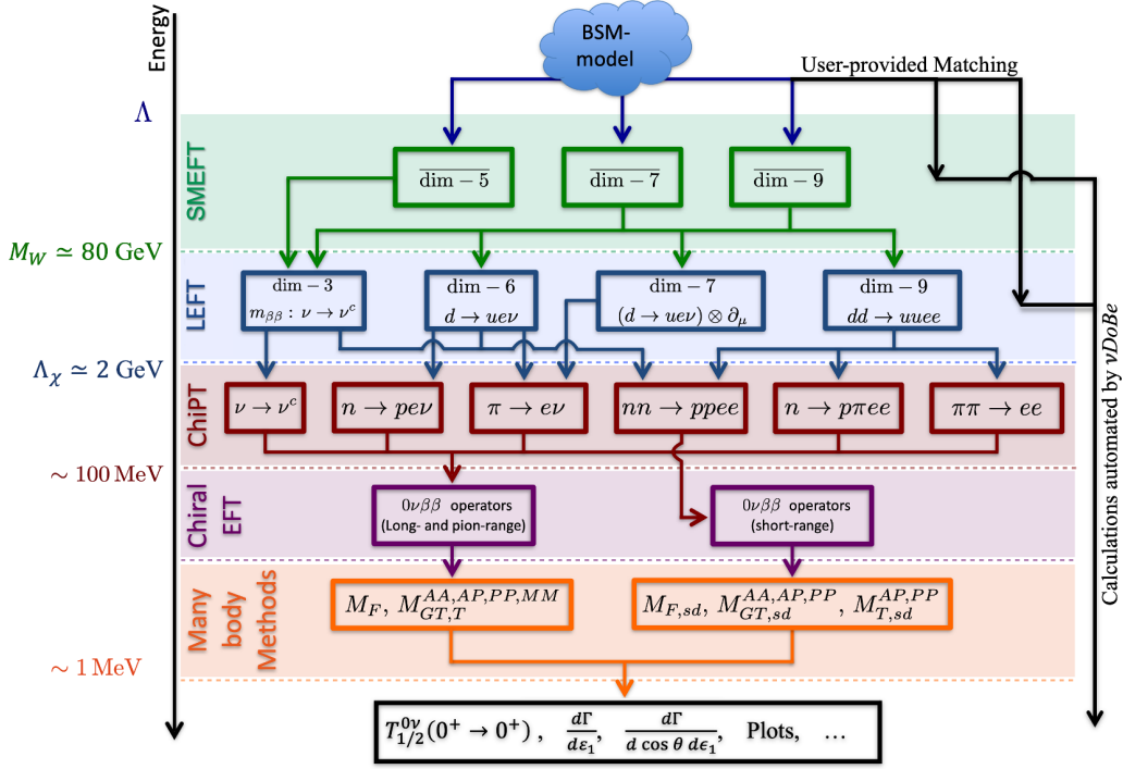
Figure 1. The EFT approach applied in \nu DoBe. Given a certain lepton number violating BSM-model, all 0\nu\beta\beta observables of interest can be calculated by following a subsequent chain of EFTs. In \nu DoBe the user is required to provide the matching conditions at either SMEFT or LEFT level. The calculations of 0\nu\beta\beta observables, plots, etc. are then automated by \nu DoBe. Figure modified from ref. [32].
