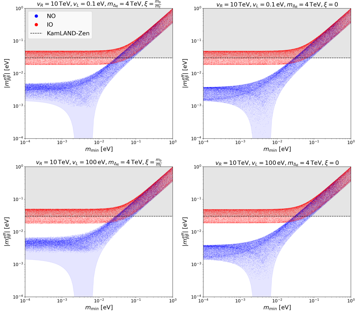
Figure 5. The effective Majorana mass m_{\beta\beta}^{\text{eff}} in dependence on the minimal light neutrino mass for the four parameter settings listed in (3.13). The shaded areas show the Majorana mass m_{\beta\beta} arising from the light-neutrino-exchange mechanism alone, while the scattered points show the resulting effective mass for the different mLRSM realizations when varying the unknown Majorana phases, \theta_L and \alpha . Both the normal (blue) and the inverted (red) mass orderings are displayed. The gray area shows the current limit given by KamLAND-Zen.
