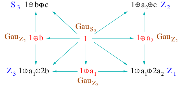
FIG. 17. 1+1D S_3 symmetry is described by symmetry TO \text{Gau}_{S_3} ( S_3 gauge theory with charge excitations). The \text{Gau}_{S_3} topological order has eight condensable algebras, and four of them are Lagrangian (the black ones above). They give rise to gapped phases as the corresponding gapped boundary states. We also indicate the unbroken symmetry groups of these phases. Four of eight are not Lagrangian, and give rise to gapless states. We also indicate the condensation-induced topological orders whose canonical boundaries give rise to these gapless states. The gapless states are critical points for the transitions between gapped or gapless states, as indicated above. The arrows indicate the embedding maps of condensable algebra and the directions of more condensation. All critical points has only one symmetric local relevant operator and are stable critical points.
