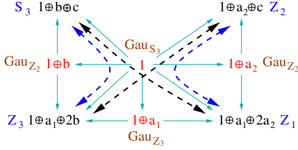
FIG. 18. The gapless \mathbf{1} -state described by eqn. (46) has one relevant direction. If this relevant direction corresponds to the competing pair (a_1, c) , the gapless \mathbf{1} -state may be the critical point of the potential continuous transitions represented by the four curved double-arrows. These potential continuous transitions are the ones that we cannot rule out at the moment.
