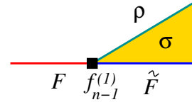
FIG. 25. When \mathcal{D}_n \equiv F is anomaly-free, Fig. 24 becomes the above, which is another way to represent Fig. 22.
