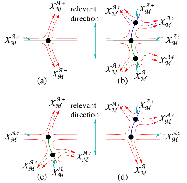
FIG. 27. The curves with arrow represent the RG flow. The dots represent the fixed points of the RG flow. The plane is a subspace of the total moduli space \mathcal{X}_M (the space formed by \mathcal{M} -systems). Let \mathcal{X}_M^A be the subspace formed by \mathcal{A} -states. The horizontal line is a subspace of \mathcal{X}_M^{\mathcal{A}_c} . In (a), the subspaces \mathcal{X}_M^{\mathcal{A}_+} and \mathcal{X}_M^{\mathcal{A}_-} are upper and lower half planes. In (b), the sub-spaces \mathcal{X}_M^{\mathcal{A}_+} and \mathcal{X}_M^{\mathcal{A}_-} are two marked curves. (c) and (d) are combinations of (a) and (b).
