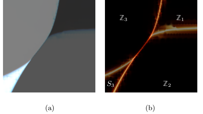
FIG. 14. A phase diagram for the first model (33) with 1.2 < J_1\beta < 1.4 (horizontal axis), 0.6 < J_2\beta < 1.0 (vertical axis), and J_c\beta = 1.5 . (a) A plot of 1/GSD , where GSD \equiv Z^2(L, L)/Z(L, 2L) and Z(L_1, L_2) is the partition function for system of size L_1 \times L_2 . (b) A plot of central charge c . Z(L, L_\infty) has a form e^{-L_\infty[\epsilon L - \frac{2\pi c}{24L} + o(L^{-1})]} when L_\infty \gg L , where c is the central charge. The red-channel of the colored image is for system of size 64 \times 64 , green-channel for 128 \times 128 , and blue-channel for 256 \times 256 .
