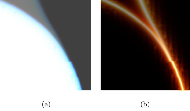
FIG. 11. A phase diagram for the model (25) with 0.993 < J_1\beta < 1.083 (horizontal axis), 0.533 < J_2\beta < 0.773 (vertical axis), and J\beta = J_c\beta = 1.0 . (a) A plot of 1/GSD , where GSD is obtained from the partition function: GSD \equiv Z^2(L, L)/Z(L, 2L) where Z(L_1, L_2) is the partition function for system of size L_1 \times L_2 . For gapped quantum systems, GSD happen to be the ground state degeneracy. (b) A plot of central charge c . The central charge c is also obtained from the partition function Z(L, L_\infty) , which has a form e^{-L_\infty[\epsilon L - \frac{2\pi c}{24L} + o(L^{-1})]} when L_\infty \gg L , where c is the central charge. This way, the central charge c is defined even for non-critical states. The red-channel of the colored image is for system of size 64 \times 64 , green-channel for 128 \times 128 , and blue-channel for 256 \times 256 .
