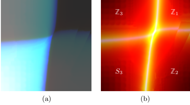
FIG. 16. A phase diagram for the first model (33) with 1.02125 < J_1\beta < 1.04125 (horizontal axis), 0.851875 < J_2\beta < 0.891875 (vertical axis), and J_c\beta = 0.5 . (a) A plot of 1/GSD . (b) A plot of central charge c . The red-channel of the colored image is for system of size 64 \times 64 , green-channel for 256 \times 256 , and blue-channel for 1024 \times 1024 .
