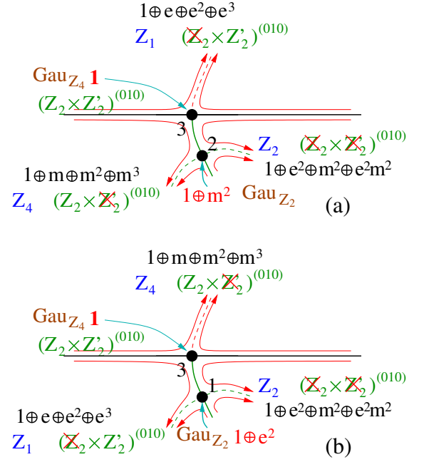
FIG. 10. Other possible local phase diagrams near the gapless 1 -state, if the relevant direction corresponds to the condensation of (a) competing pair (e, m^2) or (b) competing pair (m, e^2) . This requires the relevant direction of certain (c, \bar{c}) = (1, 1) u(1) CFT's to flow to the (c, \bar{c}) = (\frac{1}{2}, \frac{1}{2}) Ising CFT.
