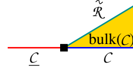
FIG. 23. In Ref. ? , Fig. 22 was drawn as the above, where F = \underline{C} , \tilde{F} = C , \rho = \tilde{\mathcal{R}} , and \sigma = \text{bulk}(C) . (See Fig. 24 and Fig. 29 in Ref. ? ).
