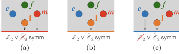
FIG. 2. A 1+1D \mathbb{Z}_2 -symmetric system (which also has a dual \tilde{\mathbb{Z}}_2 symmetry [? ]) is a \mathcal{Gau}_{\mathbb{Z}_2} -system, i.e. the system has a categorical symmetry ® \mathbb{Z}_2 \vee \tilde{\mathbb{Z}}_2 , which is described by symmetry TO \mathcal{Gau}_{\mathbb{Z}_2} – the quantum double of \mathbb{Z}_2 group. Physically, the above statement means that the \mathbb{Z}_2 symmetric system (when restricted to its symmetric sub-Hilbert space) can be exactly low-energy simulated by a boundary of bulk \mathbb{Z}_2 topological order (TO), described by \mathbb{Z}_2 gauge theory. The symmetry TO \mathcal{Gau}_{\mathbb{Z}_2} has four anyons 1, e, m, f = e \otimes m . The possible condensation-induced states in \mathcal{Gau}_{\mathbb{Z}_2} -system are given by the condensable algebras of the symmetry TO, \mathcal{A} = 1, 1 \oplus e, 1 \oplus m . (a) The 1 \oplus m -state, corresponding to the 1 \oplus m -condensed boundary, is the \mathbb{Z}_2 -symmetric state. (c) The 1 \oplus e -state is the state with spontaneous \mathbb{Z}_2 symmetry breaking. (b) The 1 -state is the gapless critical point at the continuous transition between 1 \oplus m -state and 1 \oplus e -state.
