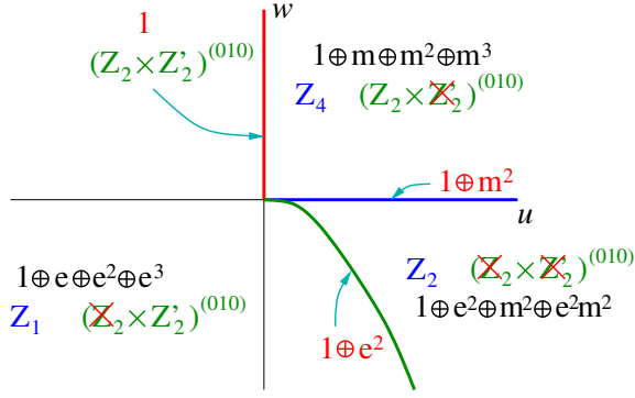
FIG. 6. Mean-field phase diagram for systems with \mathbb{Z}_4 symmetry. It has three gapped phases with unbroken \mathbb{Z}_4 , \mathbb{Z}_2 , and \mathbb{Z}_1 symmetries. The two phase transitions \mathbb{Z}_4 \rightarrow \mathbb{Z}_2 (marked by 1 \oplus m^2 ) and \mathbb{Z}_2 \rightarrow \mathbb{Z}_1 (marked by 1 \oplus e^2 ) are critical points described by the same Ising CFT. The direct phase transition \mathbb{Z}_4 \rightarrow \mathbb{Z}_1 (marked by 1 ) corresponds to a critical point that does not break the anomalous symmetry (\mathbb{Z}_2 \times \mathbb{Z}_2')^{(010)} and has the full symmetry TO \text{Gau}_{\mathbb{Z}_4} . It is a critical line that includes the \mathbb{Z}_4 parafermion CFT.
