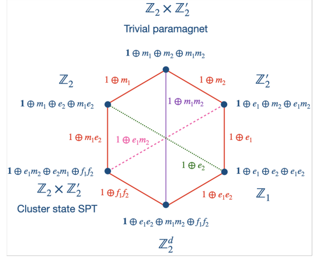
FIG. 4. A \mathbb{Z}_2 \times \mathbb{Z}'_2 symmetric system has a symmetry described by 2+1D \mathbb{Z}_2 \times \mathbb{Z}'_2 topological order \mathcal{G}_{\text{au}_{\mathbb{Z}_2 \times \mathbb{Z}'_2}} . Here, the 6 Lagrangian condensable algebras of \mathcal{G}_{\text{au}_{\mathbb{Z}_2 \times \mathbb{Z}'_2}} are represented by the vertices of the hexagon. The gapped phases they correspond to are described in terms of their symmetry-breaking/SPT order. A connecting edge between any pair represents a non-Lagrangian condensable algebra which is strictly included in both of them, and therefore corresponds to a phase transition between them. There is also a trivial condensable algebra \mathbf{1} , which is not shown in this picture; it corresponds to a multicritical point between any two gapped phases. The inclusion relations between condensable algebras have implication on the structure of phase diagram. For example, the edge labeled by \mathbf{1} \oplus m_2 connecting vertices labeled by \mathbf{1} \oplus m_1 \oplus m_2 \oplus m_1 m_2 and \mathbf{1} \oplus e_1 \oplus m_2 \oplus e_1 m_2 suggests that the former (gapless) \mathbf{1} \oplus m_2 -state describes a critical point for the stable continuous transition between the latter two gapped states. For this transition to be non-fine-tuned, the gapless \mathbf{1} \oplus m_2 -state must have only one symmetric relevant operator, which is indeed the case here (see main text for details).
