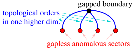
FIG. 21. Symm/TO correspondence where (emergent) symmetry is viewed as anomaly (Fig. 1 in Ref. ? ).
