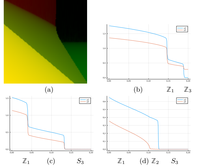
FIG. 13. Mean-field phase diagram of (31) in (u, v) space, for \alpha = \beta = 1, \gamma = -0.5 . (a): the horizontal axis is u \in [0, 0.2] and the vertical axis is v \in [-0.2, 0.2] . The red channel corresponds to the value of the S_3 order parameter \sqrt{|\Phi_1|^2 + |\Phi_2|^2} . The green channel corresponds to the value of the \mathbb{Z}_2 order parameter \sqrt{|\phi|} . The black region corresponds to a S_3 symmetric phase, the red region to a \mathbb{Z}_2 symmetric phase, the green region to a \mathbb{Z}_3 symmetric phase, and the yellow region to a \mathbb{Z}_1 phase. (b),(c),(d): Plots of \sqrt{|\Phi_1|^2 + |\Phi_2|^2} ( y_1 ) and |\phi| ( y_2 ), for u \in [0, 0.2] , and (b) v = -0.16 , (c) v = 0.02 , (d) v = 0.1 .
