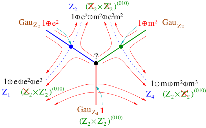
FIG. 9. A possible global phase diagram for systems with \mathbb{Z}_4 symmetry or (\mathbb{Z}_2 \times \mathbb{Z}_2')^{(010)} symmetry, which has a similar topology with the mean-field phase diagram Fig. 6. We are not sure about the phase structure near the center of the phase diagram.
