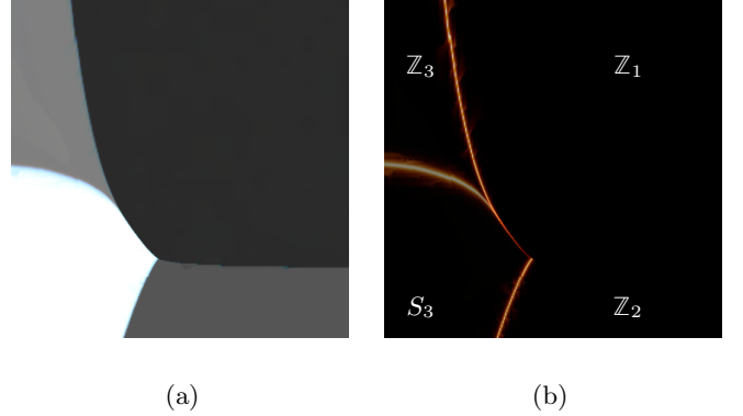
FIG. 15. A phase diagram for the second model (34) with 0.57 < J_1\beta < 1.29 (horizontal axis), 0.4775 < J_2\beta < 1.2275 (vertical axis), and J\beta = 1 - J_2\beta , J_c\beta = 1 . (a) A plot of 1/GSD . (b) A plot of central charge c . The red-channel of the colored image is for system of size 64 \times 64 , green-channel for 128 \times 128 , and blue-channel for 256 \times 256 .
