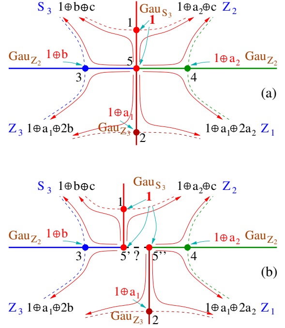
FIG. 20. Two possible global phase diagrams for systems with S_3 symmetry, which contains four gapped phases with unbroken symmetries, S_3 , \mathbb{Z}_3 , \mathbb{Z}_2 , and \mathbb{Z}_1 . The curves with arrow represent the RG flow, and the dots are the RG fixed points that correspond to the critical points of phase transitions. The right horizontal line is the space of Hamiltonians whose ground states have a condensation \mathcal{A} = 1 \oplus a_2 (see Appendix B), which is the basin of attraction of the RG fixed point 4. The left horizontal line is the space of Hamiltonians whose ground states have a condensation \mathcal{A} = 1 \oplus b , the basin of attraction of the RG fixed point 3. The upper vertical line is the space of Hamiltonians whose ground states have a condensation \mathcal{A} = 1 , the basin of attraction of the RG fixed point 1. The lower vertical line is the space of Hamiltonians whose ground states have a condensation \mathcal{A} = 1 \oplus a_1 , the basin of attraction of the RG fixed point 2. The critical point 3 and 4 are the (c, \bar{c}) = (\frac{1}{2}, \frac{1}{2}) Ising CFT (the canonical boundary of \mathcal{G}\text{au}_{\mathbb{Z}_2} topological order). The critical point 1 is a (c, \bar{c}) = (\frac{4}{5}, \frac{4}{5}) CFT (46) from (6, 5) minimal model (the canonical boundary of \mathcal{G}\text{au}_{S_3} topological order). The critical point 2 is another (c, \bar{c}) = (\frac{4}{5}, \frac{4}{5}) CFT (42) also from (6, 5) minimal model (the canonical boundary of \mathcal{G}\text{au}_{\mathbb{Z}_3} topological order). The tricritical points 5, 5', and 5'' are described by gapless 1 -condensed states with two S_3 symmetric relevant operators. The (c, \bar{c}) = (\frac{5}{6}, \frac{5}{6}) CFT (47) from (7, 6) minimal model is one such gapless 1 -condensed state. We also list the corresponding condensable algebras for these gapped phases and gapless critical points.
