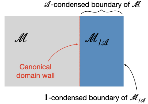
FIG. 3. A \mathcal{A} -state in a \mathcal{M} -system corresponds to a \mathcal{A} -condensed boundary of symmetry TO \mathcal{M} . Such a boundary can be obtained by attaching \mathcal{A} -condensation induced topological order \mathcal{M}_{/\mathcal{A}} with 1-condensed boundary. The \mathcal{A} -condensation changes \mathcal{M} to \mathcal{M}_{/\mathcal{A}} , causing a symmetry TO breaking , in that the symmetry TO of the state is smaller than that of the system. \mathcal{M}_{/\mathcal{A}} is the unbroken symmetry TO (an analogue of unbroken symmetry) of the \mathcal{A} -state.
