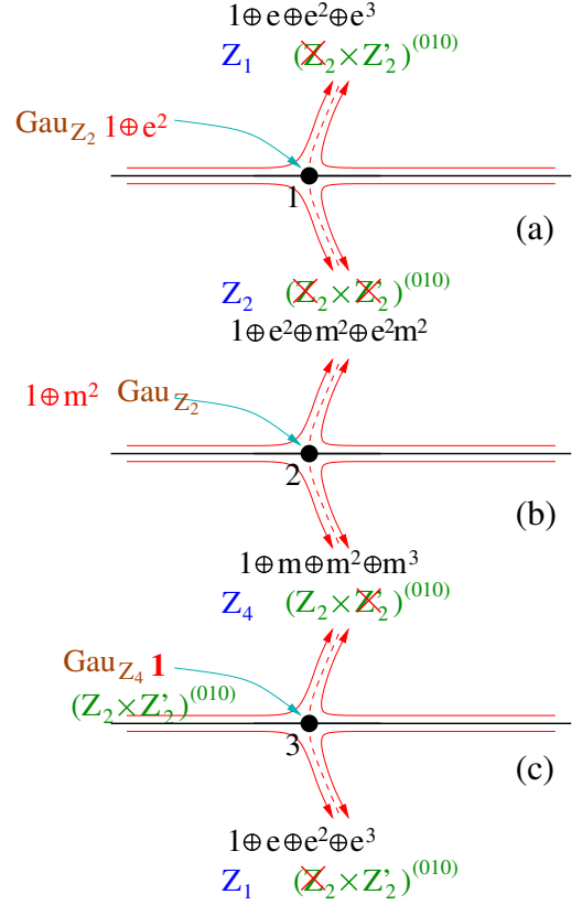
FIG. 8. Possible local phase diagram for systems with \mathbb{Z}_4 symmetry, which contains three gapped phases with unbroken symmetries, \mathbb{Z}_4 , \mathbb{Z}_2 , and \mathbb{Z}_1 . The curves with arrows represent the RG flow, and the dots are the RG fixed points that correspond to the critical points of phase transitions. The plane is a space of Hamiltonians with symmetry TO \mathcal{G}_{\text{auZ}_4} (see Appendix B for detailed discussions). The horizontal line in (a) is a space of Hamiltonians whose ground states have the condensation \mathcal{A} = \mathbf{1} \oplus e^2 , which is the basin of attraction of the RG fixed point 1. The horizontal line in (b) is a space of Hamiltonians whose ground states have the condensation \mathcal{A} = \mathbf{1} \oplus m^2 , the basin of attraction of the RG fixed point 2. The horizontal line in (c) is a space of Hamiltonians whose ground states have the condensation \mathcal{A} = \mathbf{1} , the basin of attraction of the RG fixed point 3. The critical point 3 is actually part of a critical line of (c, \bar{c}) = (1, 1) u(1) CFT (the canonical boundary of \mathcal{G}_{\text{auZ}_4} topological order). The critical point 1 and 2 are the (c, \bar{c}) = (\frac{1}{2}, \frac{1}{2}) Ising CFT (the canonical boundary of \mathcal{G}_{\text{auZ}_2} topological order). We also list the corresponding condensable algebras, for each gapped phase and gapless critical point.
