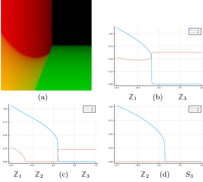
FIG. 12. Mean-field phase diagram of (31) in (u, v) space, for \alpha = \beta = \gamma = 1 . (a): the horizontal axis is u \in [-1, 1] and the vertical axis is v \in [-1, 1] . The red channel corresponds to the value of the S_3 order parameter \sqrt{|\Phi_1|^2 + |\Phi_2|^2} . The green channel corresponds to the value of the \mathbb{Z}_2 order parameter \sqrt{|\phi|} . The black region corresponds to a S_3 symmetric phase, the red region to a \mathbb{Z}_2 symmetric phase, the green region to a \mathbb{Z}_3 symmetric phase, and the yellow region to a \mathbb{Z}_1 phase. (b),(c),(d): Plots of \sqrt{|\Phi_1|^2 + |\Phi_2|^2} ( y_1 ) and |\phi| ( y_2 ), for u \in [-1, 1] , and (b) v = -0.8 , (c) v = -0.1 , (d) v = 0.5 .
