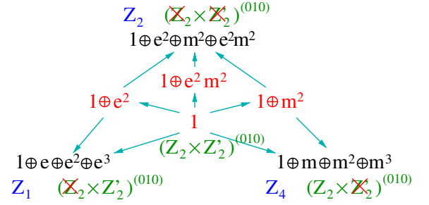
FIG. 7. \mathbb{Z}_4 -symmetric systems has a symmetry described by 2+1D \mathbb{Z}_4 topological order \text{Gau}_{\mathbb{Z}_4} (i.e. a \mathbb{Z}_4 gauge theory). The \text{Gau}_{\mathbb{Z}_4} topological order has seven condensable algebras, and 3 of them are Lagrangian (the back ones above). They give rise to gapped boundaries. Four of seven are not Lagrangian, and give rise to gapless boundaries. The gapless boundaries may be critical points for the transitions between gapped or gapless boundaries, as indicated above. The arrows indicate the directions of more condensation.
