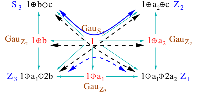
FIG. 19. The gapless \mathbf{1} -state described by eqn. (46) has one relevant direction. If this relevant direction corresponds to the competing pair (a_2, b) , the gapless \mathbf{1} -state may be the critical point of the potential continuous transitions represented by the eight curved double-arrows. The dashed curves are the potential continuous transitions that we cannot rule out at the moment. The solid curve is the continuous transition that is known to be realized by 3-state Potts model.
