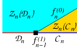
FIG. 24. A morphism between n + 1 D (gapped or gapless) quantum field theories \mathcal{C}_n and \mathcal{D}_n with (non-invertible) gravitational anomalies. See (4.3) of Ref. [?].
