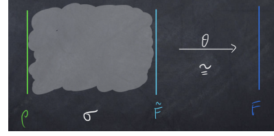
FIG. 22. A pair (\rho, \sigma) describes a “topological symmetry” in an anomaly-free field theory F (Fig. 1 in Ref. ? ).
