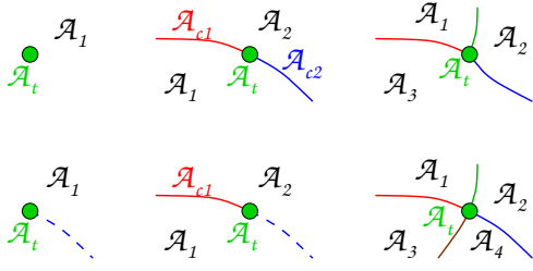
FIG. 26. Some possible structures of the phases near a tricritical point \mathcal{A}_t (the dot). The solid curves are continuous transitions (described by \mathcal{A}_{c1} , \mathcal{A}_{c2} , etc.). The dashed curves are first-order transitions.
