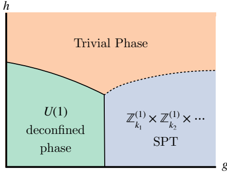
FIG. 2. The schematic phase diagram of the model described by Eq. (34) with the additional term contributing to the action amplitude e^{h \sum_{ij,I} a_{I,ij}^{\mathbb{R}/\mathbb{Z}}} . When h = 0 , there is no fluctuations of U(1) gauge charge, and the model has an exact \mathbb{Z}_{k_1}^{(1)} \times \mathbb{Z}_{k_2}^{(1)} \times \dots 1-symmetry. For h \neq 0 , this becomes an exact emergent \mathbb{Z}_{k_1}^{(1)} \times \mathbb{Z}_{k_2}^{(1)} \times \dots 1-symmetry existing below the energy gaps of U(1) gauge charges, which exists in the green and purple shaded regions. Due to the 2\pi -quantized topological term, in the confined phase (shown in purple) there is an SPT order protected by the exact emergent \mathbb{Z}_{k_1}^{(1)} \times \mathbb{Z}_{k_2}^{(1)} \times \dots 1-symmetry whose SPT invariant is given by Eq. (70).
