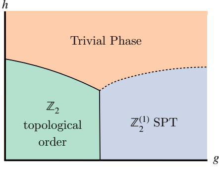
FIG. 1. The schematic phase diagram of the model described by Eq. (13). There is a topologically ordered phase described by the deconfined phase of \mathbb{Z}_2 gauge theory (shown in green), and a gapped short-range entangled phase (corresponding to the regions shaded in orange and purple). At energies below the \mathbb{Z}_2 gauge charge gap, the confined phase (colored in purple) has an exact emergent \mathbb{Z}_2^{(1)} symmetry, while the symmetry is absent at all energy scales in the trivial phase (colored in orange). At h = 0 , this \mathbb{Z}_2^{(1)} symmetry in the confined phase is exact. Due to the 2\pi -quantized topological term, the confined phase has a nontrivial SPT order protected by this exact emergent \mathbb{Z}_2^{(1)} symmetry. The SPT invariant describing this 1-SPT order is given by Eq. (11)
