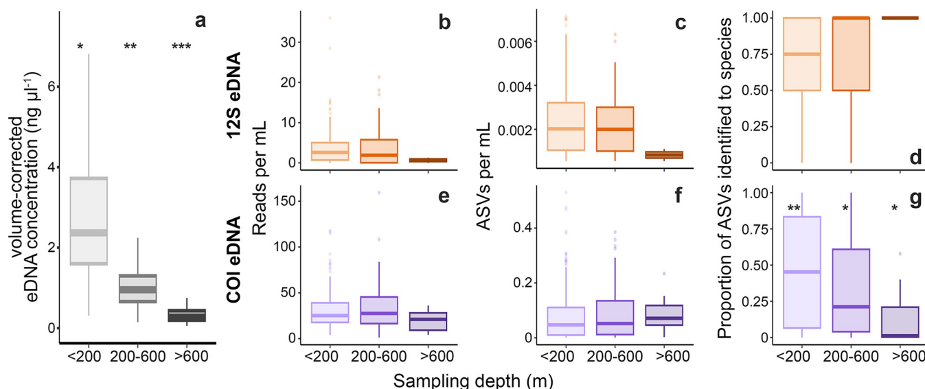
Fig 5. eDNA sample characteristics with respect to primer and sampling depth. (a) The concentration of DNA per sample decreased with depth (n = 433). For samples with more than 1,000 reads, the number of reads per mL (b,e) and total ASVs per mL of seawater (c,f) were not meaningfully variable across depth bins. The proportion of ASVs assigned to species (d,g) decreased with depth for COI samples (n = 331), with 12S samples (n = 231) having higher proportions of species-level identifications than COI across depths. Statistical differences among depth bins (Games-Howell, p < 0.05 ) are indicated by the number of asterisks. Results of global and post hoc tests describing the effects of depth bin on each eDNA metric are given in Table 3.
