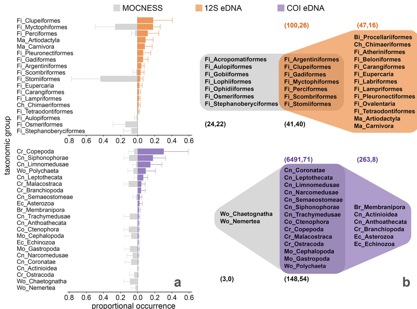
Fig 3. eDNA sampled a higher diversity of taxonomic groups than MOCNESS. (a) Mean proportional occurrence ( \pm SD) of taxonomic groups in co-located MOCNESS ( n = 27 nets) and eDNA samples from 0–1,750 m for vertebrate ( n = 211 12S samples) and invertebrate groups ( n = 244 COI samples). Bar charts include taxonomic orders with mean proportional occurrences greater than 0.01. (b) Venn diagrams show a higher richness of taxonomic groups sampled by eDNA than MOCNESS for both primers, but a higher number of vertebrate species were detected by MOCNESS. Number pairs describe total and species-level taxonomic richness for each method (number of ASVs for eDNA and unique taxonomic assignments for MOCNESS, number of species). Taxonomic group type key: Fi = bony fish, Ch = cartilaginous fish, Ma = mammal, Bi = bird; Cn = cnidarian, Cr = crustacean, Mo = mollusc, Br = bryozoan, Wo = worm, Ec = echinoderm.
