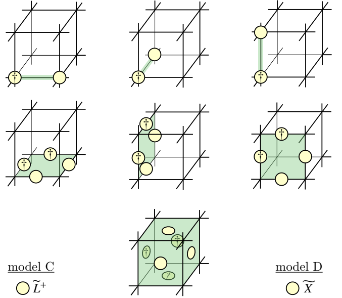
FIG. 8. Graphical representation of \tilde{W}^\dagger(\partial c_{p+1}) for model C (Eq. (44)) and D (Eq. (28)) in 3d space for (1st row) p = 0 , (2nd row) p = 1 , and (3rd row) p = 2 . For model C (D), the yellow colored disks represent \tilde{L}^+ ( \tilde{X} ) operators, the product of which yields \tilde{W}^\dagger(\partial c_{p+1}) . Discs labeled by \dagger denote the hermitian conjugate and c_{p+1} is colored green.
