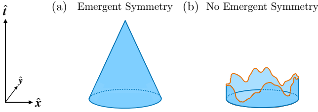
FIG. 14. Shows a cartoon of the different decay processes of 1-form symmetry excitations in 2 + 1d spacetime. The world sheet of the 1-brane excitation is colored blue, while the world-line of gauge charge excitations is orange.
