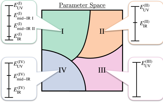
FIG. 1. The parameter space of a many-body Hamiltonian can be partitioned by its differing hierarchies of energy scales. A schematic depiction of this is shown here. The parameter space is partitioned into four regions, labeled I, II, III, and IV, with their differing energy scale hierarchies shown.
