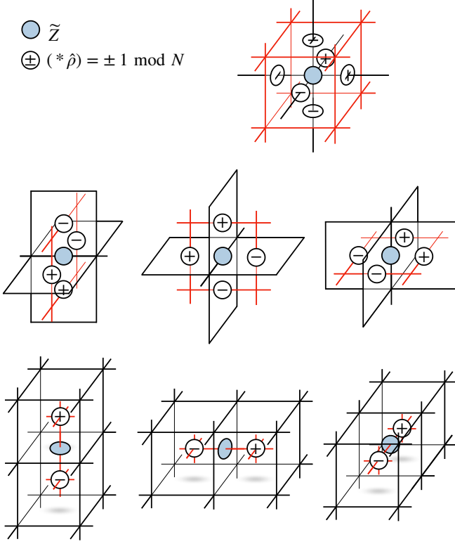
FIG. 10. Graphical representation of the topological defects created by (*\tilde{Z})_{\hat{c}_{d-p}} in model D for 3d space and (1st row) p = 0 , (2nd row) p = 1 , and (3rd row) p = 2 . The blue disk represents the (*\tilde{Z})_{\hat{c}_{d-p}} operator. The disks labeled by \pm represent (*\hat{\rho})_{c_{p+1}} = \pm 1 for that c_{p+1} (see Eq. (35)).
