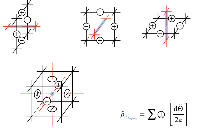
FIG. 11. Graphical representation of \hat{\rho}_{\hat{C}_{d-p-2}} (see Eq. (54)) in 3d space for (1st row) p = 0 and (2nd row) p = 1 . The \pm disks denote the sign in front of that \lfloor d\tilde{\Theta}/(2\pi) \rfloor in the sum for \hat{\rho}_{\hat{C}_{d-p-2}} . The direct lattice is colored in black, the dual lattice is in red, and \hat{\rho}_{\hat{C}_{d-p-2}} is in blue.
