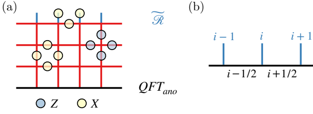
FIG. 4. (a) A lattice realization of Fig. 3b, where qubits live on the links. The star and plaquette terms of the toric code model are shown both in the bulk and on the \tilde{\mathcal{R}} boundary. (b) Since the bulk is topological, one can take the thin slab limit.
