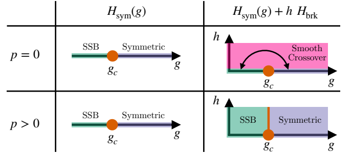
FIG. 13. A Hamiltonian H_{\text{sym}}(g) with a p -form symmetry spontaneously broken at g < g_c has a qualitatively similar phase diagram whether p = 0 or p > 0 . However, explicitly breaking the symmetry with hH_{\text{brk}} ( |h| \ll 1 ), the phase diagram of H_{\text{sym}}(g) + hH_{\text{brk}} differs between p = 0 and p > 0 . For p = 0 , there is now a smooth crossover between what used to be the SSB phase and the symmetric phase. Shown here is the case where the symmetry-breaking perturbation is relevant. For p > 0 , H_{\text{sym}}(g) + hH_{\text{brk}} has an exact emergent p -form symmetry, so there is not a smooth crossover between the phases. Starting in the SSB phase and increasing h would lead to an eventual phase transition out of the SSB phase.
