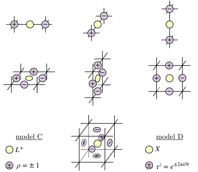
FIG. 7. Graphical representation of the excitation created by L_{c_p}^+ [X_{c_p}] in model C [D] in 3d space for (1st row) p = 1 , (2nd row) p = 2 , and (3rd row) p = 3 . The yellow disk represents L_{c_p}^+ [X_{c_p}] . For model C, the purple \pm disk denotes the sign in \rho_{c_{p-1}}(L_{c_p}^+ \langle 0 \rangle) = \pm(L_{c_p}^+ \langle 0 \rangle) for that (p-1) -cell. For model D, the \pm disk instead denotes the sign in \tau_{c_{p-1}}^z(X_{c_p} \langle 0 \rangle) = \omega^{\pm 1}(X_{c_p} \langle 0 \rangle) for that (p-1) -cell.
