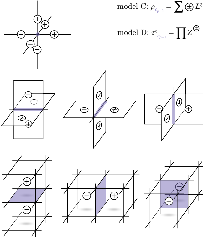
FIG. 6. Graphical representation of \rho_{c_{p-1}} in model C (42) and \tau_{c_{p-1}}^z in model D (26) in 3d space for (1st row) p = 1 , (2nd row) p = 2 , and (3rd row) p = 3 . The (p-1) -cell c_{p-1} is colored purple. The \pm disks on the p -cells denote the sign in front of L_{c_p}^z in the sum for \rho_{c_{p-1}} , or whether Z_{c_p} is Z^+ \equiv Z or Z^- \equiv Z^\dagger in the product for \tau_{c_{p-1}}^z .
