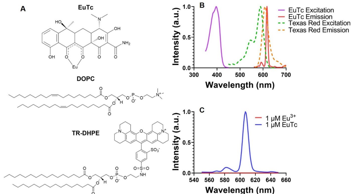
Figure 1. Molecular structures and spectroscopic characteristics of EuTc (1 \mu M) and Texas Red-DHPE with DOPC liposomes. (A) Molecular structures of EuTc, DOPC, and TR-DHPE. (B) Excitation and emission of spectra of EuTc compared with excitation and emission spectra of Texas-Red DHPE. (C) Emission spectra of the EuTc complex (1 \mu M) and \text{Eu}^{3+} (1 \mu M) alone in the presence of DOPC liposomes. EuTc and \text{Eu}^{3+} were excited at 400 nm.
