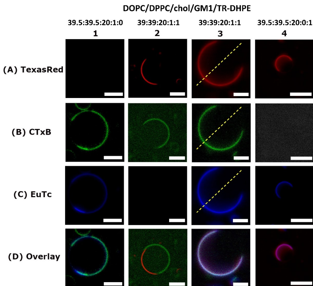
Figure 6. Imaging phase separation in GUVs. Phase separating GUVs imaged by either Texas Red (TR-DHPE) and/or EuTc luminescence and/or CTxB-AlexaFluor647. The GUVs were composed of DOPC, DPPC, cholesterol, GM1, and TR-DHPE. The ratios above the column labels are the molar ratios of the lipids in the GUVs. Rows indicate fluorescence due to (A) Texas Red-DHPE, (B) CTxB-AlexaFluor647, and (C) EuTc labeling. Overlay images (D) colocalization of the various probes. Images shown depict the GUVs in their final state, i.e. with all labels present for a given condition. Fluorescence intensity profiles along the dashed lines are shown in Fig. S6. All scale bars are 5 \mu m.
