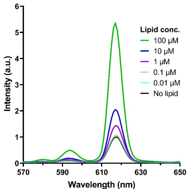
Figure 2. EuTc emission intensity in the presence of varying concentration of DOPC liposomes. The DOPC liposomes enhance EuTc emission intensity in a concentration-dependent manner.
