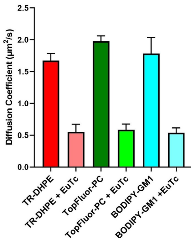
Figure 9. Influence of EuTc on lipid diffusion coefficients in SLBs. Diffusion coefficients of TR-DHPE, TopFluorPC, and BODIPY-GM1 in DOPC SLBs before and after addition of EuTc (+ EuTc). Data is represented as mean \pm standard deviation, N \geq 9 for all samples.
