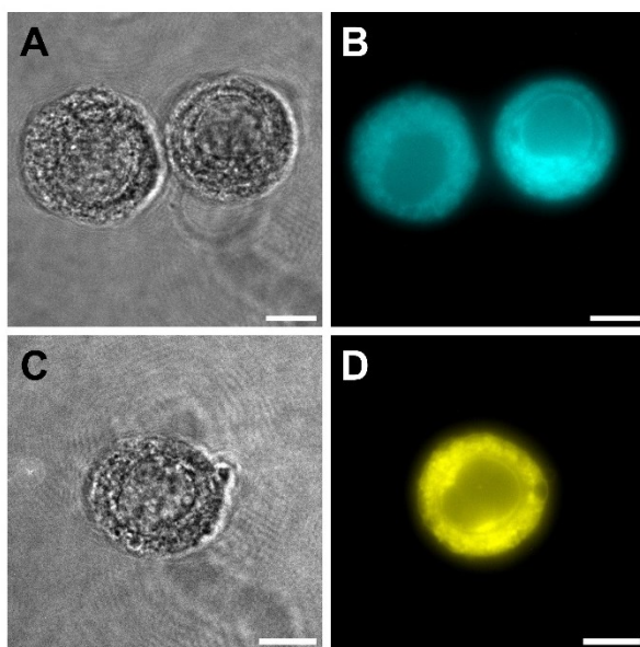
Figure 10. Cellular membrane labeling with EuTc. (A-B) UMSCC-2 cells incubated with EuTc and then imaged in brightfield (A) and EuTc (B) channels. (C-D) A UMSCC-2 cell incubated with FM1-43 then imaged in brightfield (C) and FM1-43 (D) channels. All scale bars are 10 \mu M.
