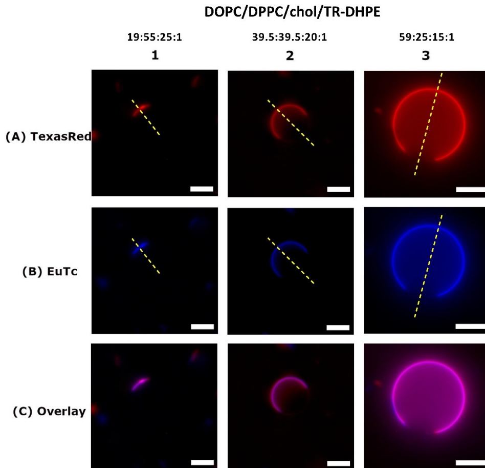
Figure 5. Phase separating GUVs composed of DOPC, DPPC, cholesterol, and TR-DHPE with varying area fraction of the Ld and Lo phases imaged by Texas Red (TR-DHPE) and EuTc luminescence. The ratios above the column numbers indicate the molar ratios of DOPC, DPPC, cholesterol, and TR-DHPE in the GUV. Rows indicate fluorescence due to (A) Texas Red-DHPE and (B) EuTc labeling. Overlay images (C) show colocalization of EuTc and Texas Red on the GUV membrane. Fluorescence intensity profiles along the yellow dashed lines are shown in Fig. S5. All scale bars are 5 \mu m.
