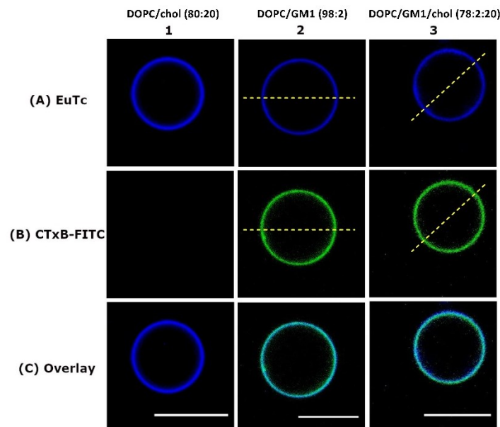
Figure 4. Single phase GUVs labeled with EuTc and CTxB-FITC. The GUV compositions are noted above the column numbers. Rows indicate fluorescence due to (A) EuTc and (B) CTxB-FITC labeling. Overlay images (C) show colocalization of EuTc and CTxB-FITC on the GUV membrane only when GM1 is present. Intensity profiles along the yellow dashed lines in Columns 2 and 3 can be shown in Fig. S2. All scale bars are 10 \mu\text{m} .
