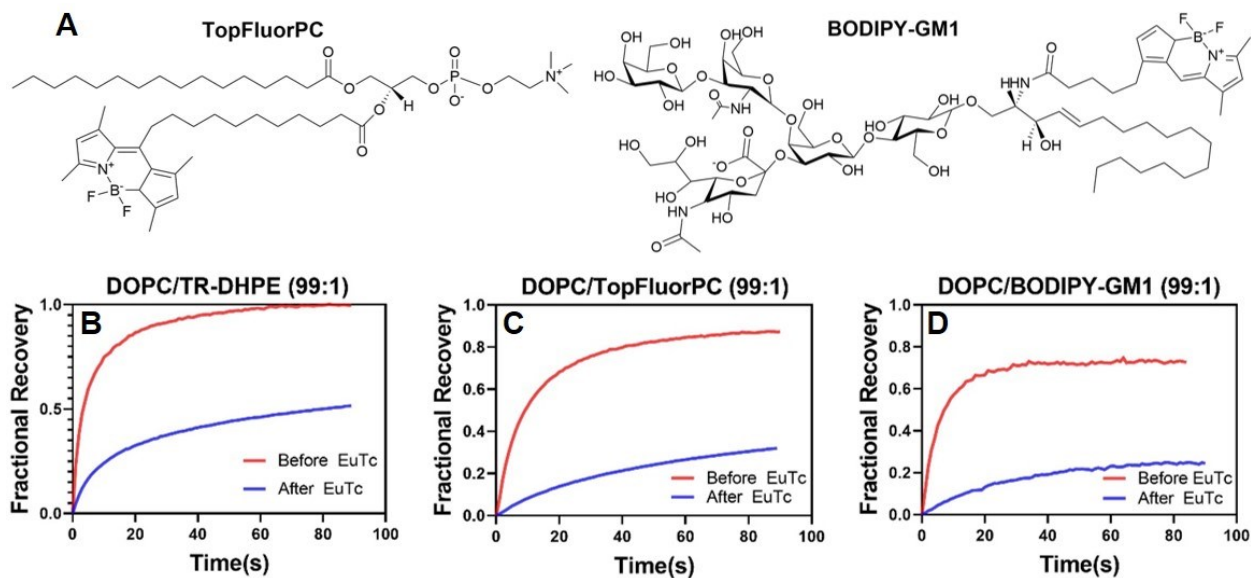
Figure 8. Molecular structures of TopFluorPC and BODIPY-GM1 (A). FRAP recovery curves of DOPC/TR-DHPE (99:1) (B), DOPC/TopFluorPC (99:1) (C), and DOPC/BODIPY-GM1 (99:1) (D) SLBs before and after EuTc exposure.
