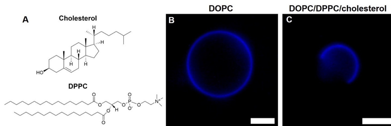
Figure 3. EuTc labeled GUVs. (A) Molecular structures of DPPC and cholesterol. (B) DOPC GUV and (C) phase separated GUV (DOPC/DPPC/cholesterol, 40:40:20) labeled with 1 \mu M EuTc. All scale bars are 5 \mu m.
