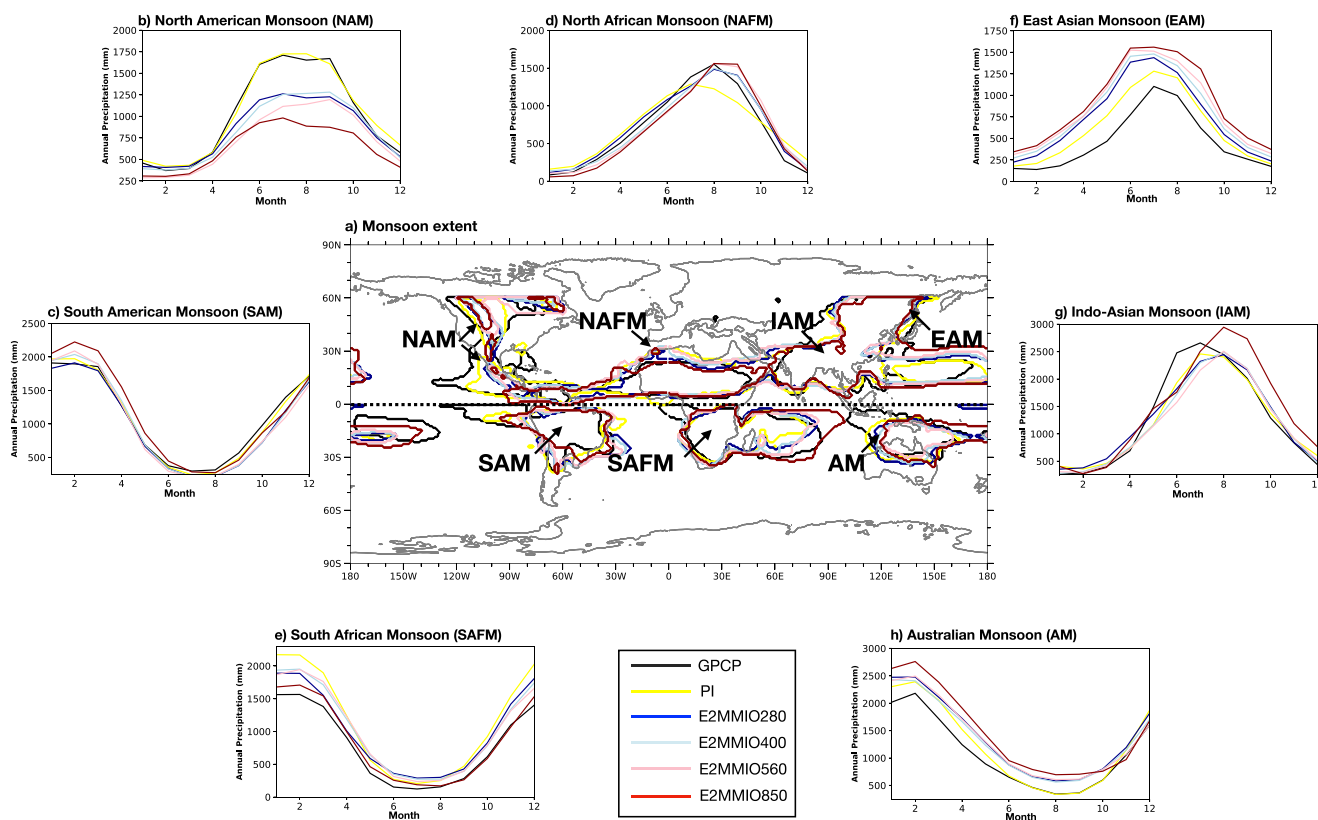
Figure 12. Early-to-middle Miocene global monsoon distribution (a). Annual precipitation cycle for regional monsoons: North American (b; NAM), South American (c; SAM), Northern African (d; NAFM), Southern African Monsoon (e; SAFM), East Asian Monsoon (f; EAM), Indo-Asian Monsoon (g; IAM), and Australian Monsoon (h; AM). Experiments show observation, Global Precipitation Climate Project (black), multi-model preindustrial ensemble (yellow), and early-to-middle Miocene multi-model ensembles 280 ppm (dark blue), 400 ppm (light blue), 560 ppm (pink), and 850 ppm (red). Monsoon extent in plot a shows regions where the percentage (>55%) of mean annual precipitation occurring during the extended boreal summer season (MJJAS, Northern Hemisphere) and during the extended austral summer season (NDJFM, Southern Hemisphere) delineated by dotted line over the equator. The regional annual precipitation cycle calculation is based on the regional monsoon extent.
