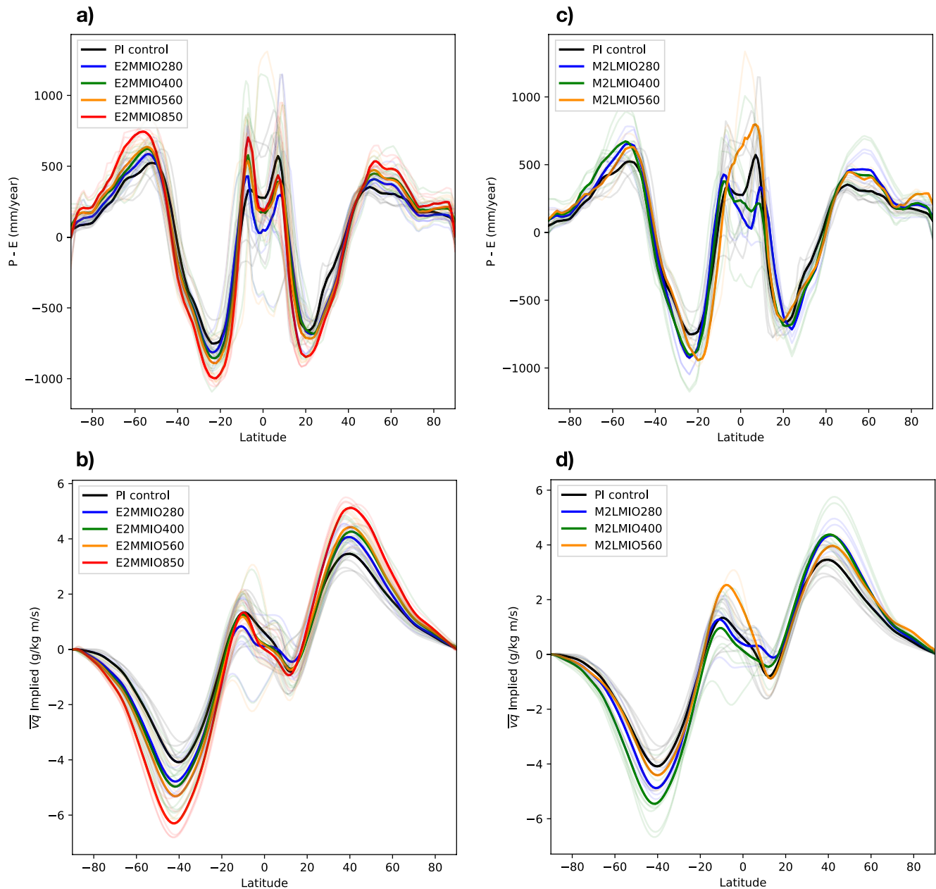
Figure 7. Zonal mean hydrological cycle analysis showing P-E (mm yr -1 ) (a and c), and implied zonal mean moisture transport (g kg -1 m s -1 ) (b and d) for early-to-middle Miocene (E2MMIO) and middle-to-late Miocene (M2LMIO) multi-model means (dark colors), and individual models (light colors).
