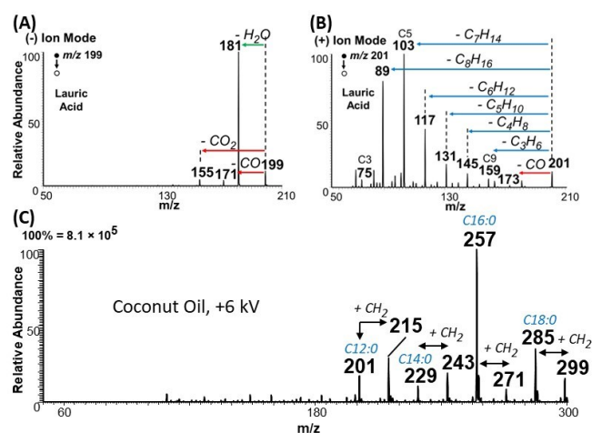
Figure 9 Comparison of tandem MS data (CID) in (A) negative- and (B) positive-ion modes for lauric acid at m/z 199 and 201, respectively. (C) Positive-ion mode mass spectrum showing the analysis of complex coconut oil diluted in MeOH using the plasma-nanodroplet fusion setup with +6 kV DC voltage applied.
