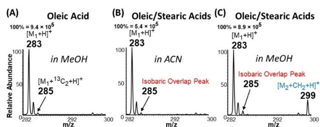
Figure 8 Demonstration of the Type II isobaric overlap phenomenon and how the effect is overcome by esterification. Positive-ion mode mass spectra obtained from the analysis of (A) 500 \mu M oleic acid ( M_1 ) in methanol, (B) 500 \mu M oleic acid with 10% stearic acid ( M_2 ; 50 \mu M) prepared in acetonitrile (no esterification), and (C) 500 \mu M oleic acid with 10% stearic acid (50 \mu M) prepared in methanol (esterification occurs). Isobaric overlap peak is a mixture of [M_1 + ^{13}C_2 + H]^+ and [M_2 + H]^+ species occurring at m/z 285. During esterification the signal due to stearic acid is shifted to m/z 299 enabling its characterization.
