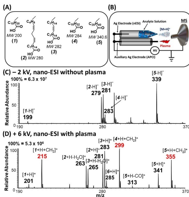
Figure 1 (A) Schematics showing the chemical structures of five fatty acids (FAs): lauric acid (1), linoleic acid (2), oleic acid (3), stearic acid (4), and behenic acid (5). (B) Experimental setup for plasma-nanodroplet fusion and online MS analysis. Nanodroplets are derived from non-contact nano-ESI where the Ag electrode is not in physical contact with analyte solution. Nonthermal plasma is derived from the auxiliary Ag electrode when DC voltage >4 kV is applied. (C) Typical negative-ion mode mass spectrum recorded following the analysis of a 200 ppm solution containing the five FAs mixture at -2 kV nano-ESI. (D) Typical positive-ion mode mass spectrum of the same FA solution recorded using the plasma-nanodroplet fusion source, using +6 kV applied voltage.
