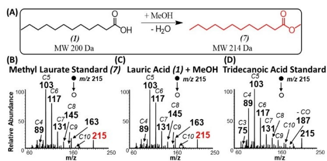
Figure 3 (A) Schematic illustrating esterification reaction between lauric acid and methanol. Positive-ion mode MS/MS analysis of (B) standard methyl laurate, (C) reaction product generated in our experiment from the analysis of lauric acid in the presence of methanol, and (D) standard of tridecanoic acid.
