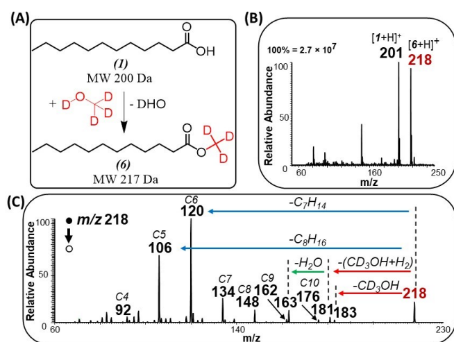
Figure 4 (A) Schematic illustrating gas-phase esterification of lauric acid ( 1 ) in presence of MeOH-D 4 vapor. (B) Positive-ion mode full MS analysis showing esterification product ( 6 ) at m/z 218. (C) MS/MS of the esterification product, m/z 218.
