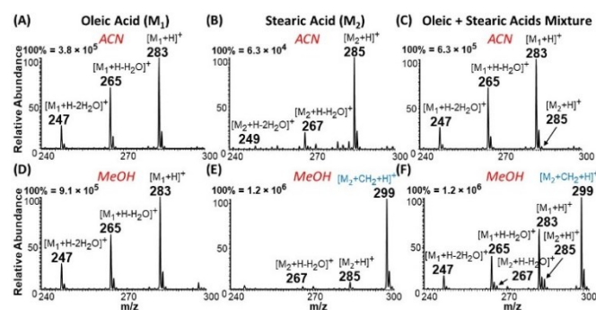
Figure 7 Positive-ion mode full MS analysis of 500 \mu M each of (A,D) oleic acid in (A) acetonitrile (ACN) and (D) methanol; (B,E) stearic acid in (B) acetonitrile and (E) methanol; and (C,F) equimolar mixtures (500/500 \mu M) of oleic and stearic acids in (C) acetonitrile and (F) methanol. Each analyzed solution was tested with the plasma-nanodroplet fusion platform using + 6 kV spray voltage.
