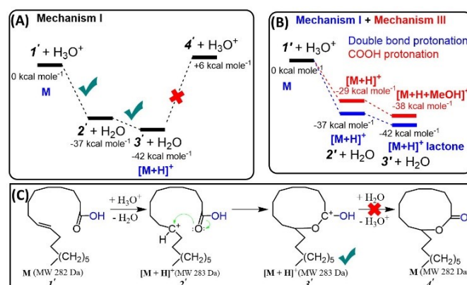
Figure 5 (A) Free energy diagram of gas-phase intramolecular cyclization of oleic acid. (B) Comparison of DFT calculations for the energetics involved in the protonation of the double bond in oleic acid versus the protonation of the carboxyl group. (C) Scheme showing stepwise mechanism for intramolecular cyclization of unsaturated fatty acids as discovered in this study (Mechanism I). See alternative Mechanism II (lactone formation through hydroxycarboxylic acid) in Supporting Information.
