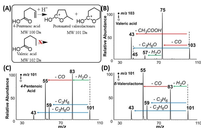
Figure 6 (A) Schematics displaying the intramolecular cyclization of 4-pentenoic acid to give cyclic carbonium ions while valeric acid cannot be cyclized. Positive-ion mode MS/MS spectra of standards of (B) valeric acid, (C) 4-pentenoic acid, and (D) \delta -valerolactone. 4-pentenoic acid converts into 5- and 6-membered cyclic carbonium ions, showing identical MS/MS spectra (C and D).
