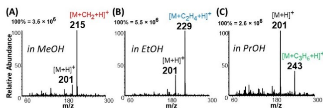
Figure 2 Positive-ion mode spectra for 500 \mu\text{M} lauric acid ( M ), with solution prepared in (A) methanol (MeOH), (B) ethanol (EtOH), and (C) propanol (PrOH). Esterification occurs for all solvents when plasma-nanodroplet fusion is enabled, yielding expected products at m/z 215, m/z 229, and m/z 243, respectively. Conversion rates for methanol, ethanol, and propanol are 85.7%, 75.8%, and 27.2%, respectively. Conversion rate is defined as the ratio of the absolute ion intensity of a specific ester product relative to the sum of intensities of the fatty acid and the ester derived from this acid.
