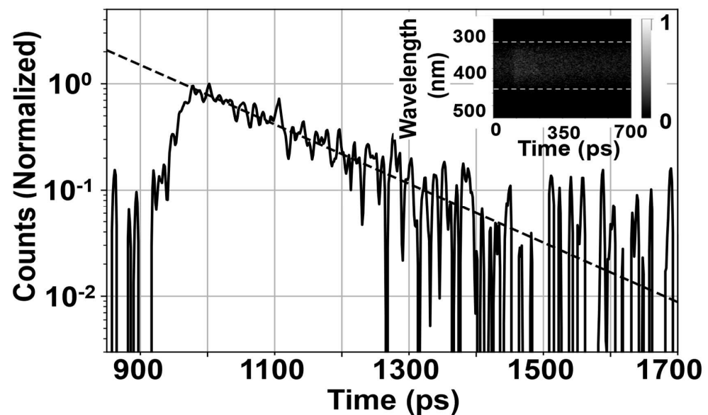
Figure 11. A streak of time-resolved CL, acquired at RT for the reference structure, and its raw image (inset). Reprinted with permission from the AIP. After Ref. [34].
