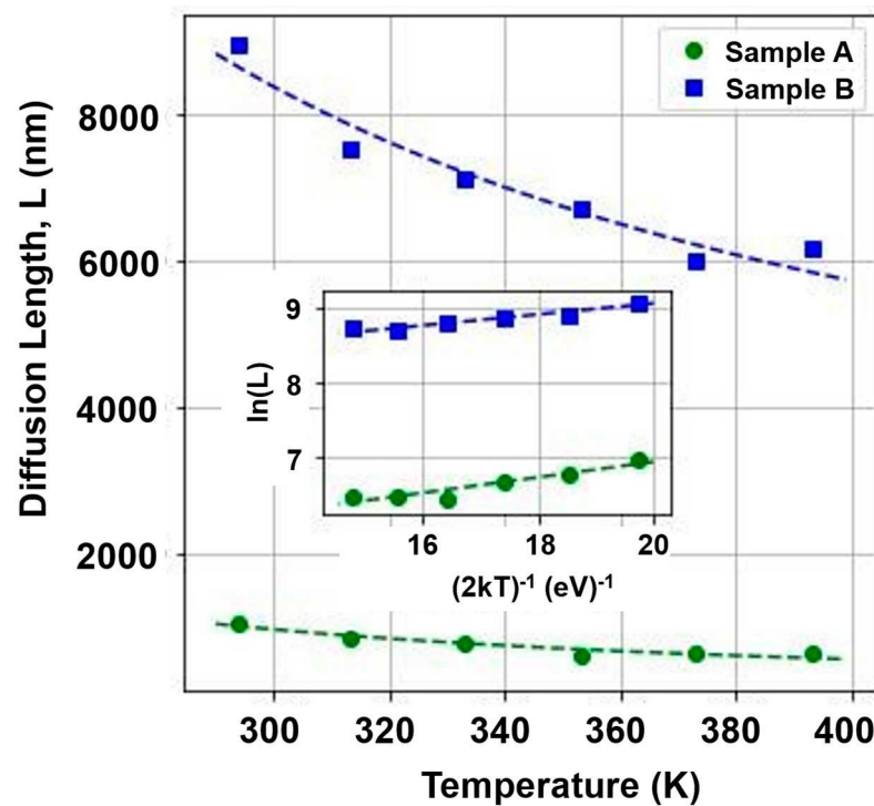
Figure 3. Dependence of the diffusion length on temperature for highly resistive p-type samples. Inset: Arrhenius plot and the fit for \Delta E_{L,T} . Reprinted with permission from the AIP. After Ref. [36].
