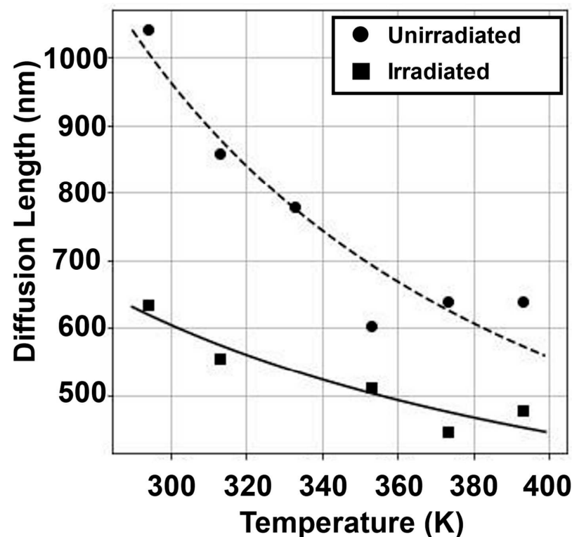
Figure 13. L vs. T dependence prior to and following bombardment with high-energy protons with the following energy/dose sequence: 25 keV, 1.6 \times 10^{14} \text{ cm}^{-2} + 50 keV, 1.7 \times 10^{14} \text{ cm}^{-2} + 70 keV, 3.6 \times 10^{14} \text{ cm}^{-2} . Reprinted with permission from the AIP. After Refs. [27,36].
