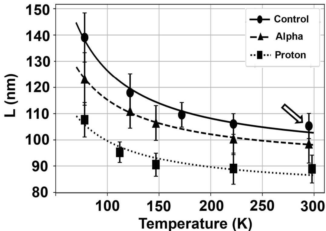
Figure 10. Temperature dependence of L for various radiation types. The arrow shows the RT values. Reprinted with permission from the AIP. After Ref. [34].
