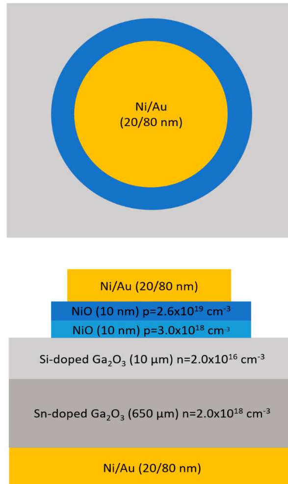
Figure 19. Architecture of the vertical p-NiO/n- \text{Ga}_2\text{O}_3 heterojunction structure (top and front view). The top Ni/Au contact is 1000 \mu\text{m} in diameter. The structure was provided by the group of Profs. S. J. Pearton and Fan Ren of the University of Florida.
