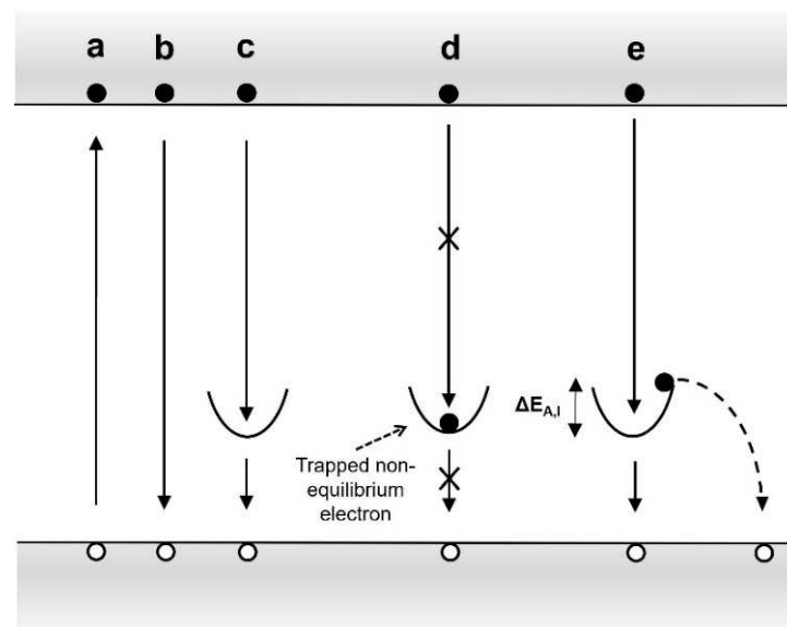
Figure 18. Model for the electron-injection-induced effect (for the example of electron beam irradiation, which generates non-equilibrium electron–hole pairs). Reprinted with permission from the American Institute of Physics. After Ref. [45].
