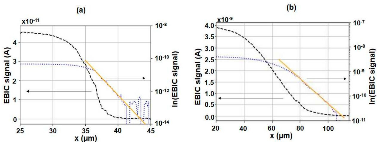
Figure 2. Raw data for the structure A (a) and the structure B (b) at RT, and the fit for the extraction of the diffusion length. Reprinted with permission from the AIP. After Ref. [36].
