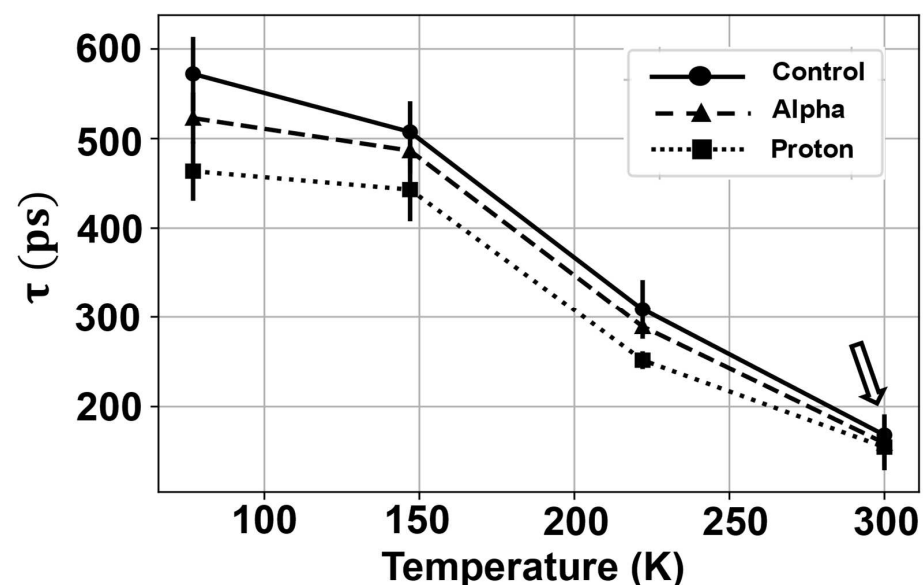
Figure 12. Lifetime vs. temperature dependence for structures irradiated by various particles. The arrow shows the RT value. Reprinted with permission from the AIP. After Ref. [34].
