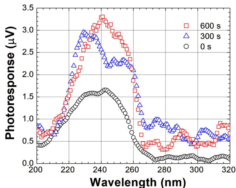
Figure 21. Spectral photoresponse of the structure in Figure 19 before and after incremental charge injection. The charge, corresponding to 600 s of injection, is 60 mC. The effect persists for at least several hours.
