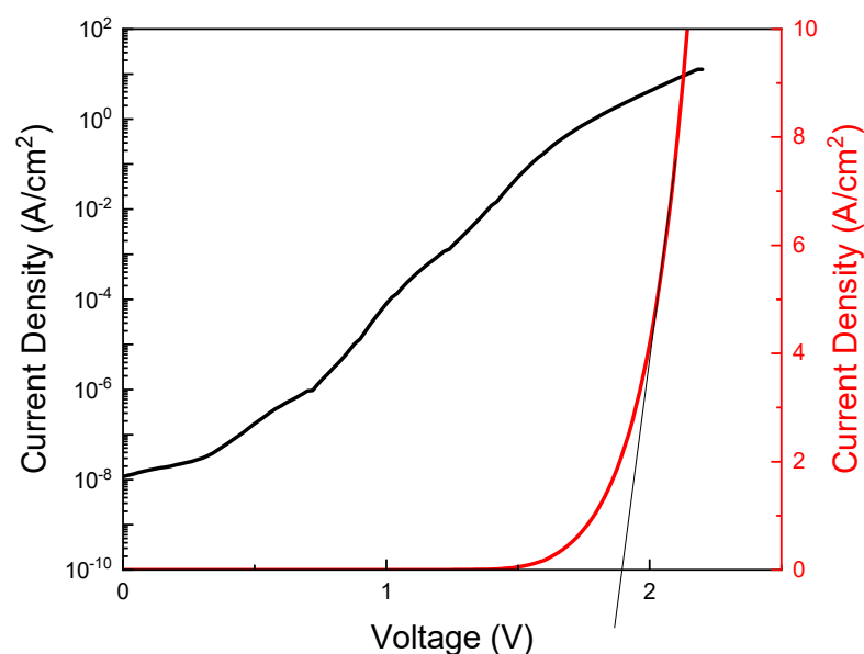
Figure 20. Forward branch of the I-V curve for the p-NiO/n- \text{Ga}_2\text{O}_3 heterojunction in linear and logarithmic scales. The turn-on voltage value, obtained by the intersection of the tangential line to the I-V curve with the horizontal axis, is \sim 1.9 \text{ V} .
