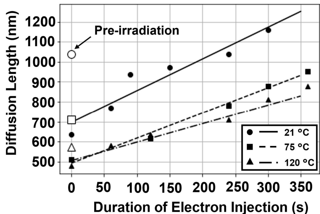
Figure 14. L vs. duration of electron injection dependence at variable temperatures for highly resistive \text{p-Ga}_2\text{O}_3 . The L values for 0 injected charge are shown in an open circle (21 °C), square (75 °C), and triangle (120 °C). \Delta E_{A,L} , obtained from the dependence of L on the injection duration at varying T , is estimated at 91 meV using Equation (6). Reprinted with permission from the AIP. After Ref. [27].
