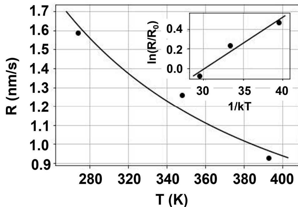
Figure 15. R vs. T dependence. Inset: Arrhenius plot of Equation (6) for the calculation of \Delta E_{A,I} . Reprinted with permission from the AIP. After Ref. [27].
