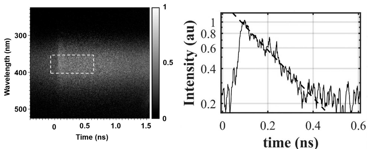
Figure 4. (Left): Time-resolved CL image from a streak camera with a center wavelength of 380 nm. The dashed rectangle shows the region for time decay determination. (Right): Normalized spectrum of CL decay at 380 nm with an exponential fit for n-type \beta\text{-Ga}_2\text{O}_3 . The lifetime is obtained from the exponential fit inverse slope for the temporal CL decay. Reprinted with permission from the AIP. After Ref. [33].
