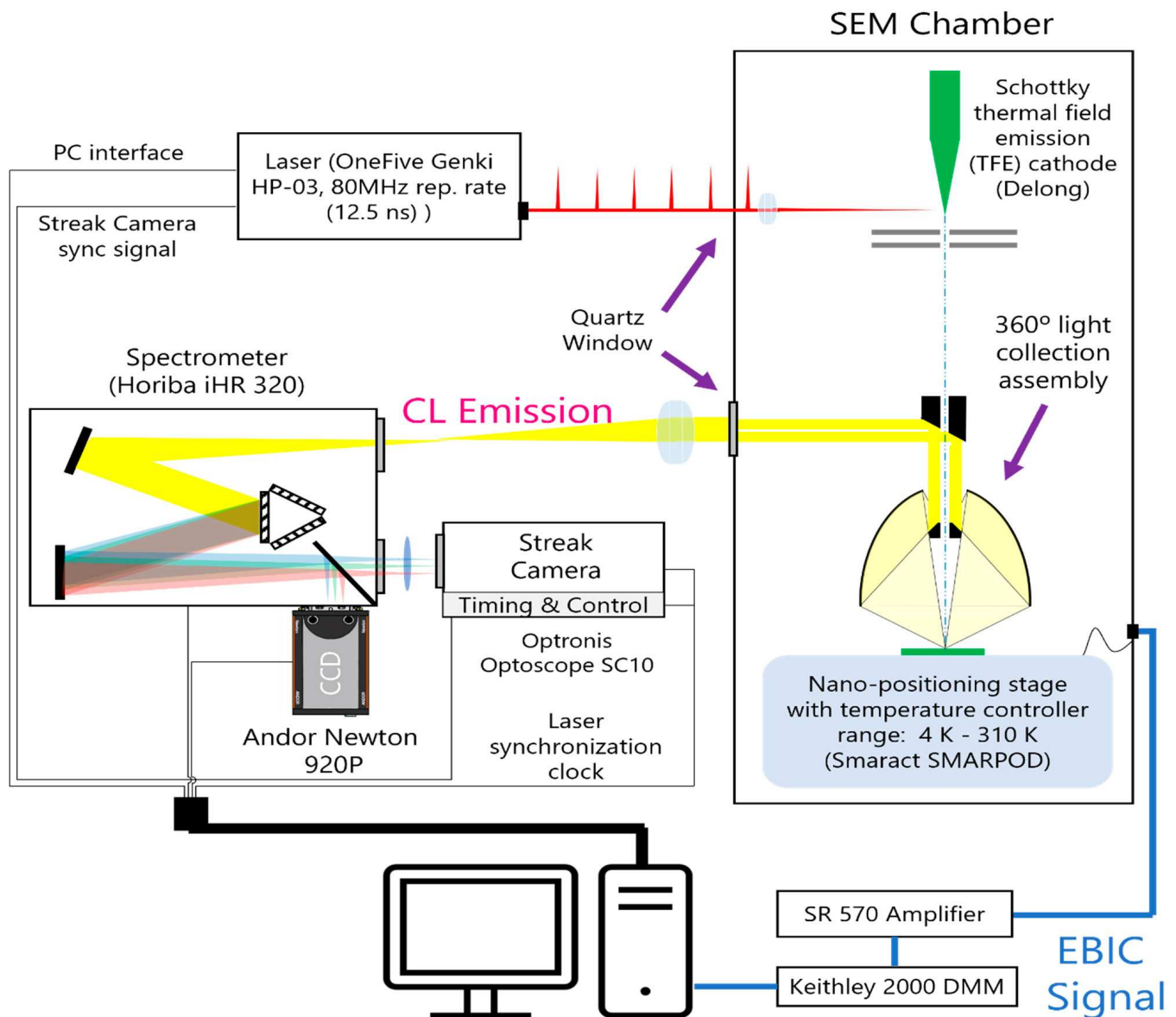
Figure 5. Experimental setup of the Attolight Allallin 4027 Chronos SEM-CL tool capable of sustaining temperatures from 4 K to 310 K.
