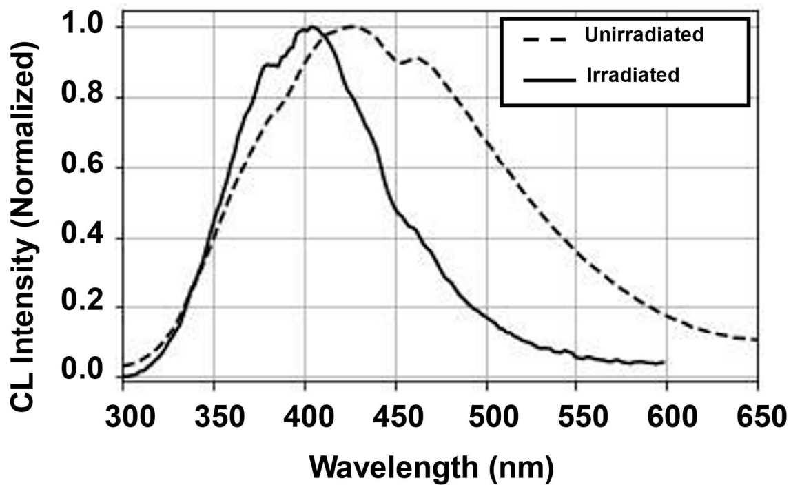
Figure 16. Normalized continuous RT CL spectrum before and after proton irradiation. A blue shift and smaller full-width at half-maximum (FWHM) were observed for the CL spectrum after irradiation. Reprinted with permission from the AIP. After Ref. [27].
