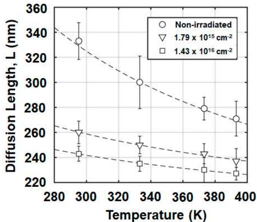
Figure 7. Dependence of L on T for irradiated and reference samples with fits, revealing the activation energy, \Delta E_{L,T} . Reprinted with permission from the AIP. After Refs. [32,33].
