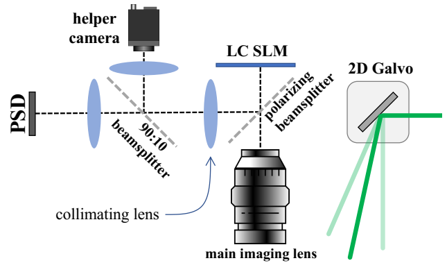
Figure 6: Optical schematic. The main imaging lens focuses the scene onto the SLM. The PSD images the masked scene on the SLM. A helper camera views the scene for calibration and ground truth depth experiments.
